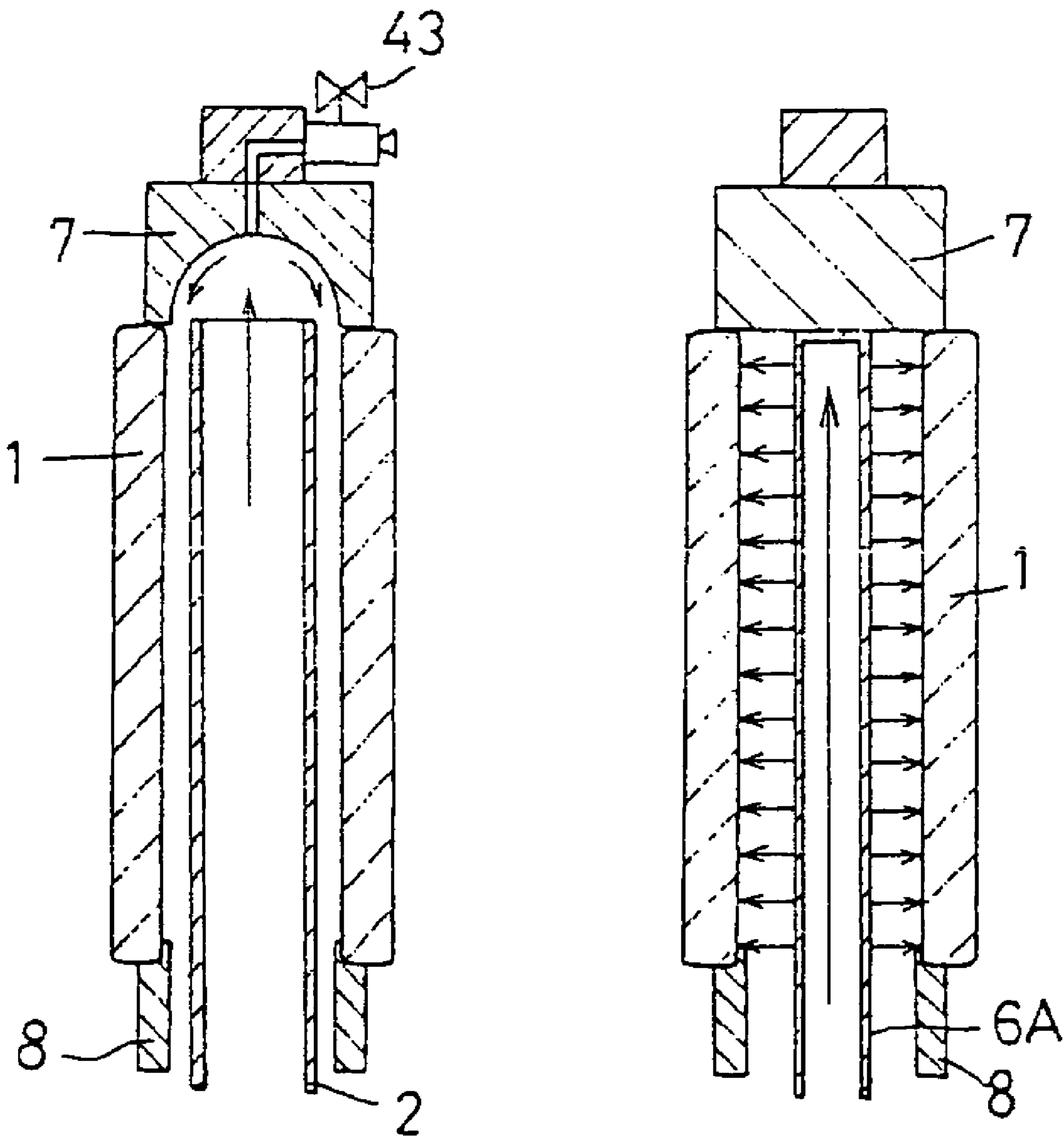
(b) SPRAY COOLING
