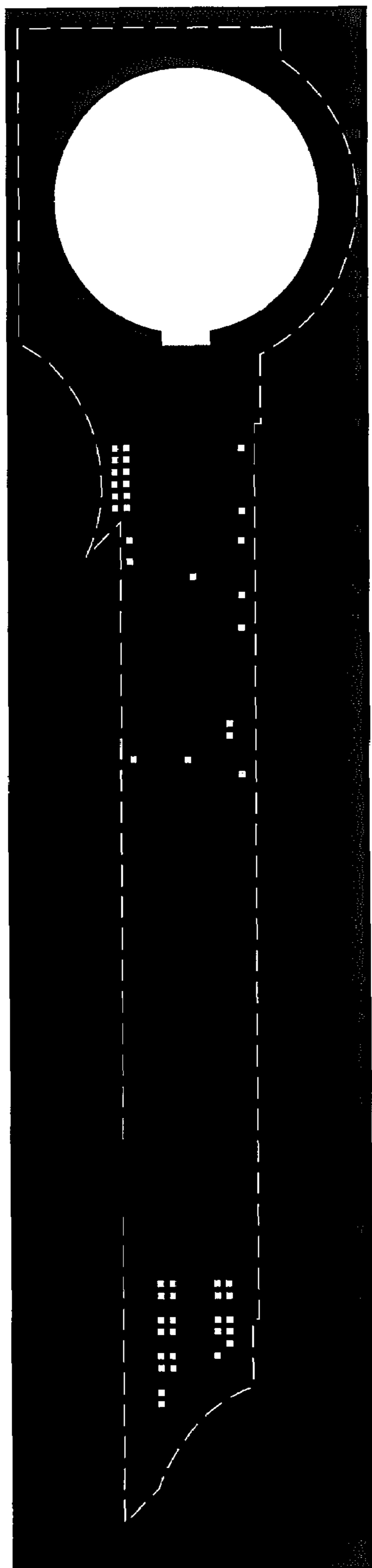
Via 1 mask
