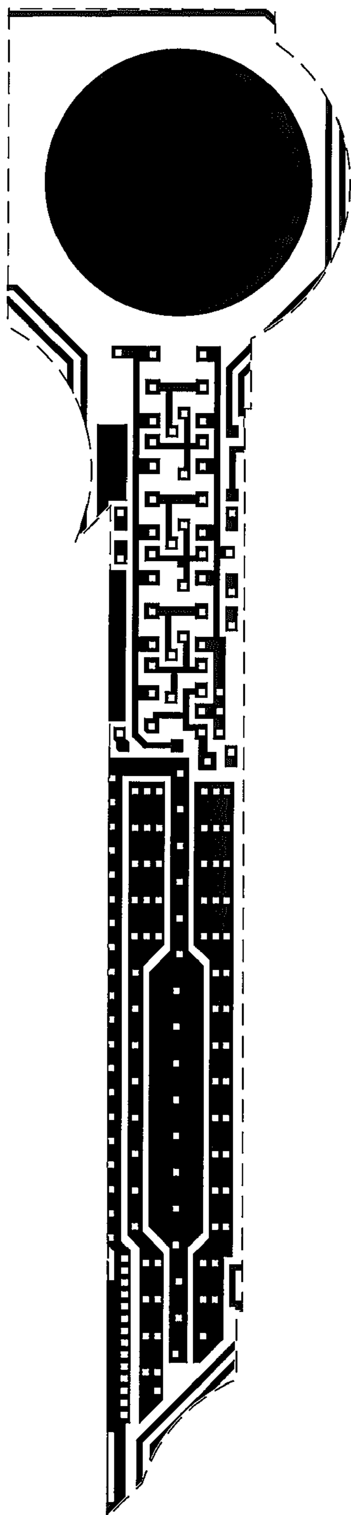
Metal 1 mask
