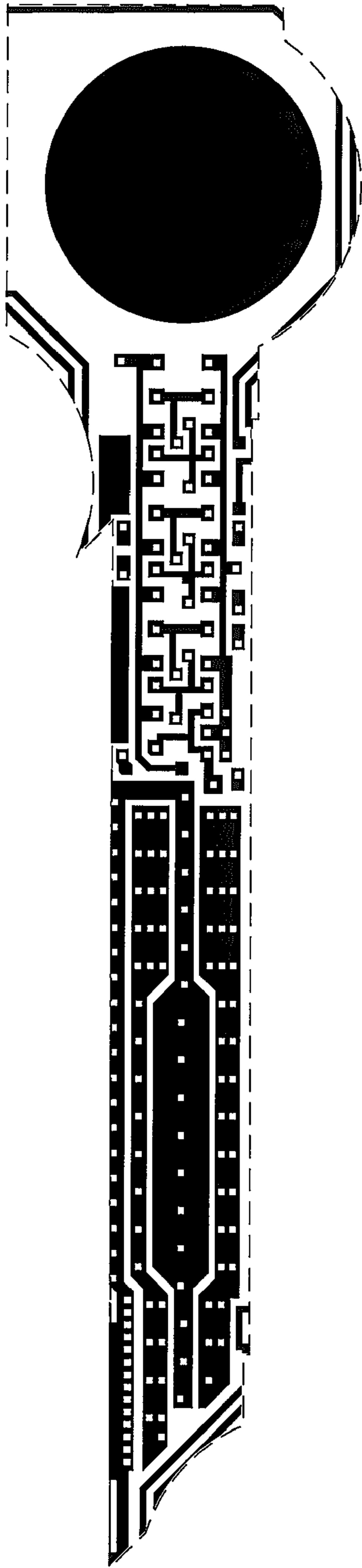
Metal 1 mask
