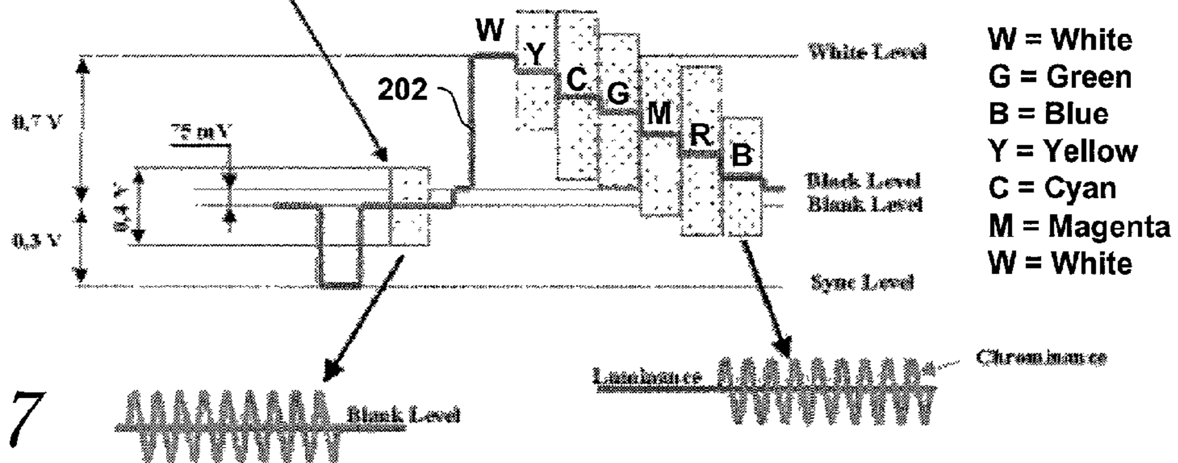
Chrominance burst
