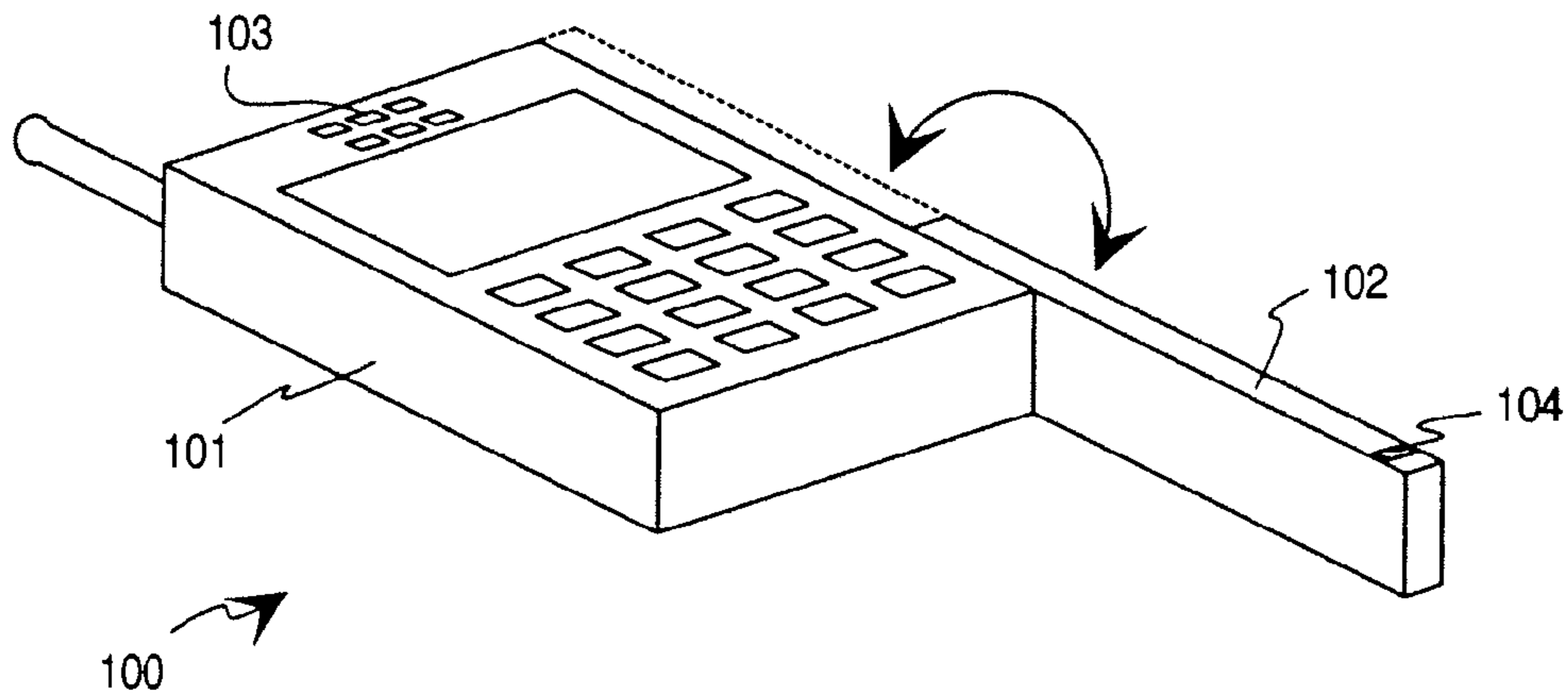
Fig. 1 PRIOR ART
