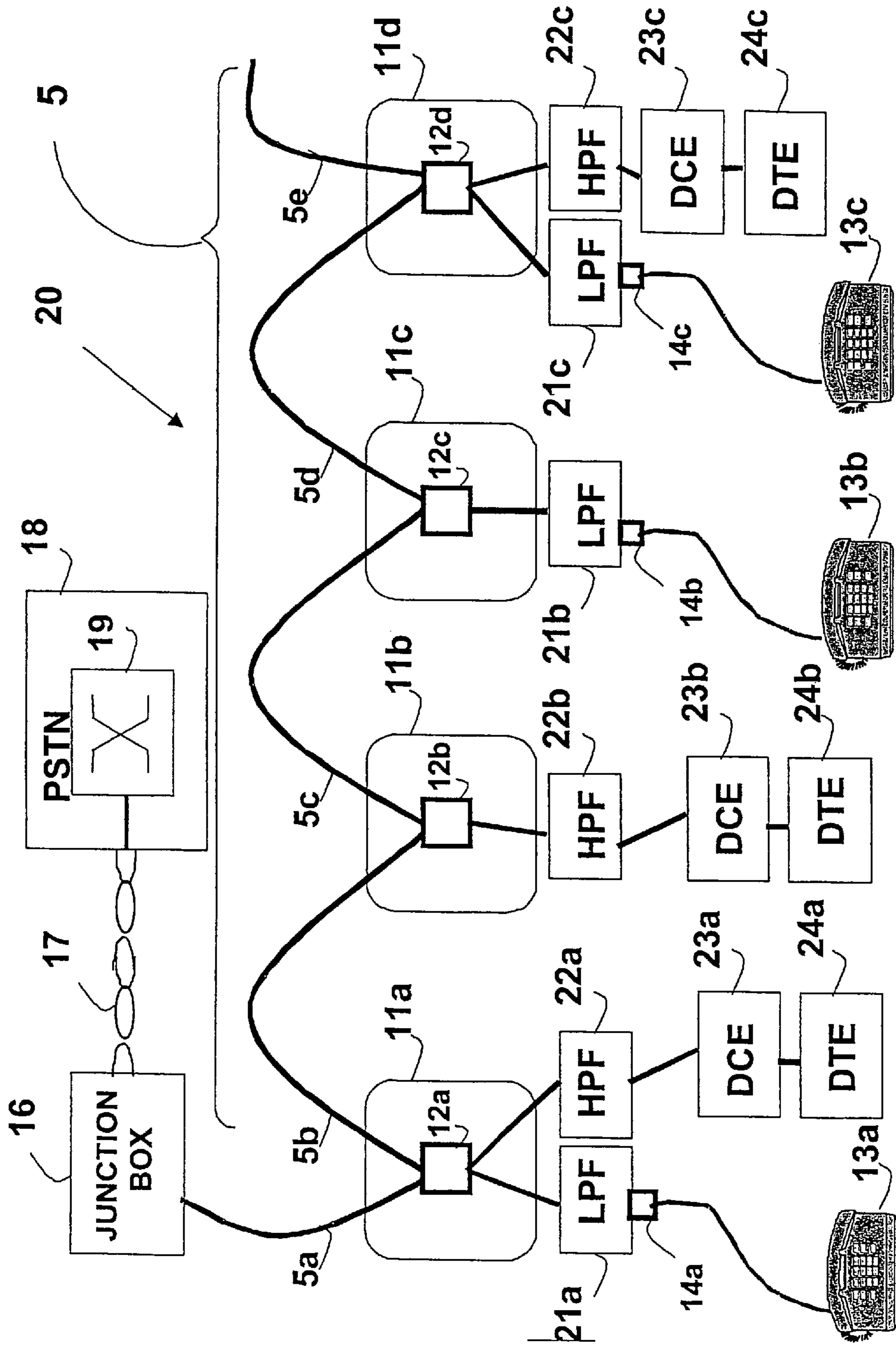
FIGURE 2 (PRIOR-ART)
