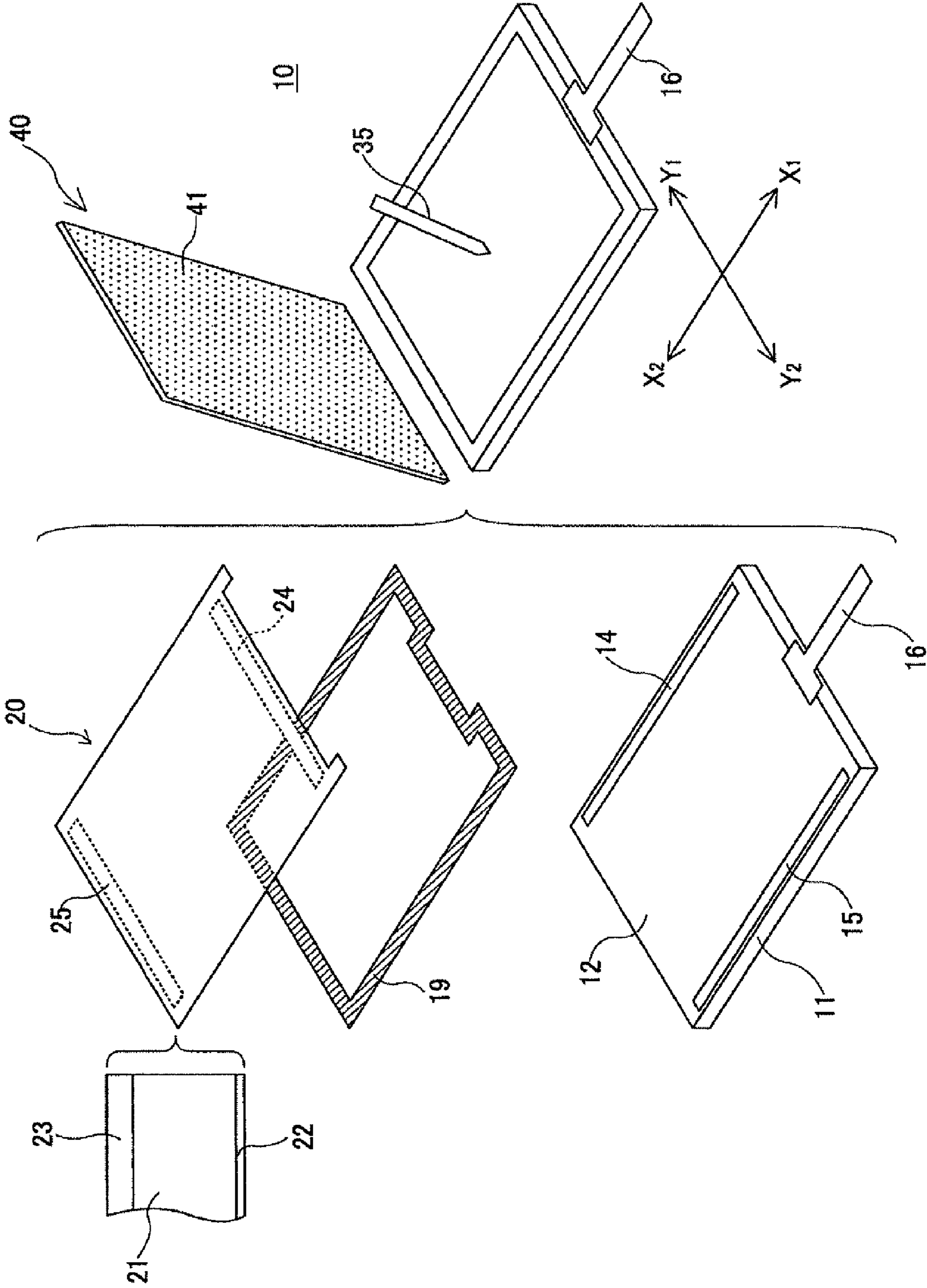
FIG. 1 PRIOR ART
