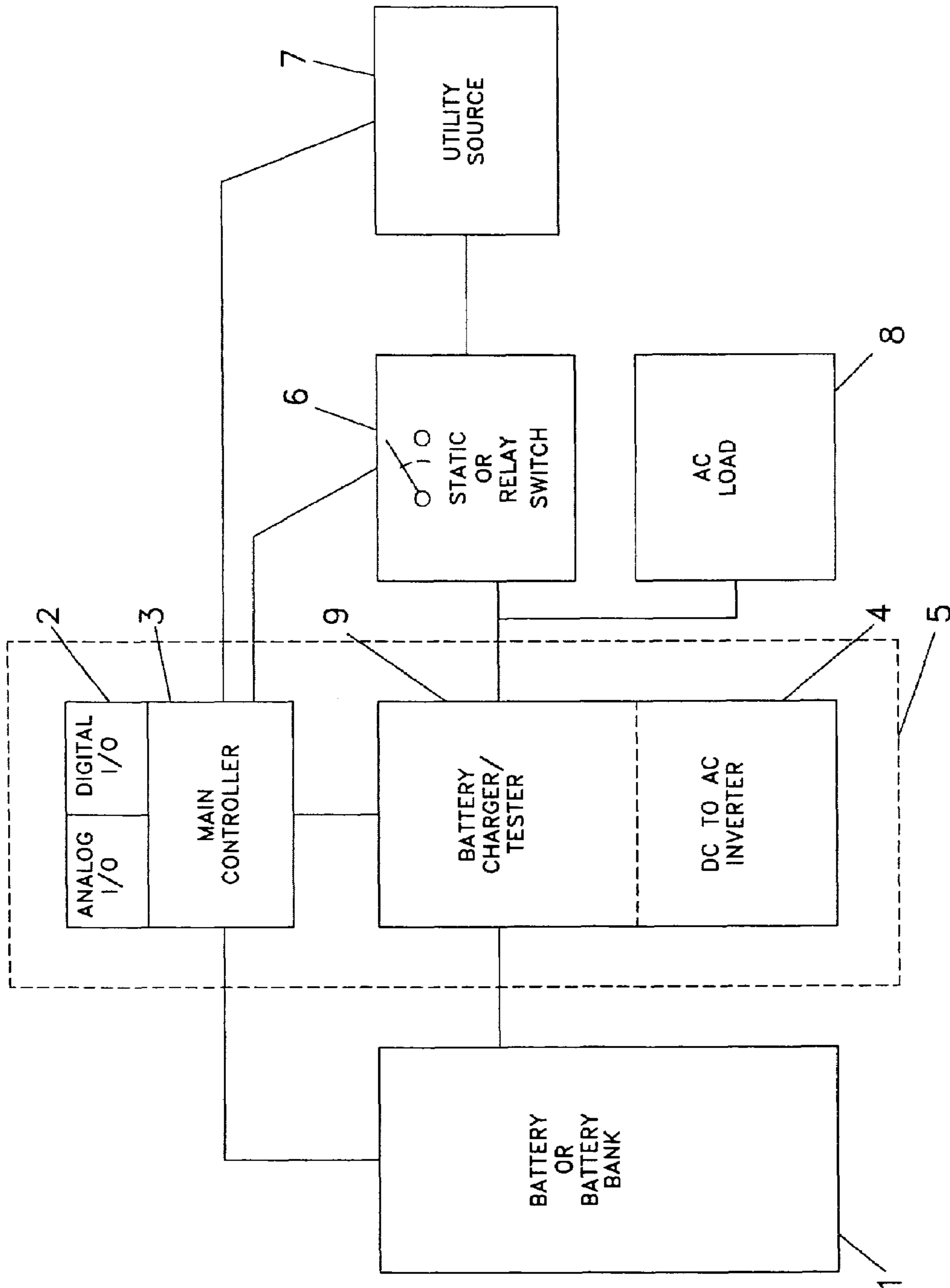
FIGURE 4A OFF LINE UPS TOPOLOGY
