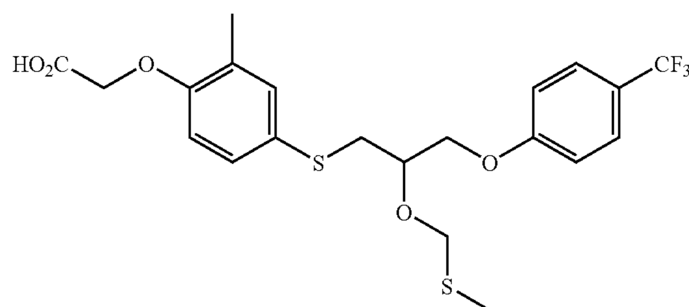
{2-Methyl-4-[2-methylsulfanylmethoxy-3-(4-trifluoromethylphenoxy)-propylsulfanyl]-phenoxy}-acetic acid
