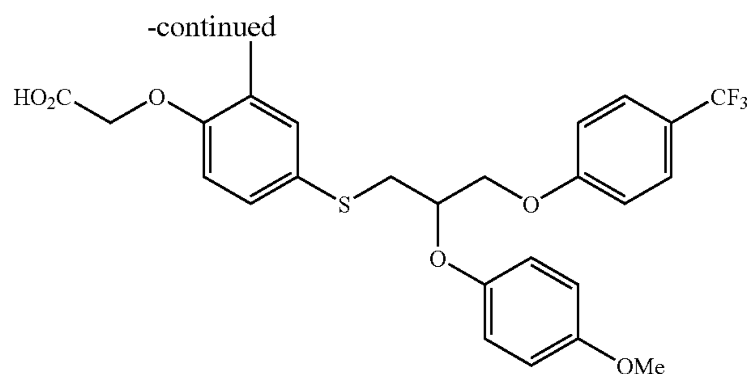
91% Compound 29
