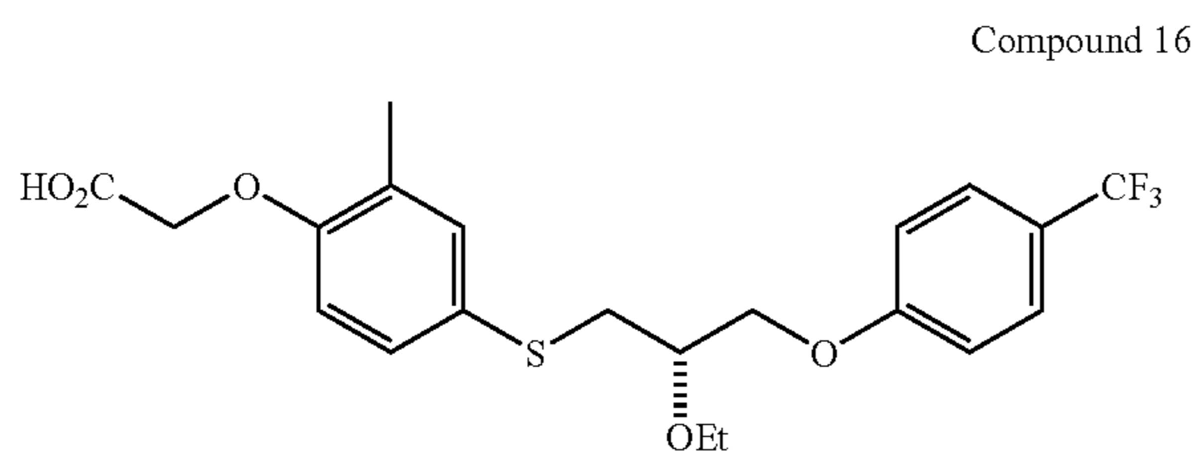
(S)-{4-[2-Ethoxy-3-(4-trifluoromethyl-phenoxy)-propylsulfanyl]-2-methyl-phenoxy}-acetic acid
