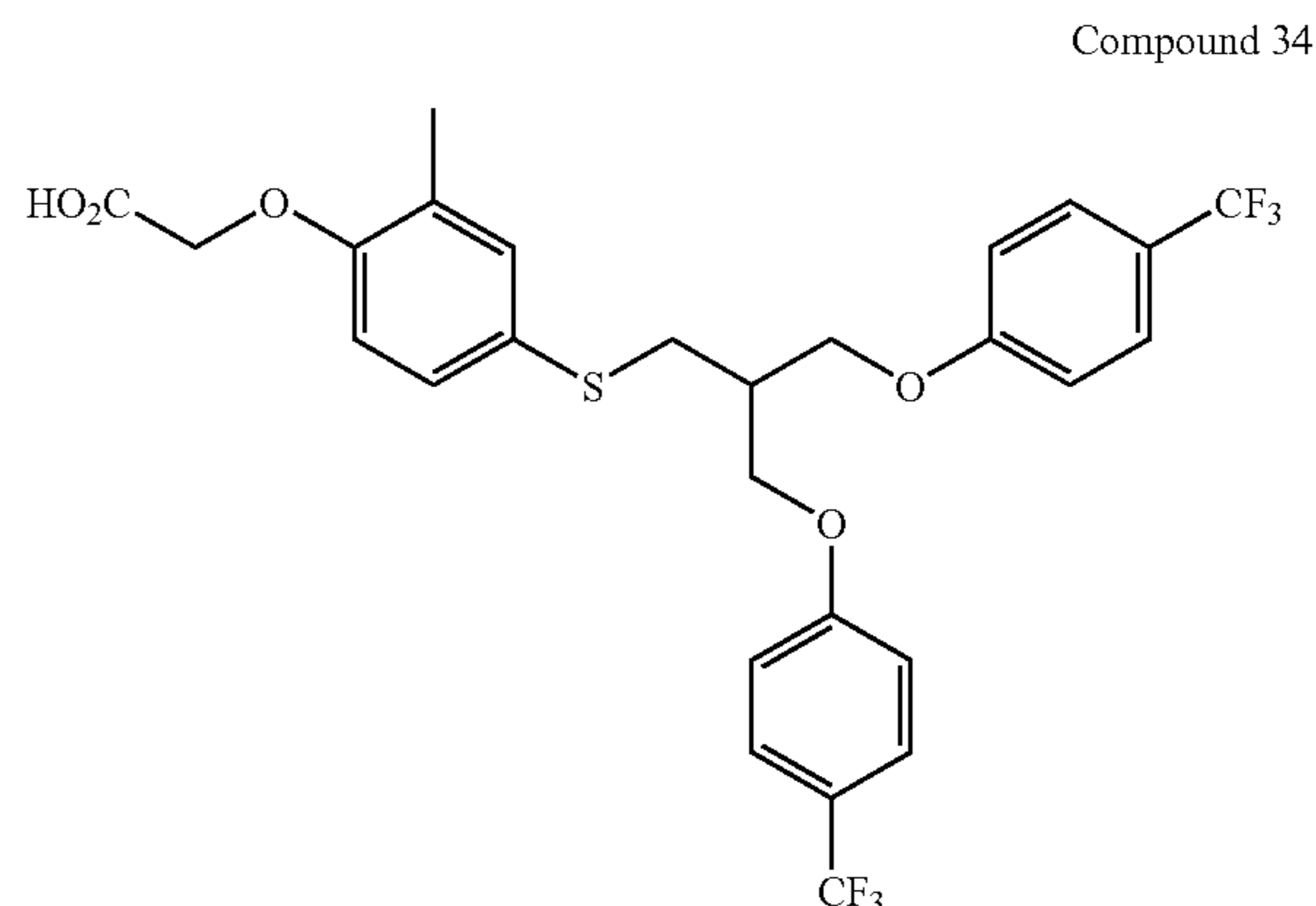
{2-Methyl-4-[3-(4-trifluoromethyl-phenoxy)-2-(4-trifluoromethyl-phoxymethyl)-propylsulfanyl]-phenoxy}-acetic acid
