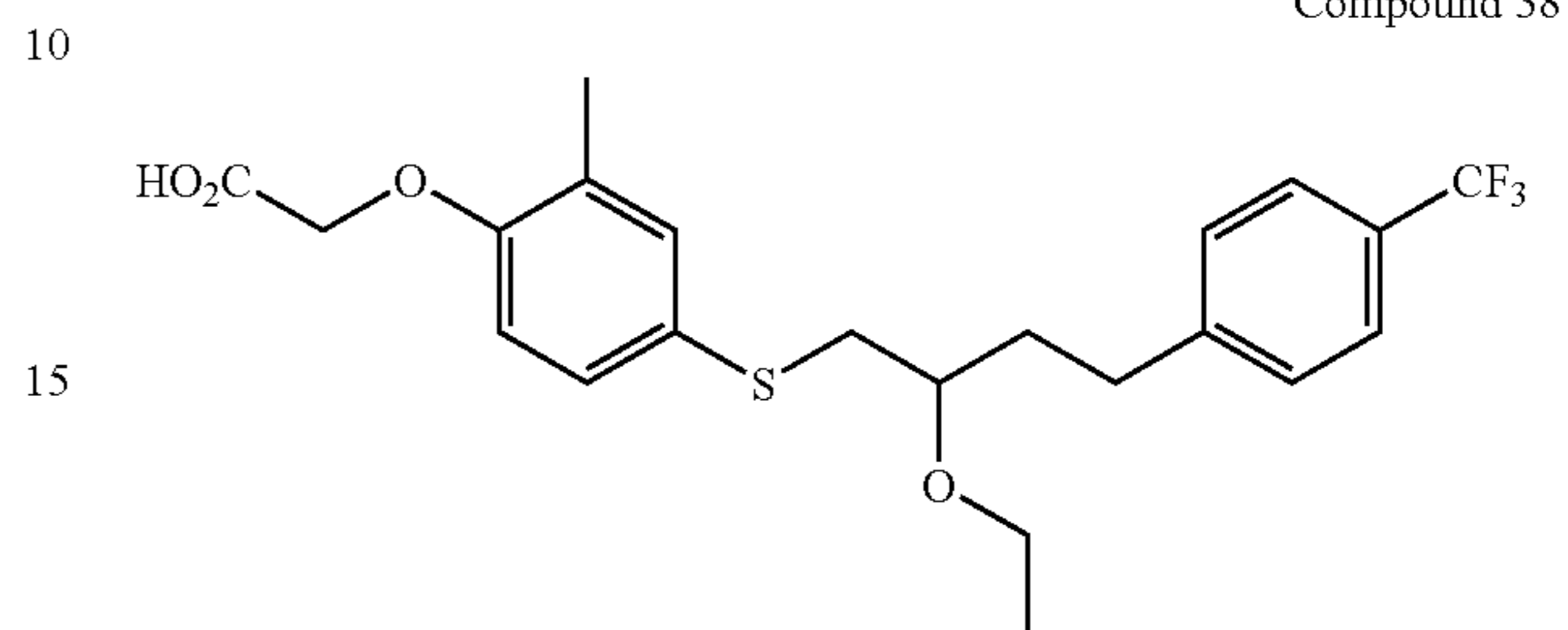
{4-[2-Ethoxy-4-(4-trifluoromethyl-phenyl)-butylsulfanyl]-2-methyl-phenoxy}-acetic acid
