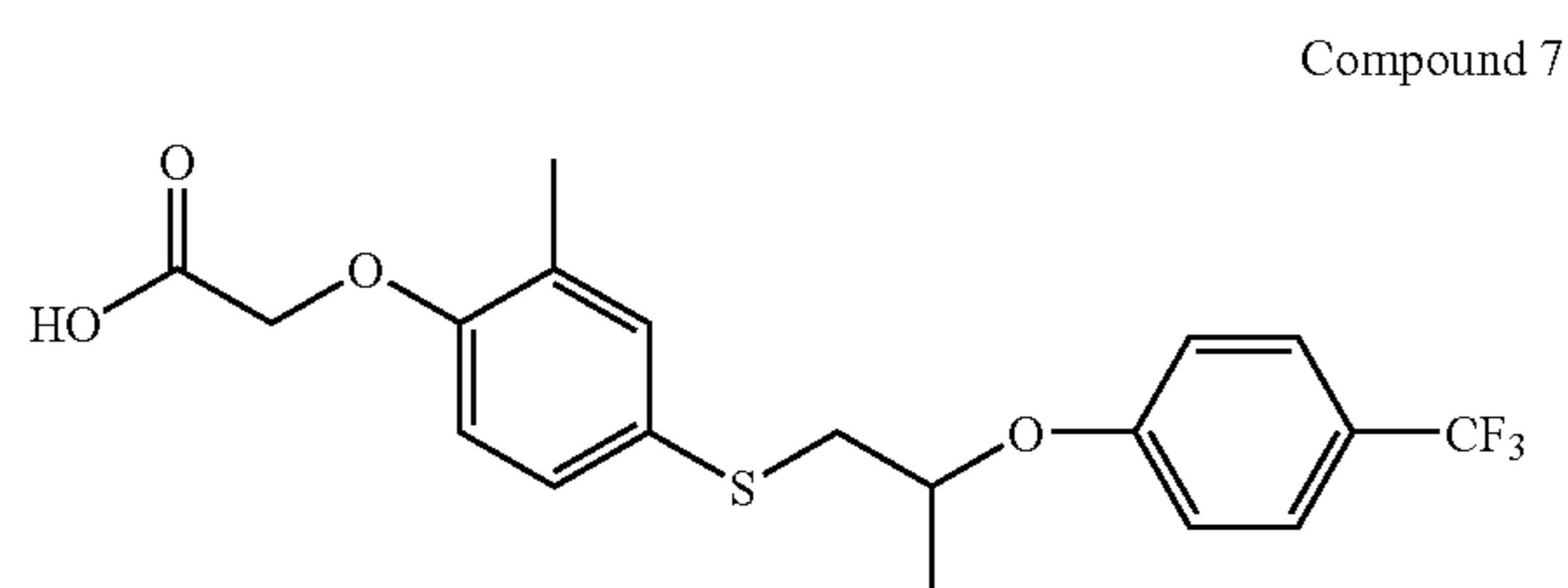
{2-Methyl-4-[2-(4-trifluoromethyl-phenoxy)-propyl-sulfanyl]-phenoxy}-acetic acid
