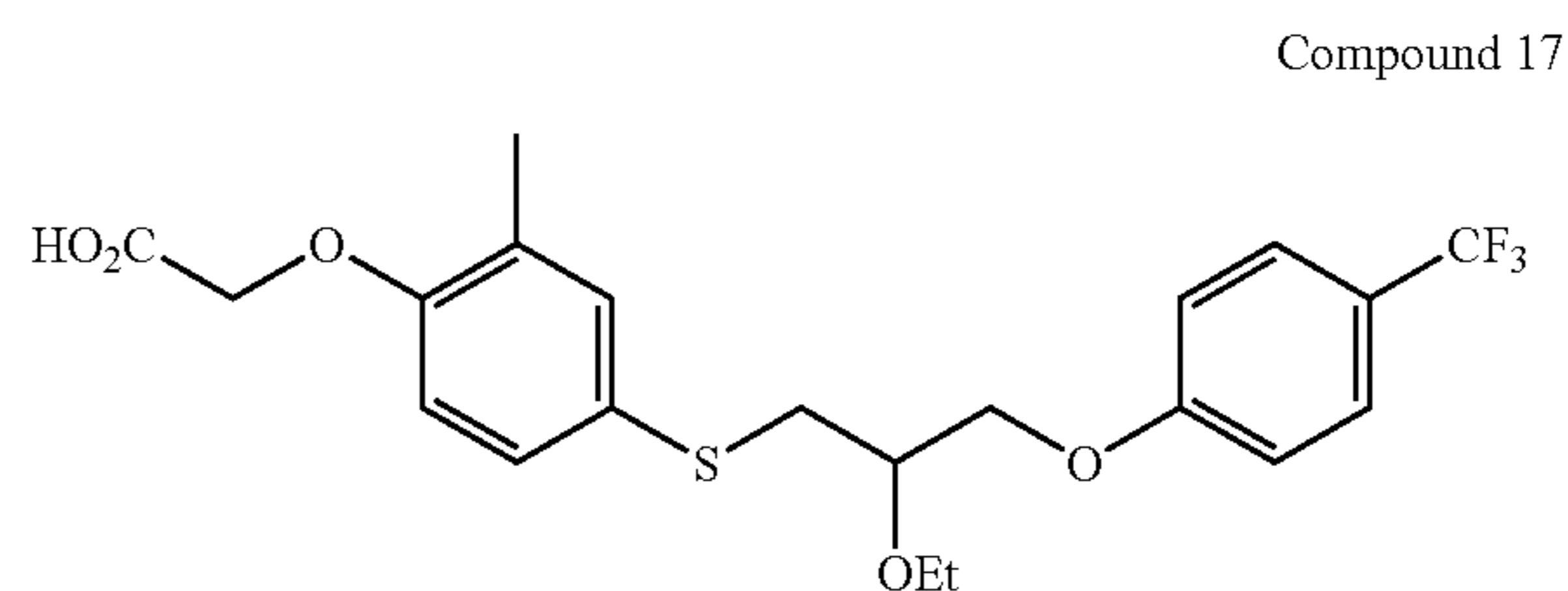
{4-[2-Ethoxy-3-(4-trifluoromethyl-phenoxy)-propylsulfanyl]-2-methyl-phenoxy}-acetic acid
