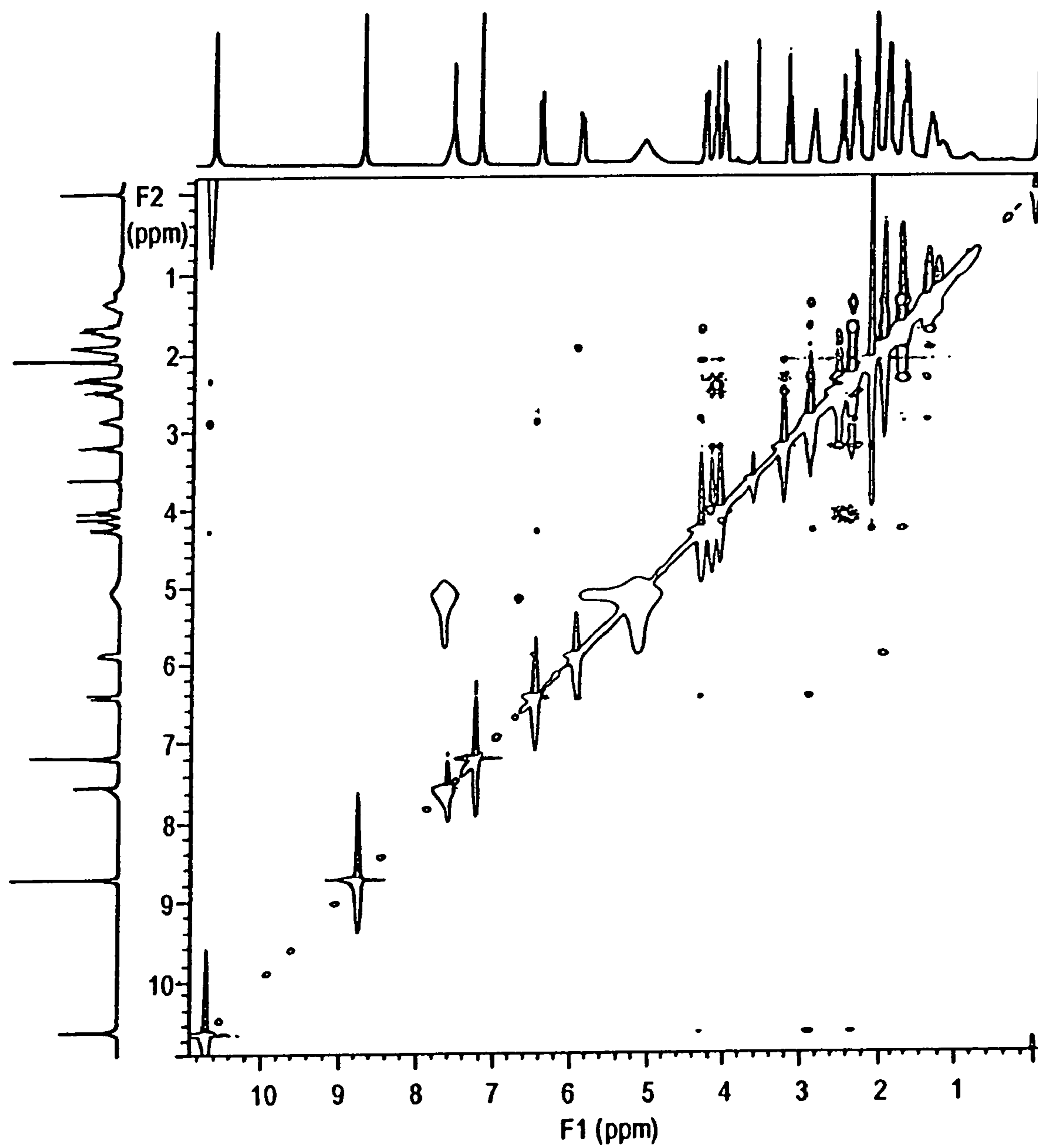
NOESY of salinosporamide A (1), 300 MHz, d 5 -pyridine
