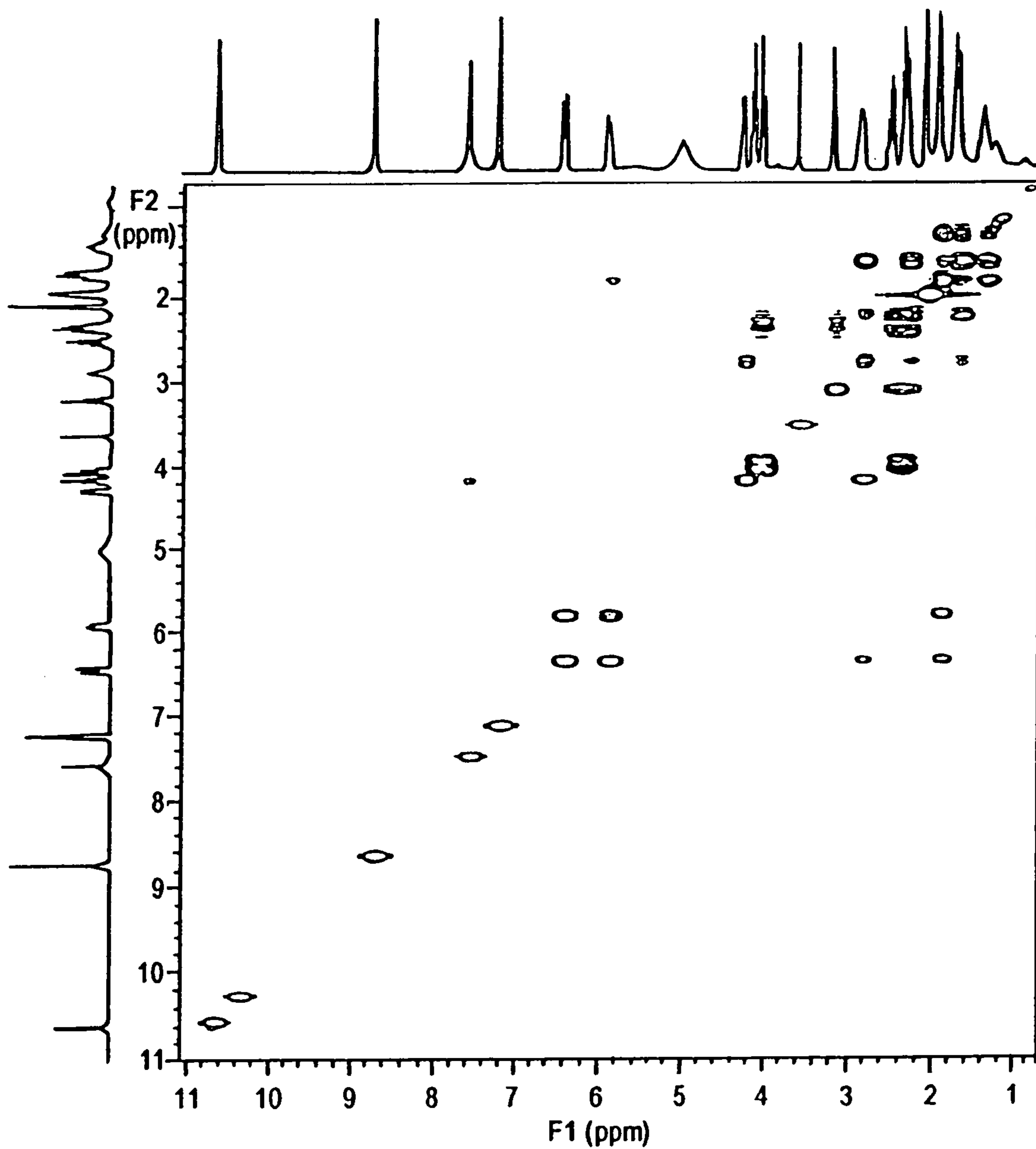
H,H-COSY of salinosporamide A (1), 300 MHz, d 5 -pyridine
