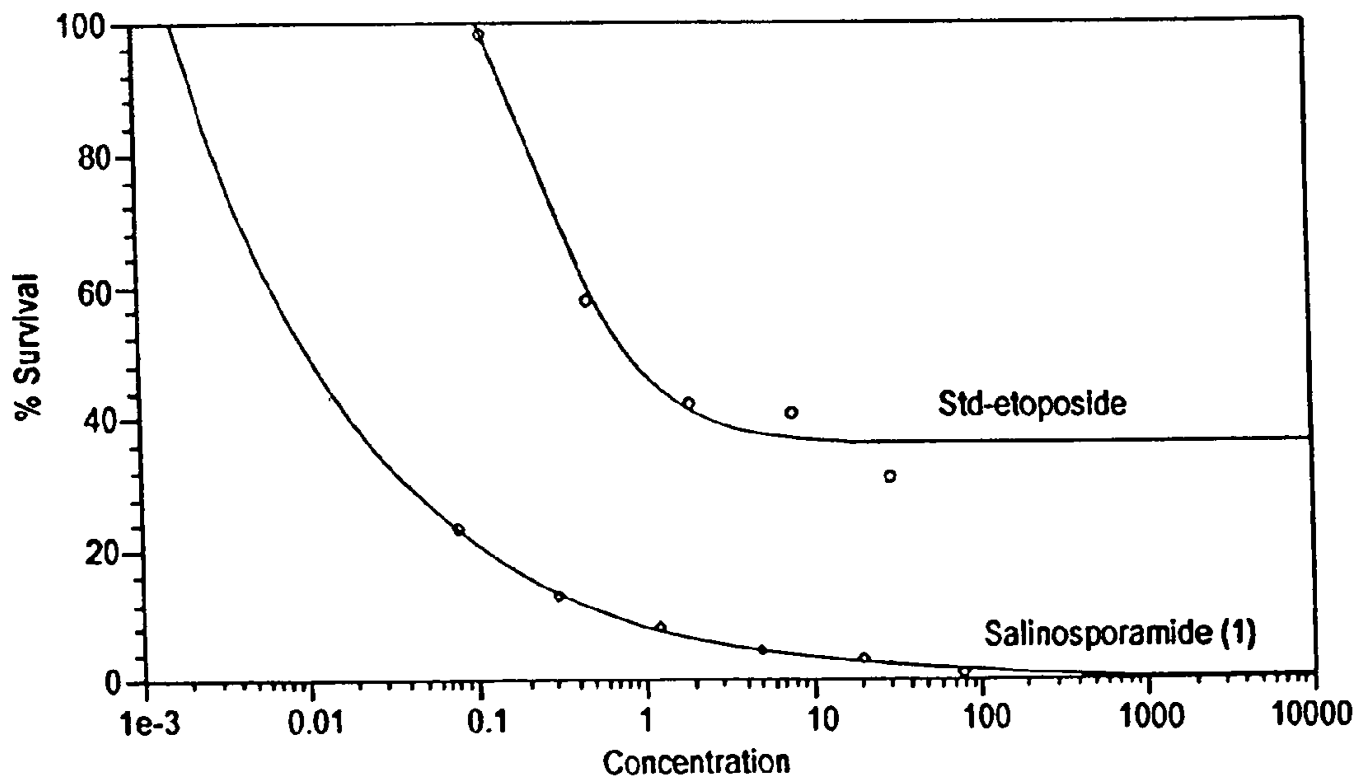
Standard Curve
