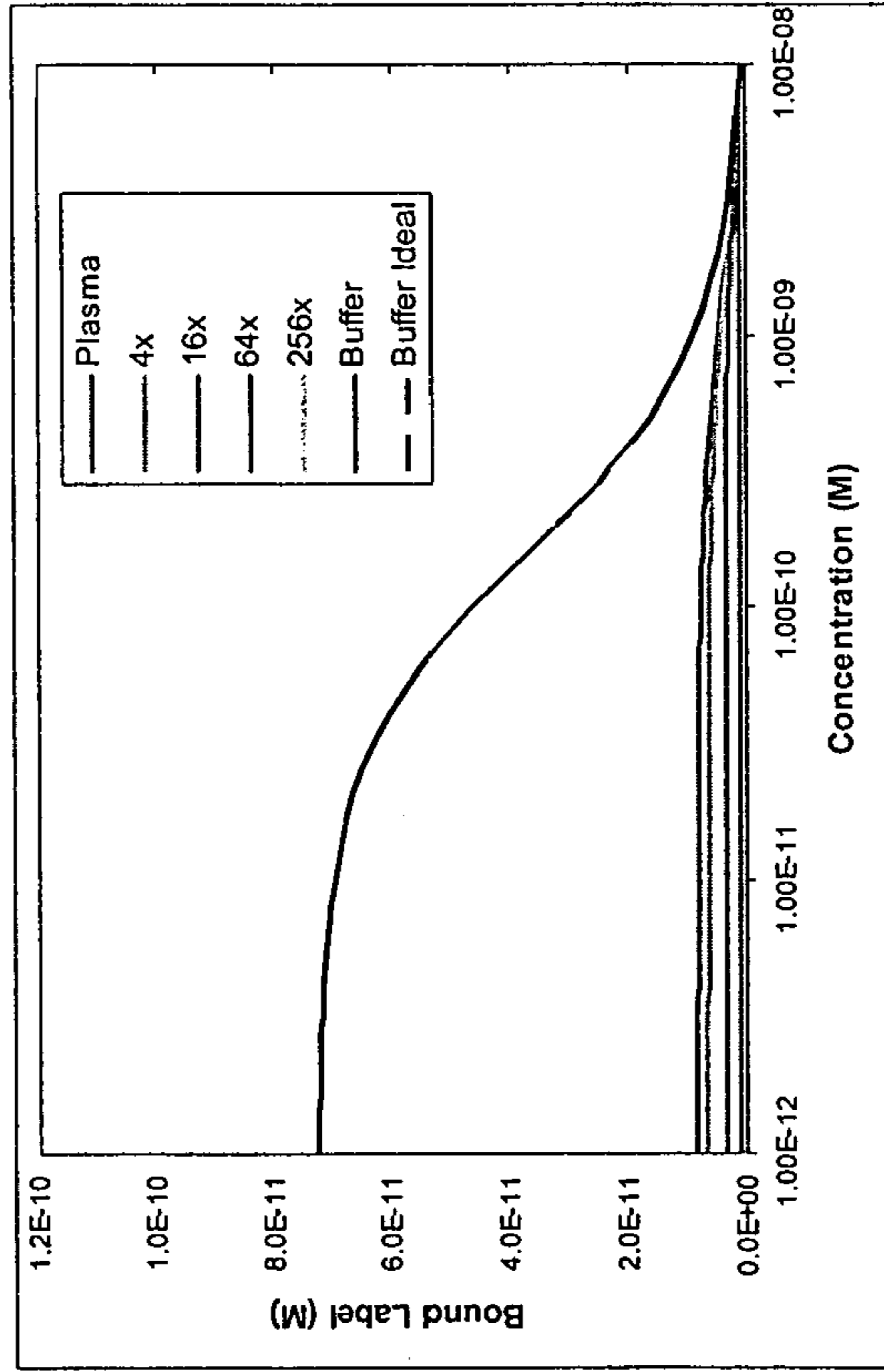
Competitive Binding
