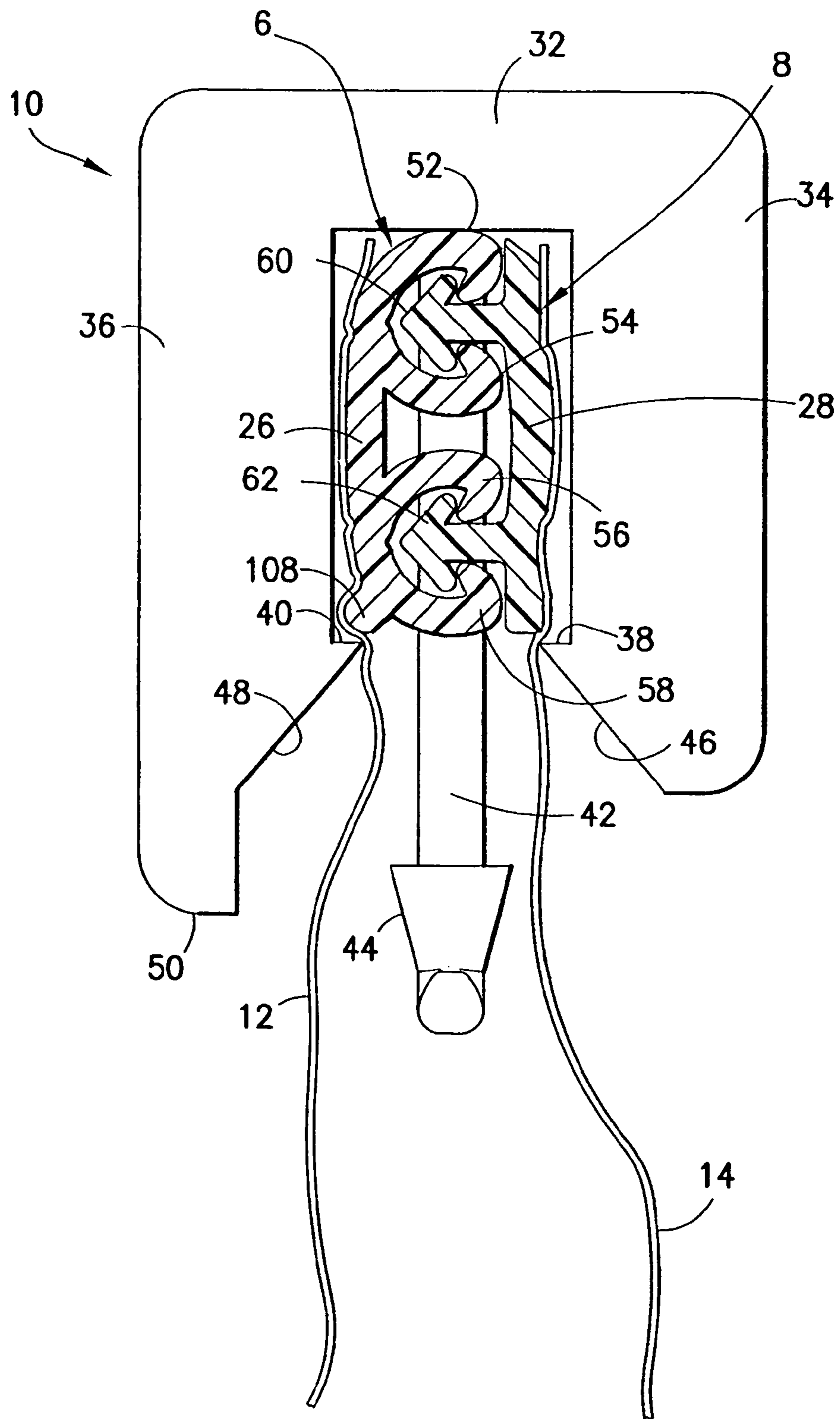
FIG. 2 PRIOR ART
