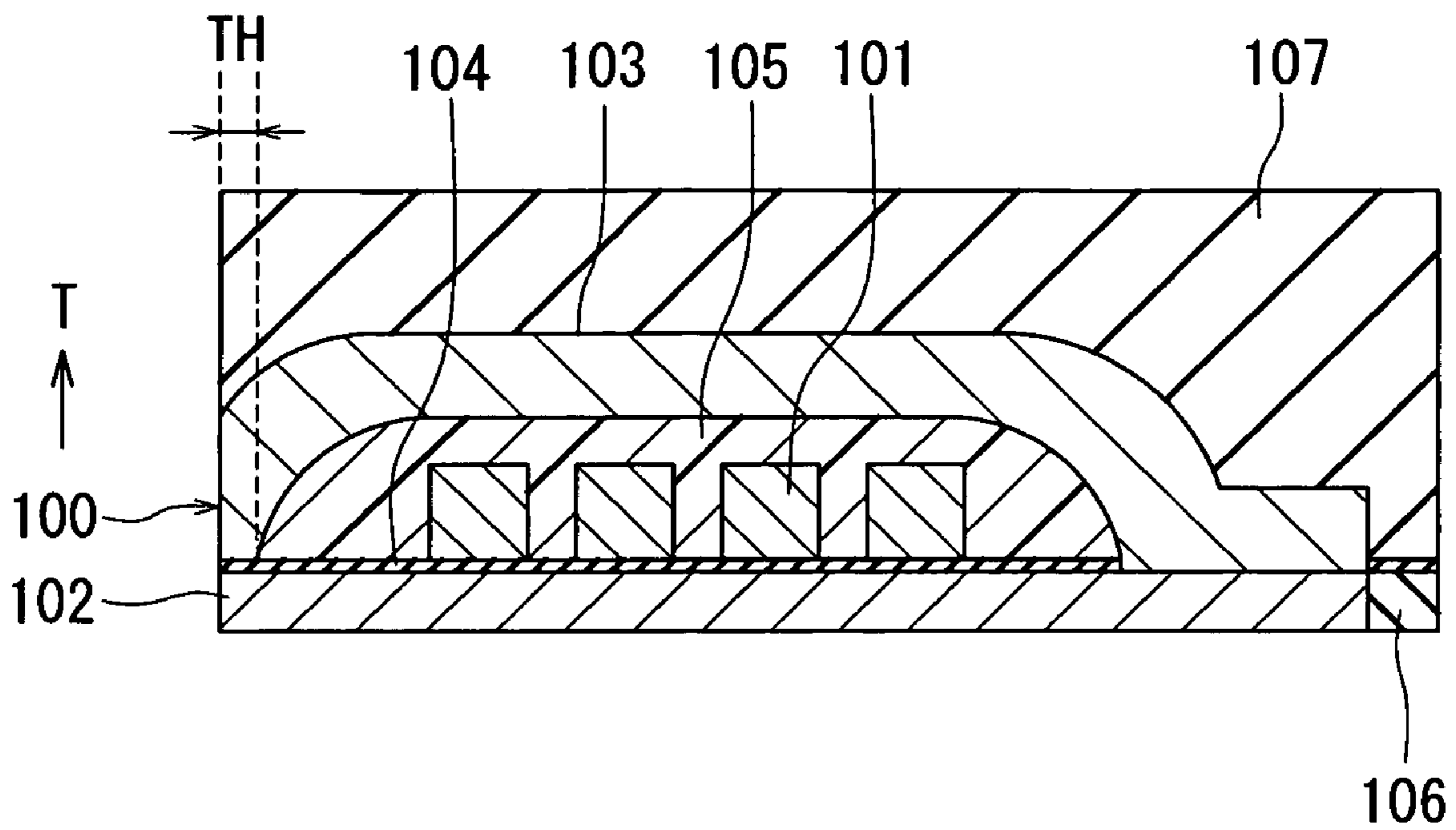
FIG. 44 RELATED ART
