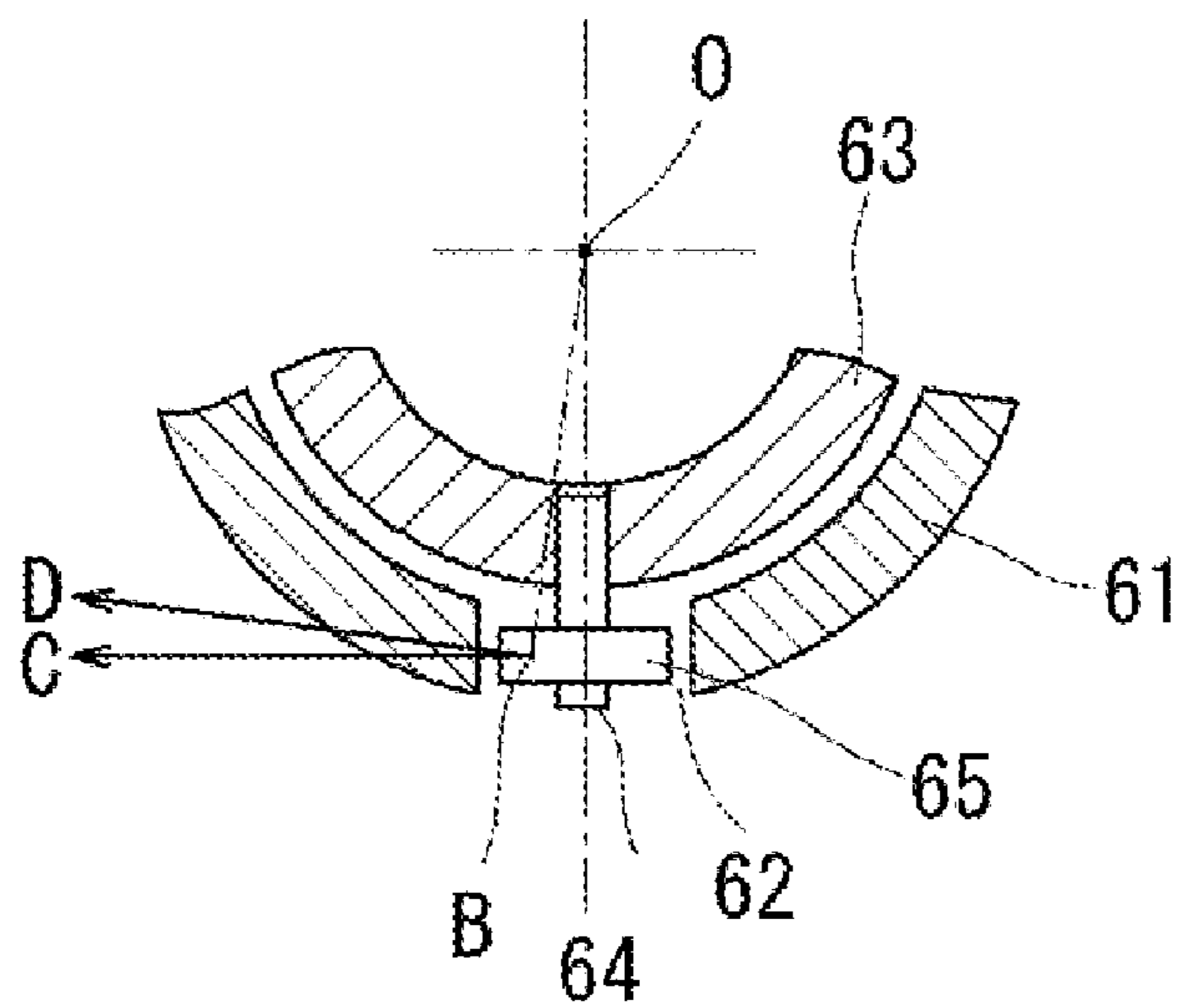
FIG. 10 PRIOR ART
