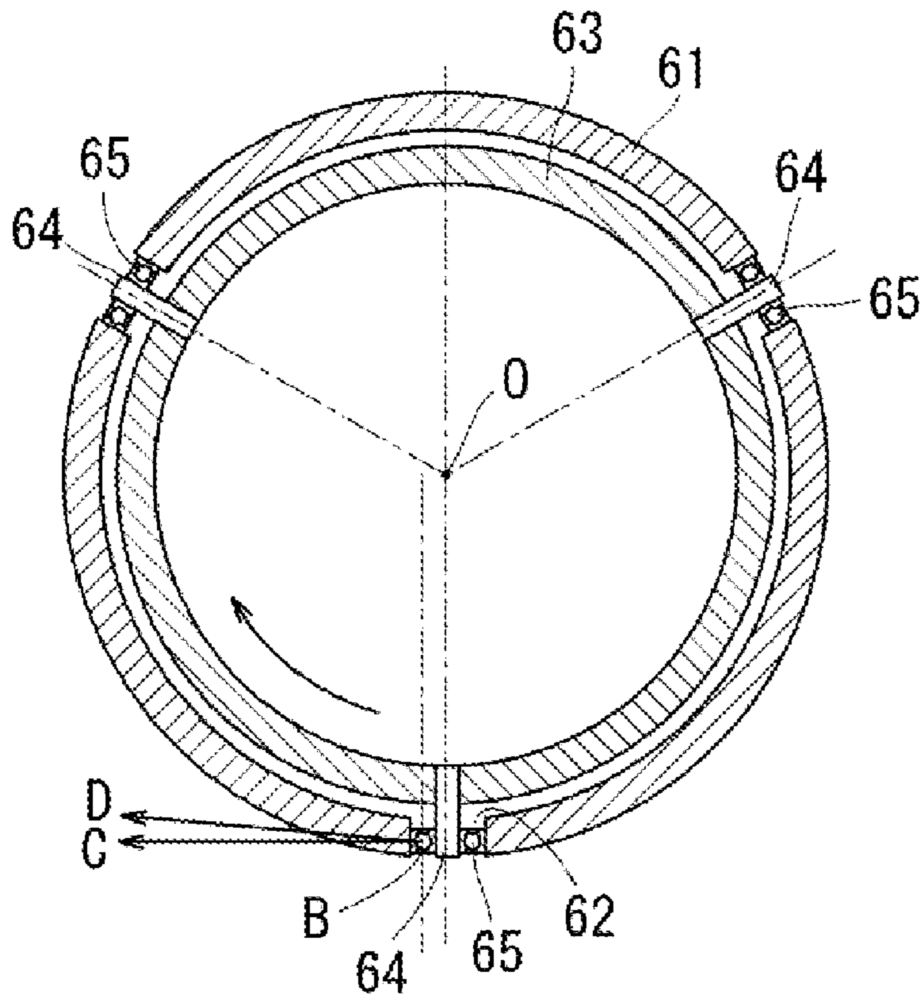
FIG. 9 PRIOR ART
