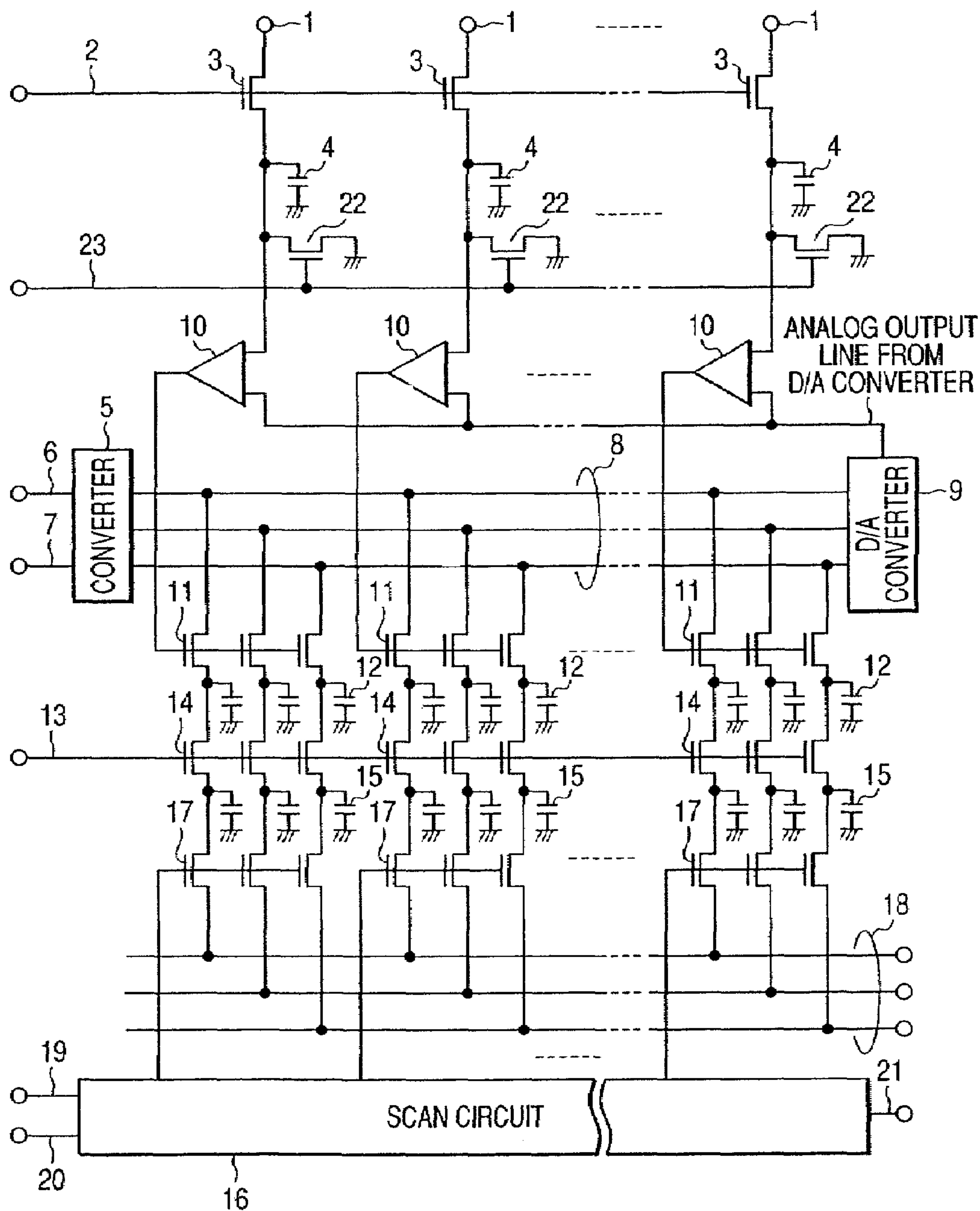
FIG. 22 PRIOR ART
