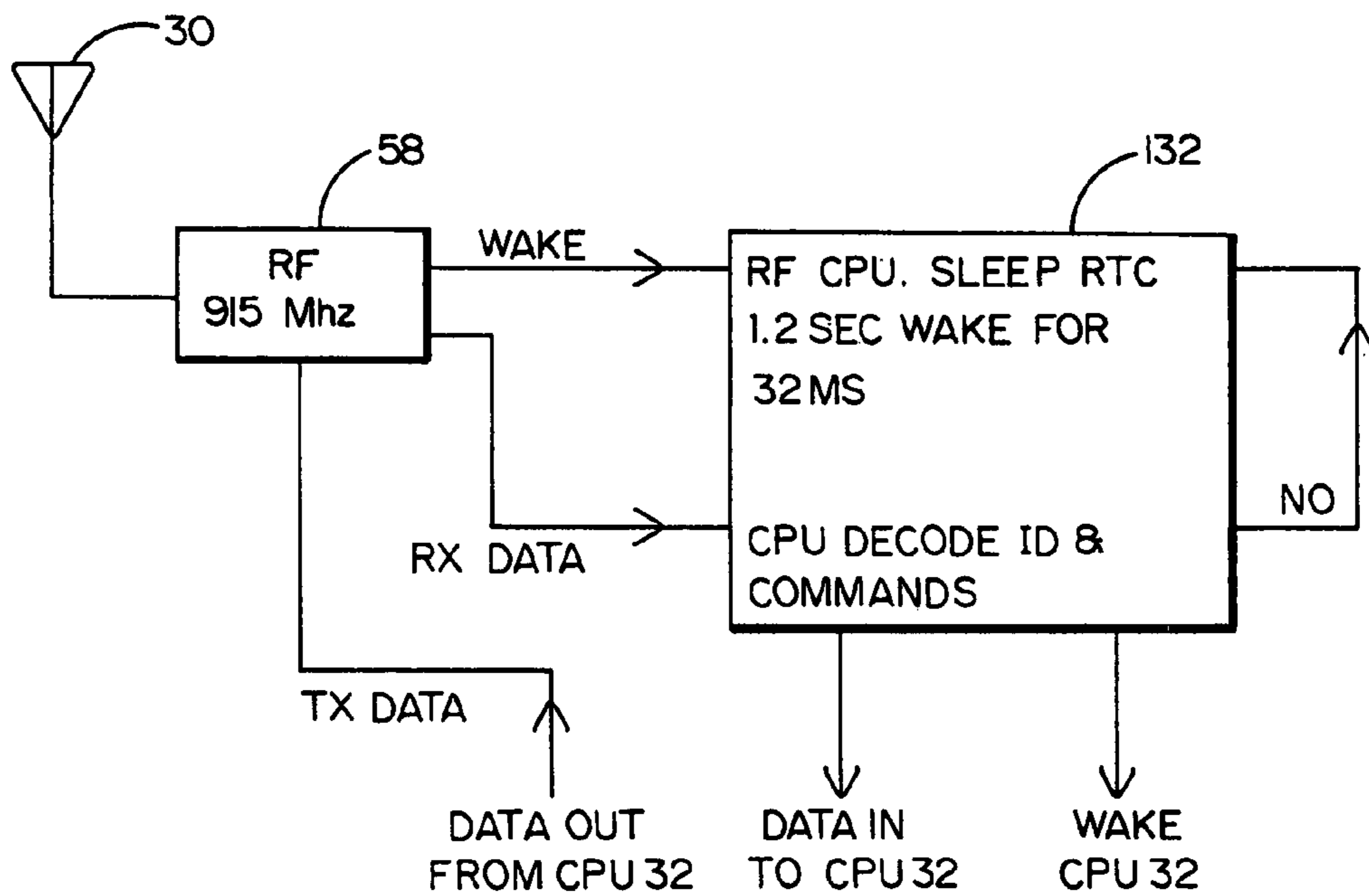
FIG. 11 CPU OF TRANSCEIVER 58
