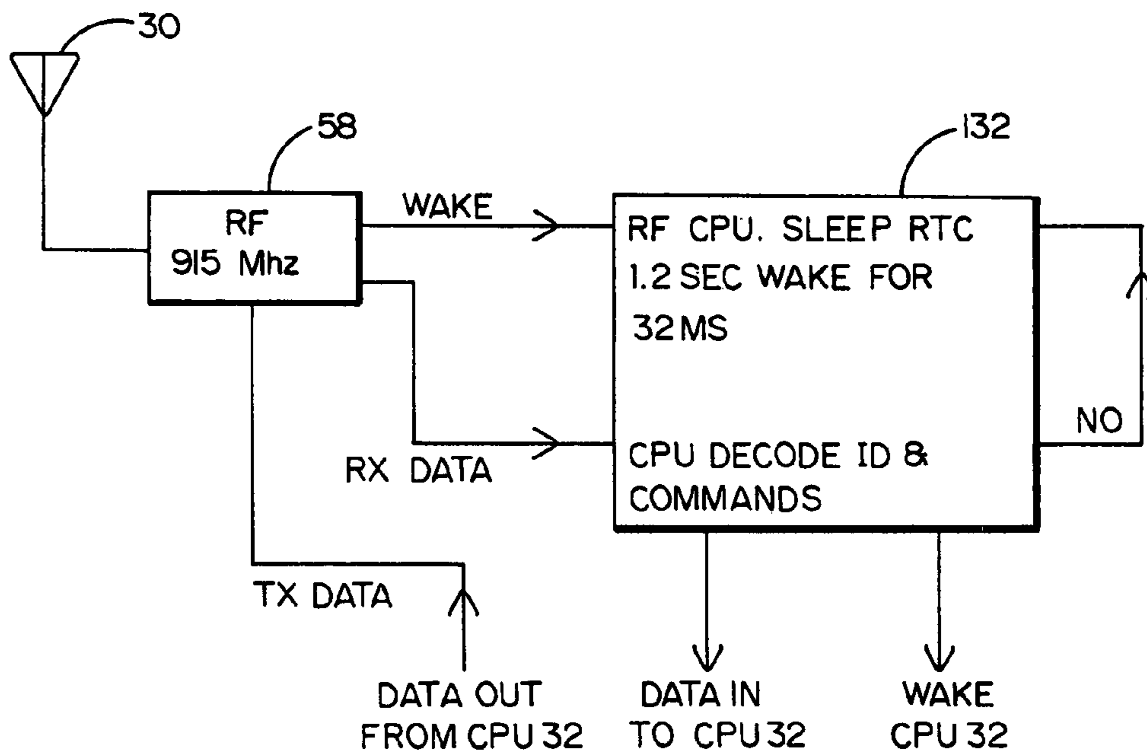
FIG. 11 CPU OF TRANSCEIVER 58
