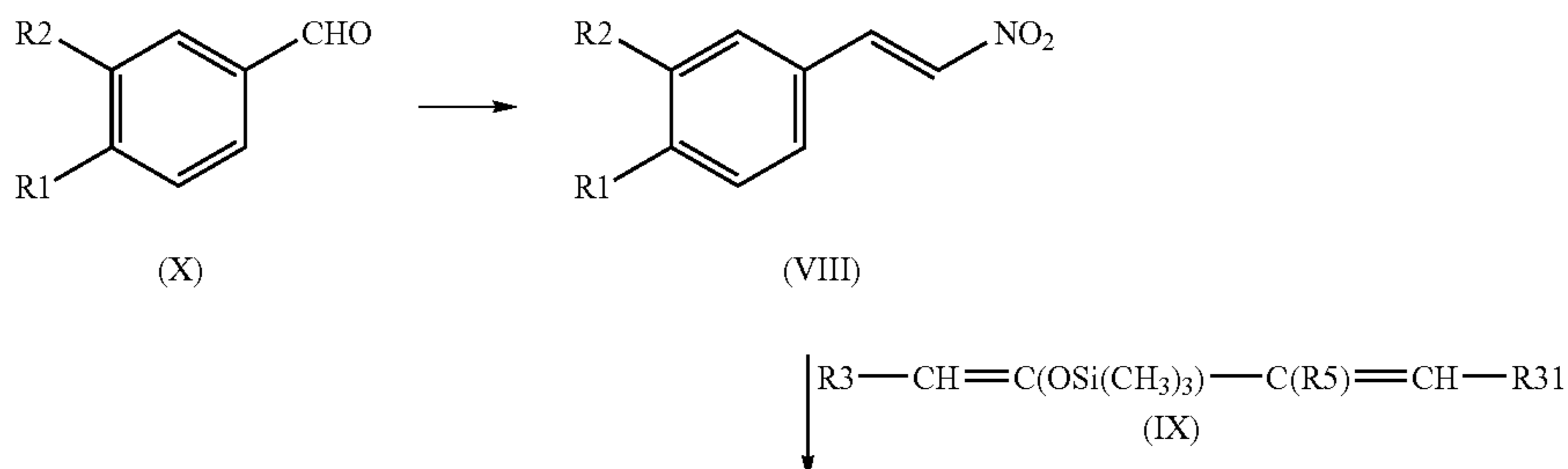
Reaction scheme 2:
