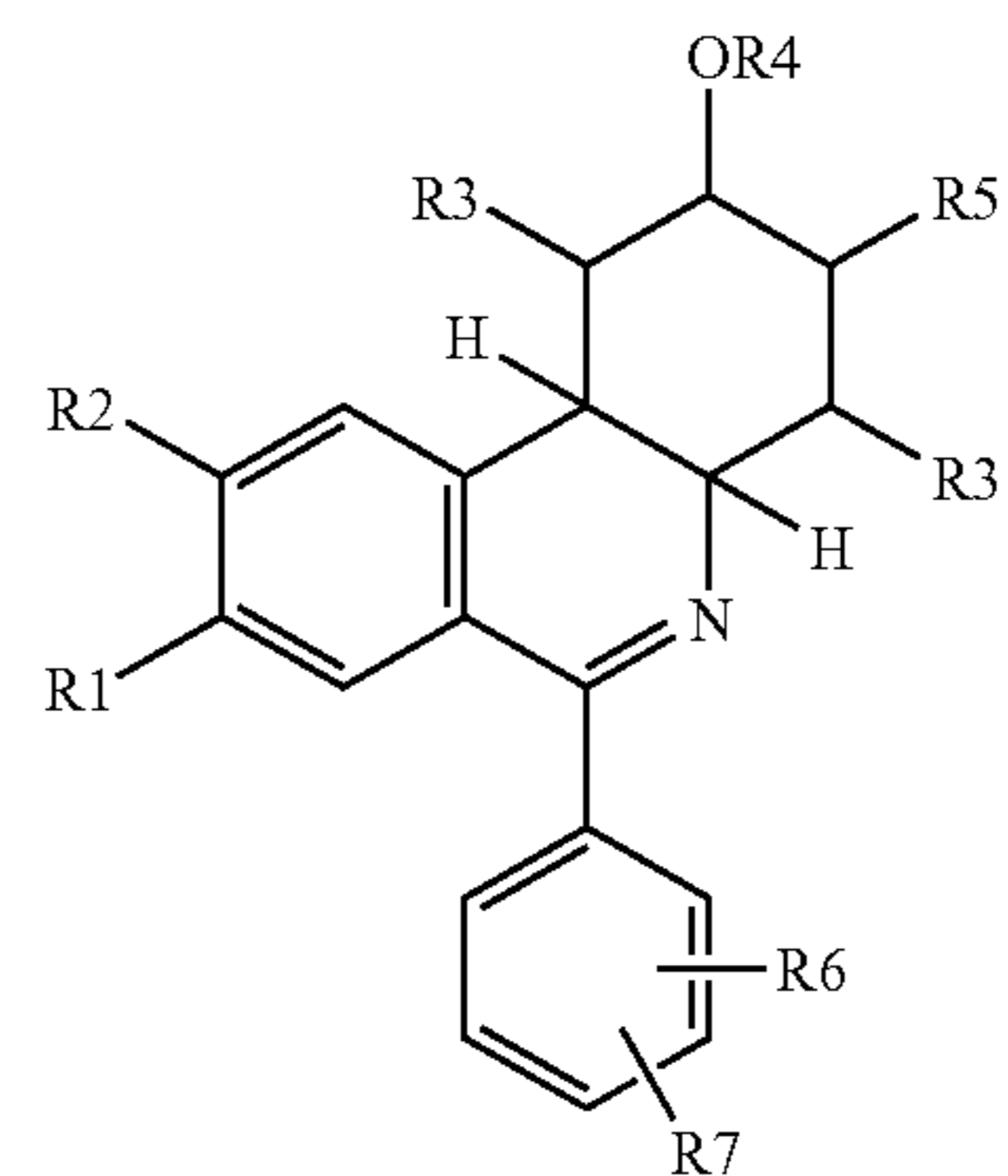
(I)
