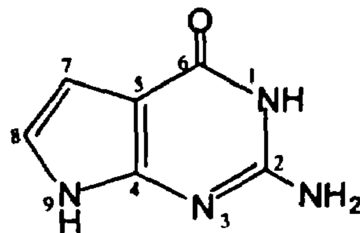
2-Amino-6-oxy-7-deaza-purine or 7-Deaza-guanine
