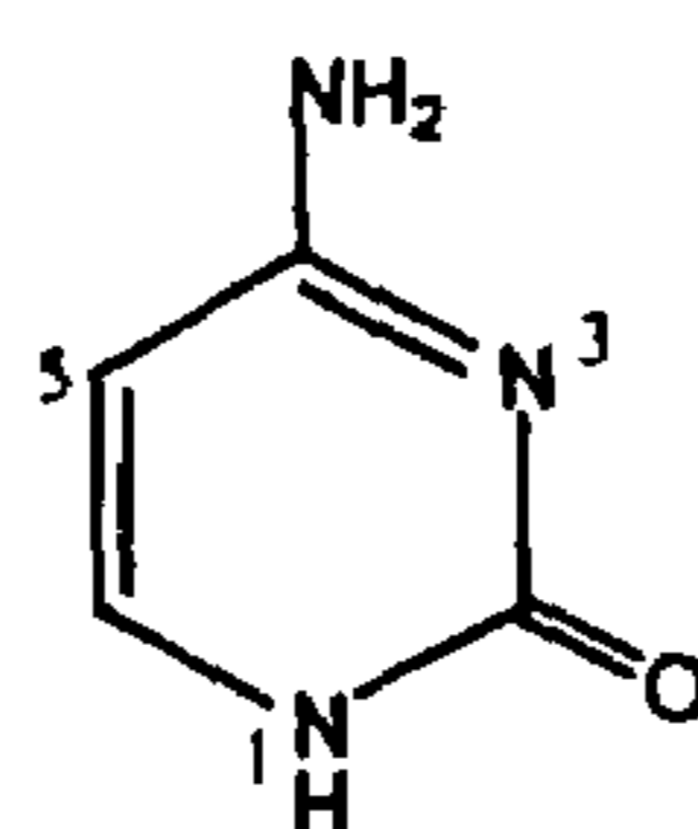
2-Oxy-4-amino pyrimidine or cytosine
