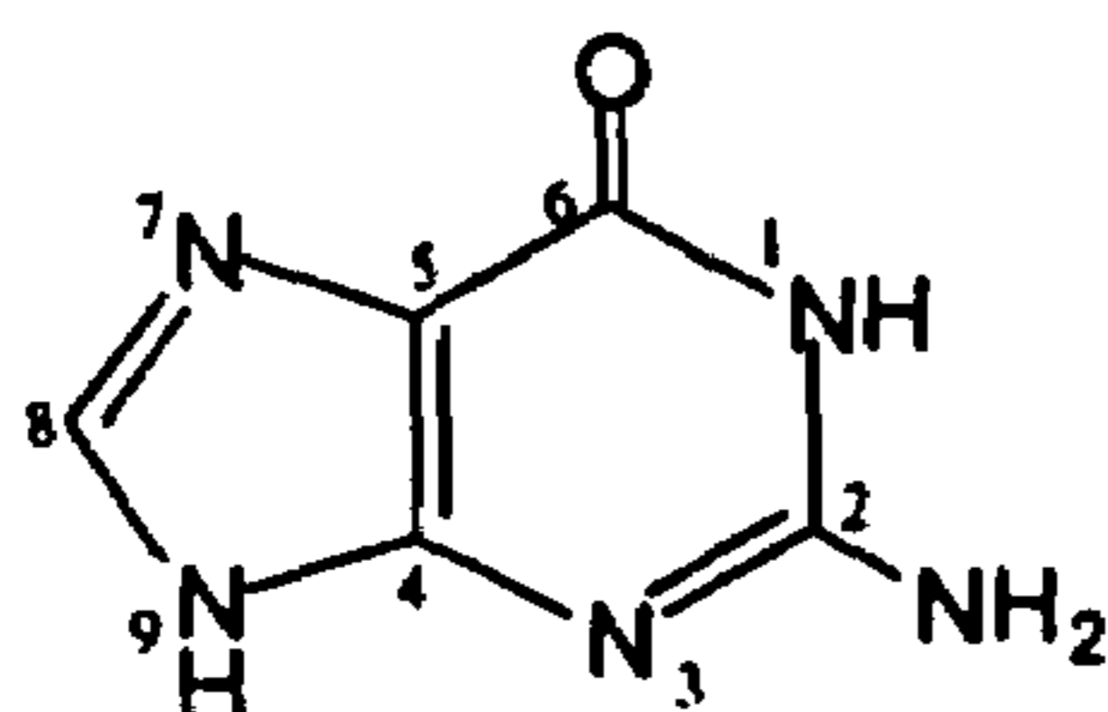
2-Amino-6-oxy-purine or Guanine
