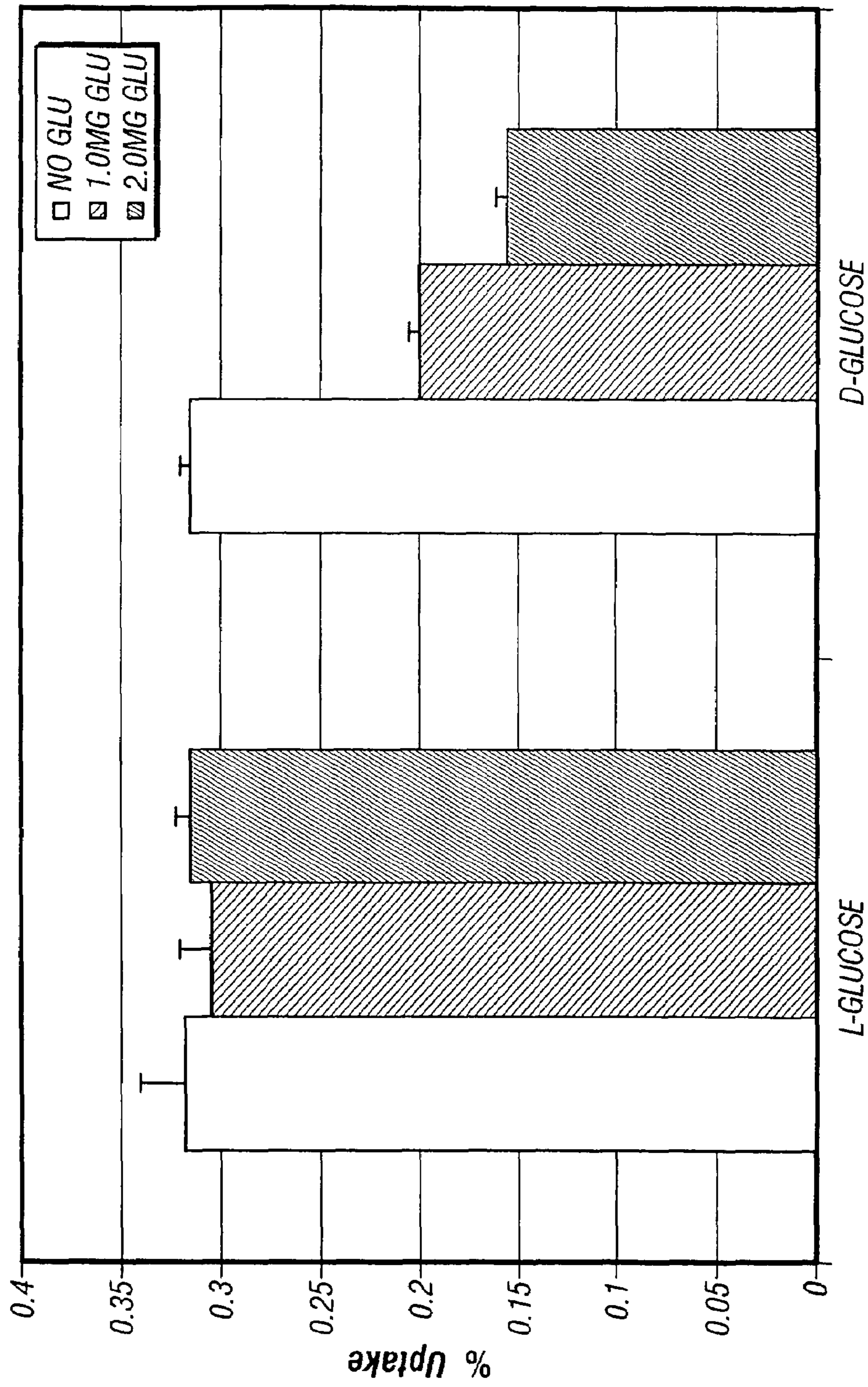
Glucose Isomer
