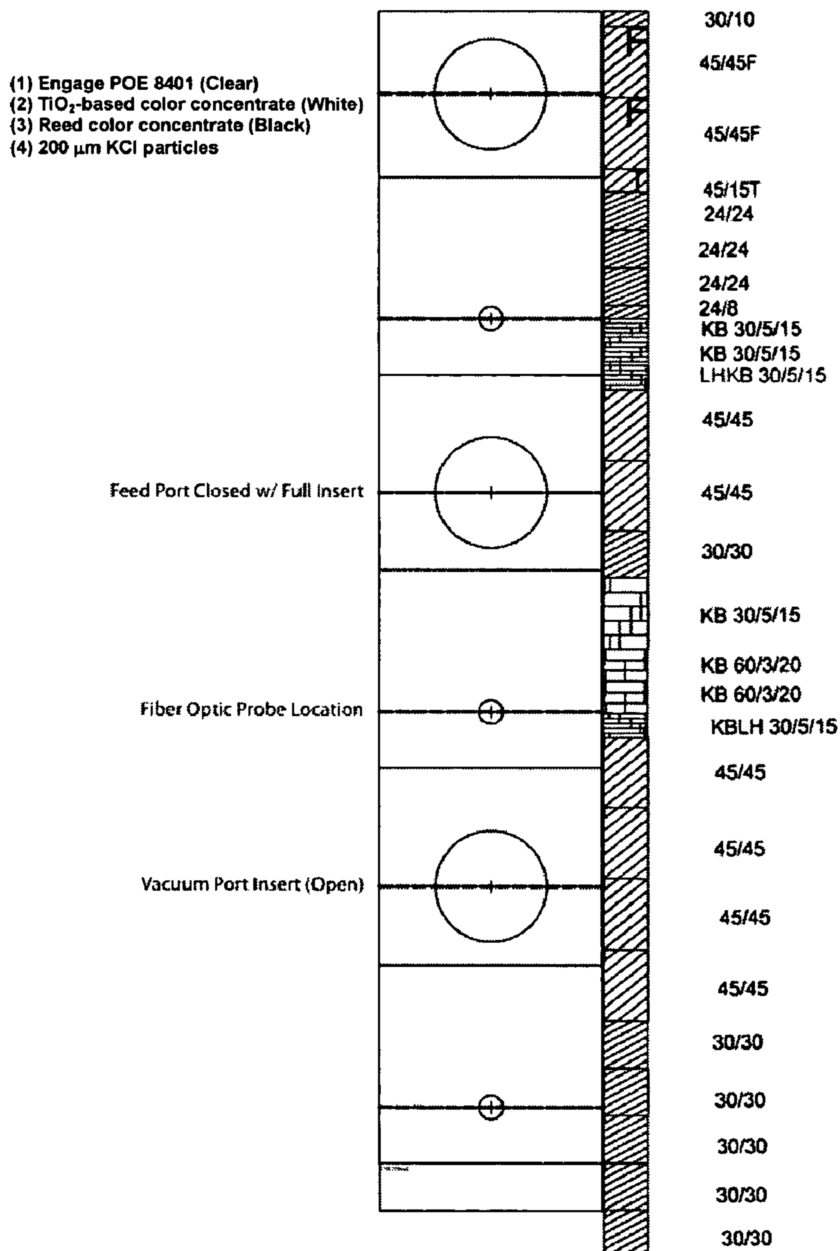
Figure 2. Screw configuration, feed locations, and probe locations used for the 28 mm TSE experiments.
