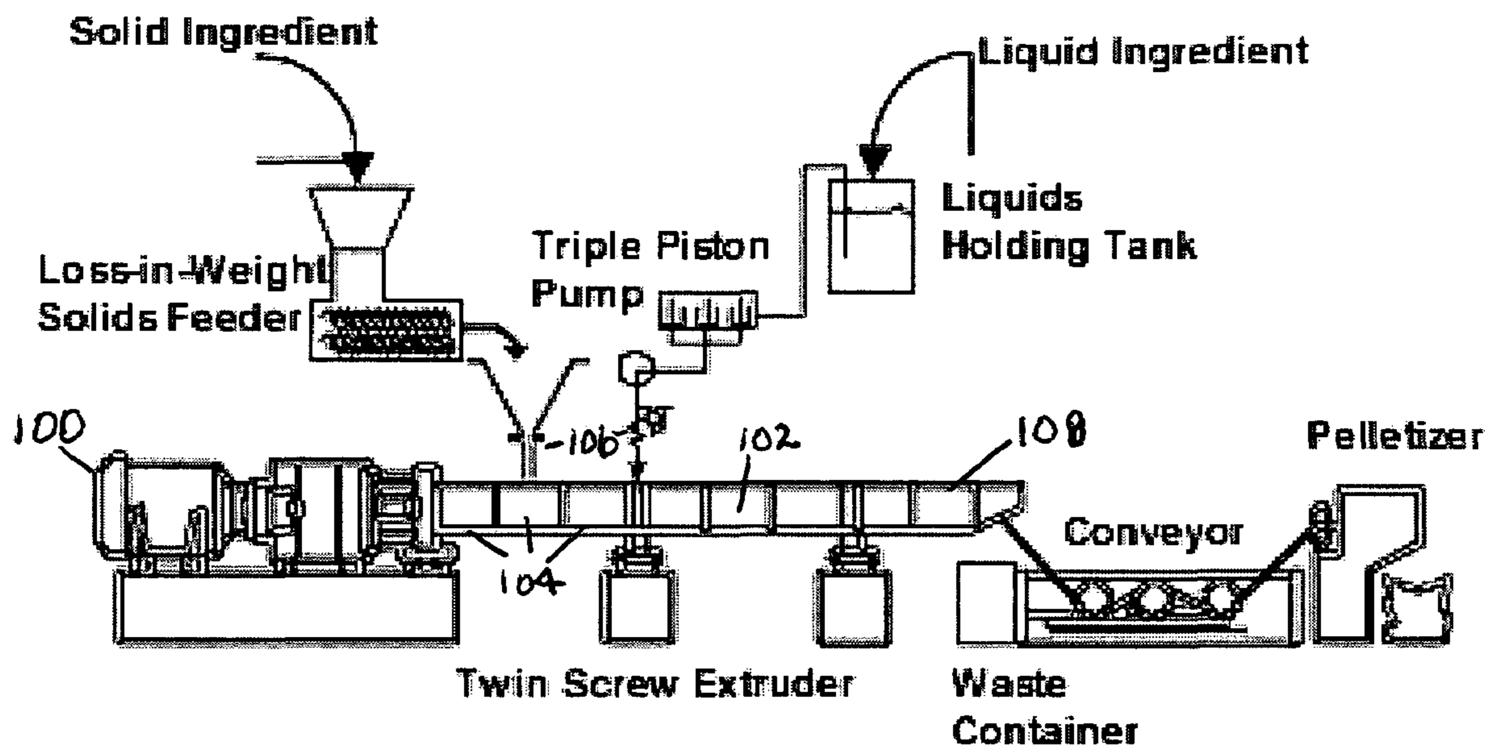
Twin-screw extrusion process used to fabricate continuously graded particle-reinforced polymer composites.
