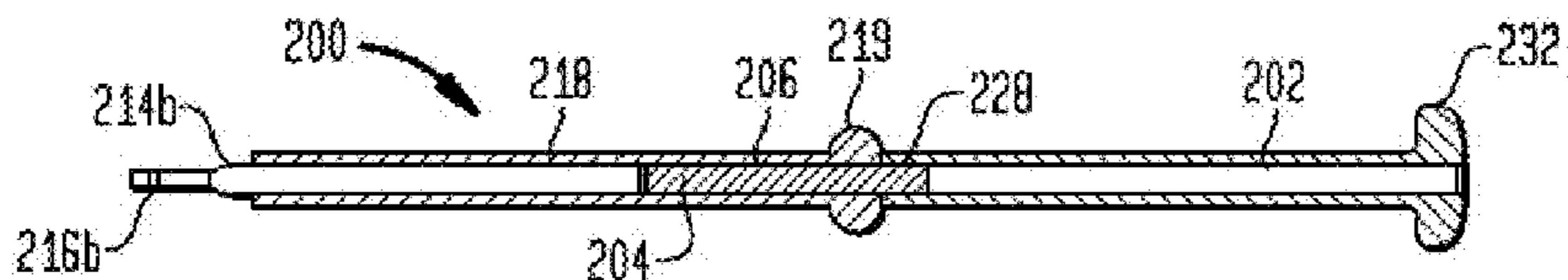
(SECTION A-A OF FIG. 2b)
