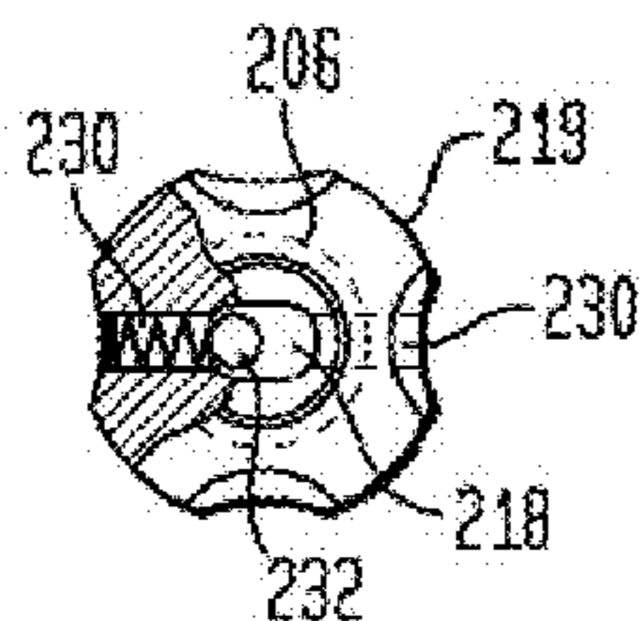
FIG. 2i (SECTION E-E OF FIG. 2d)
