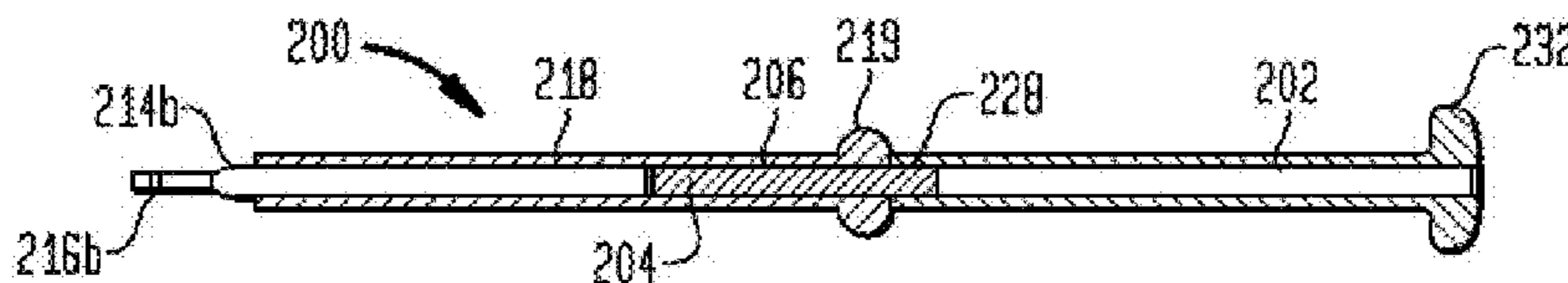
FIG. 2k (SECTION A-A OF FIG. 2b)
