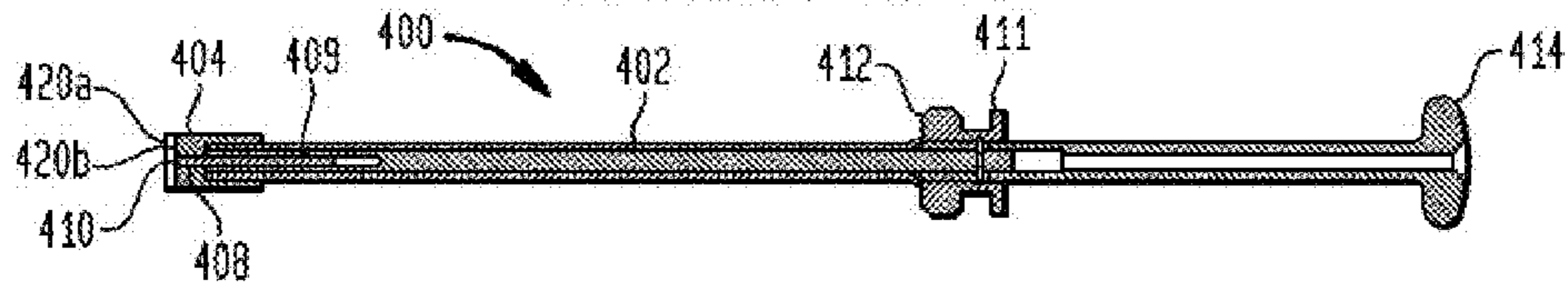
FIG. 4c (SECTION A-A OF FIG. 4b)
