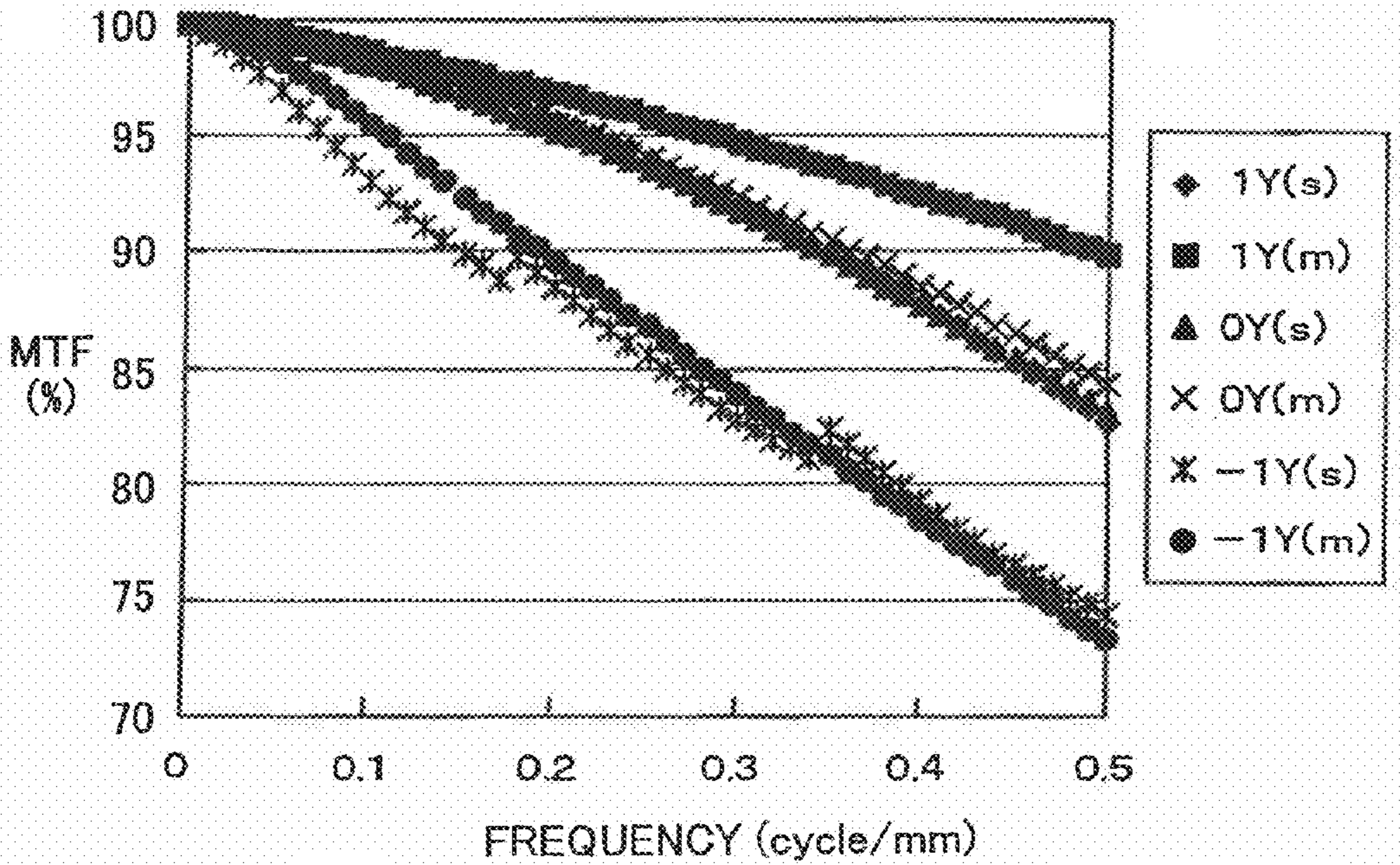
MTF CHARACTERISTICS 3 1.0X
