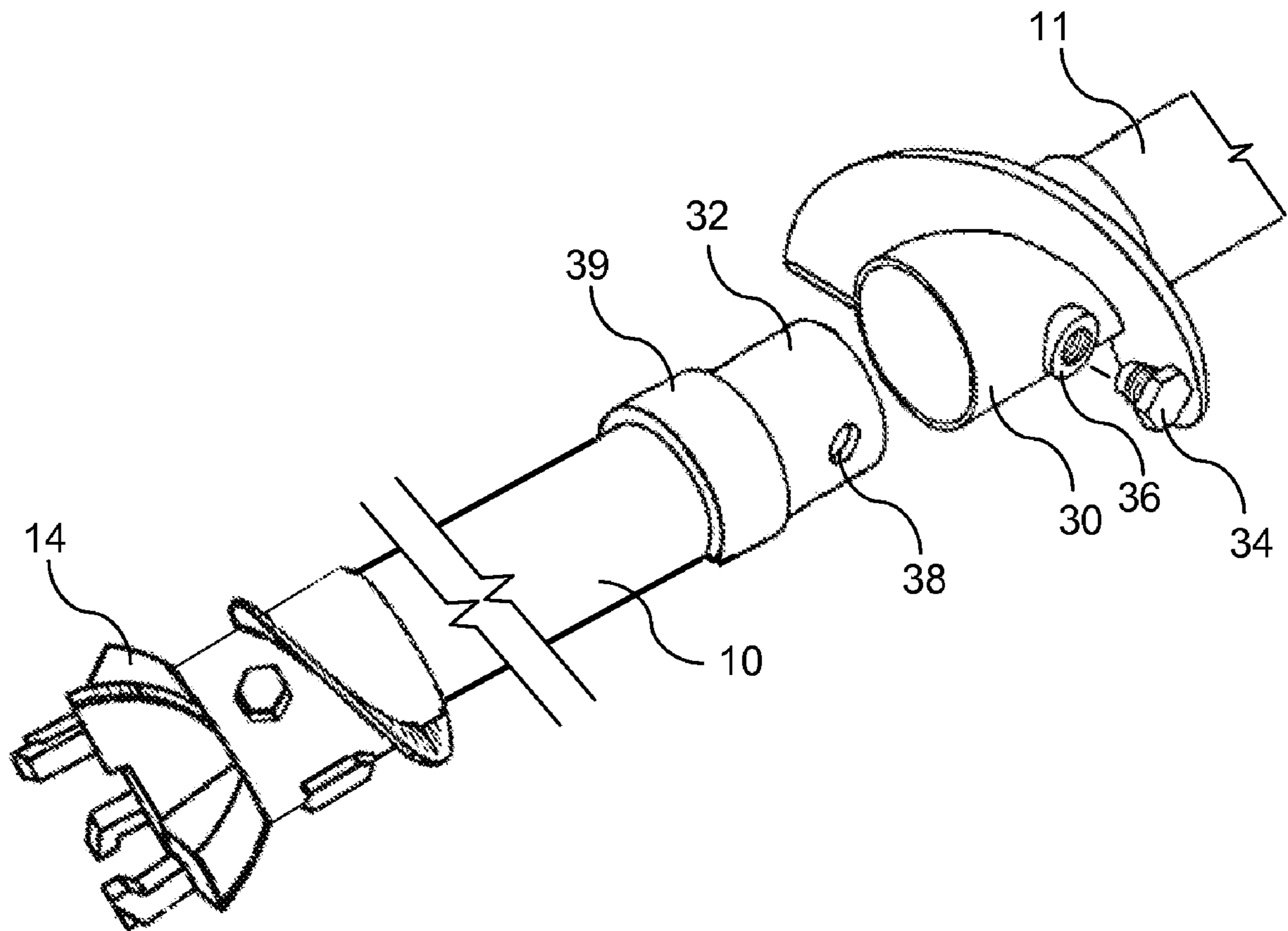
FIG. 3 PRIOR ART
