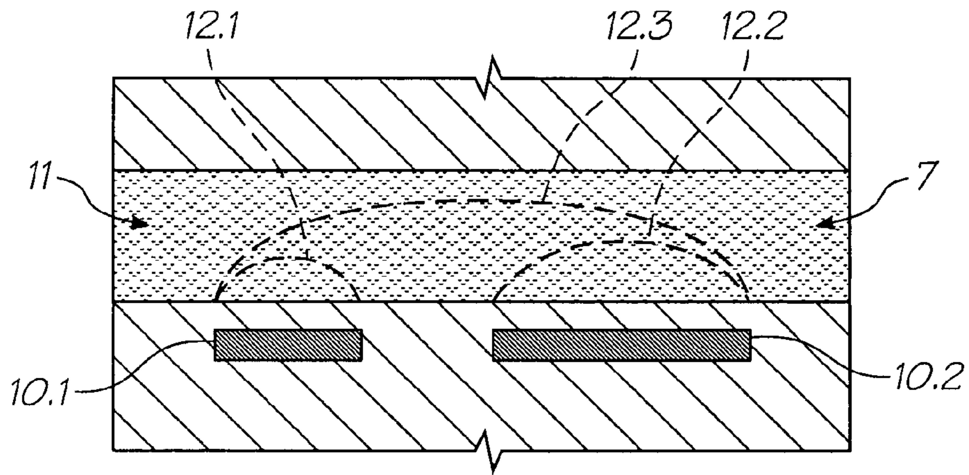
FIG. 52 (PRIOR ART)
