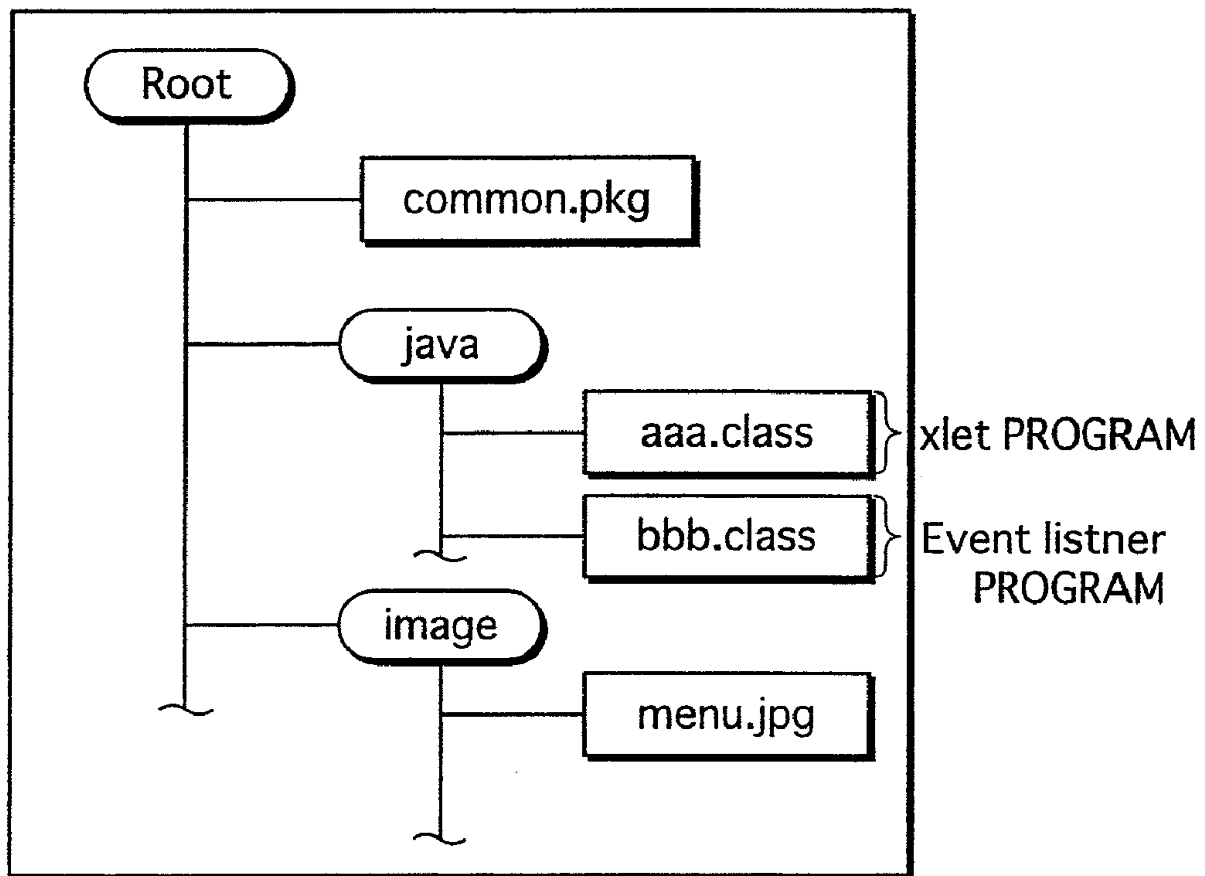
JAR FILE
