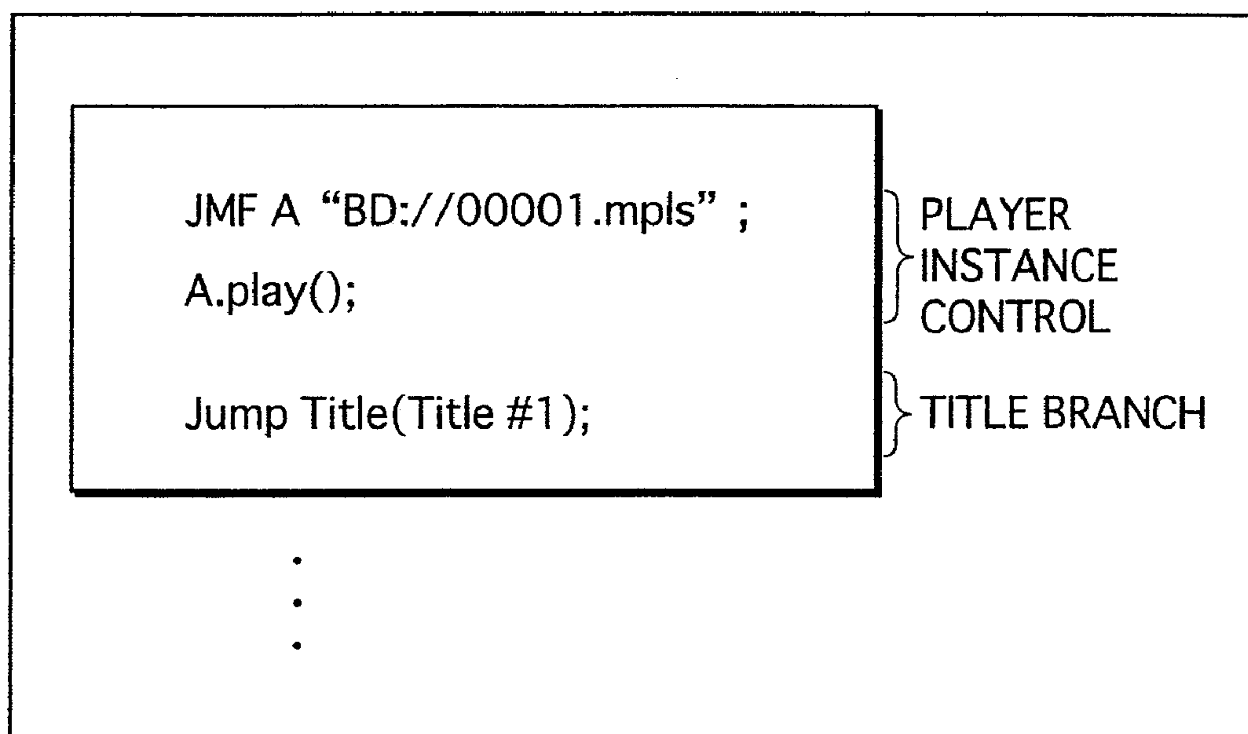
xlet PROGRAM
