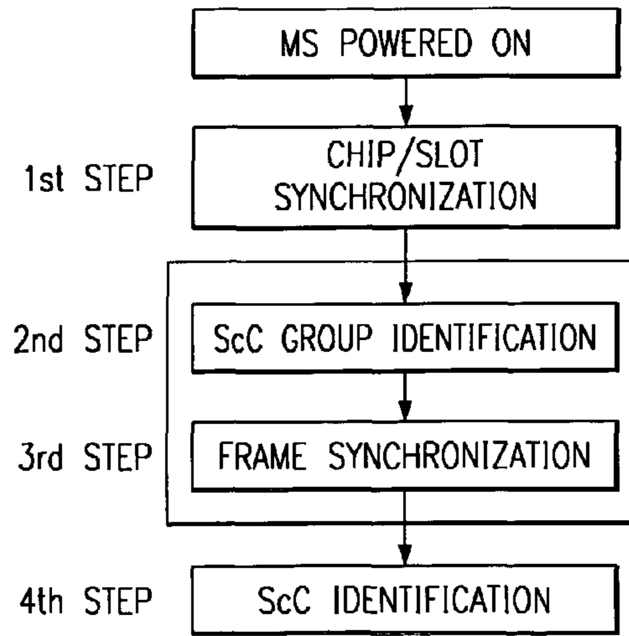
FIG. 3C (PRIOR ART)
