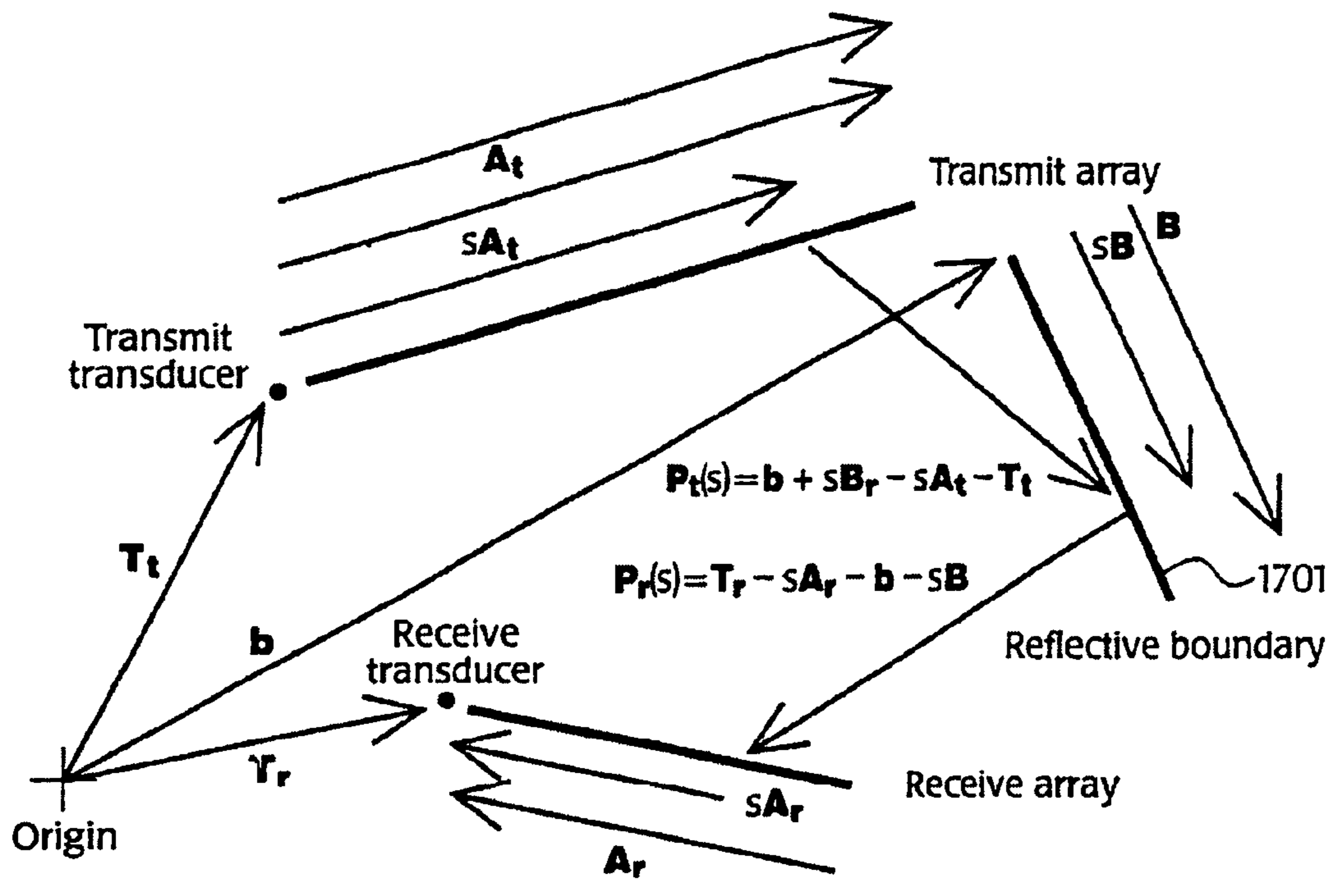
Fig. 17 - Coordinate subsystem with scattering
