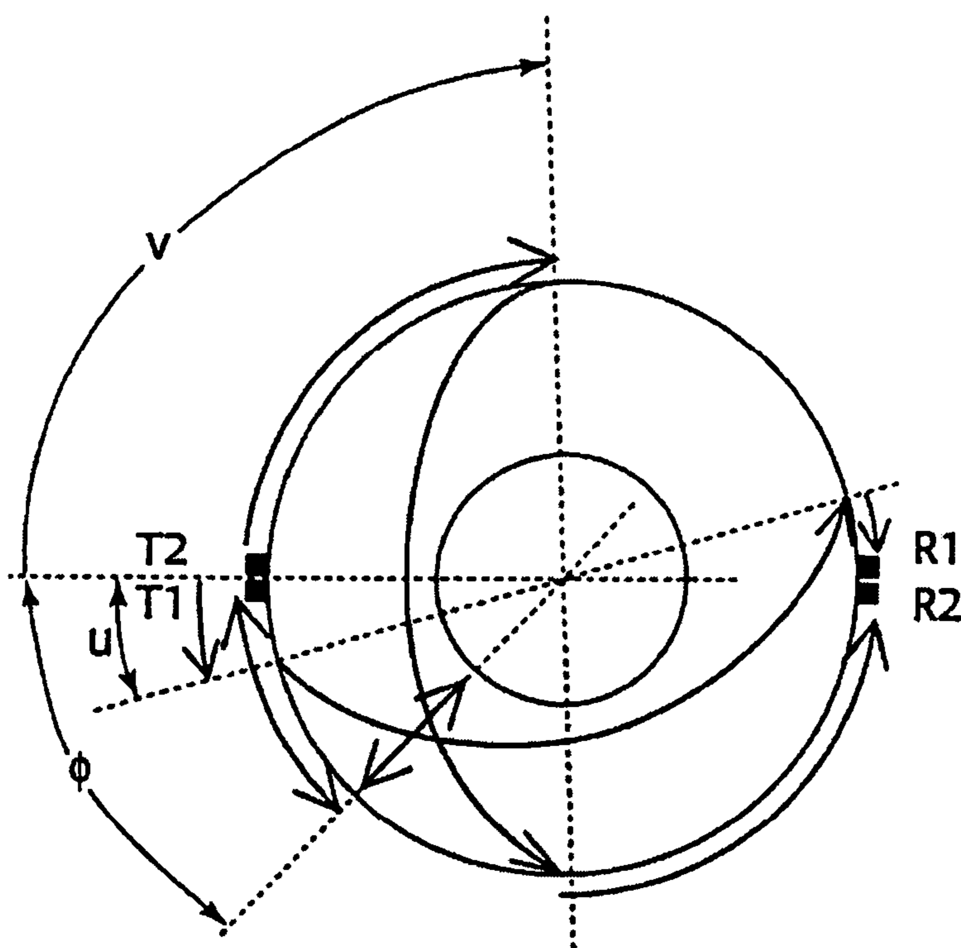
(b) Top view
