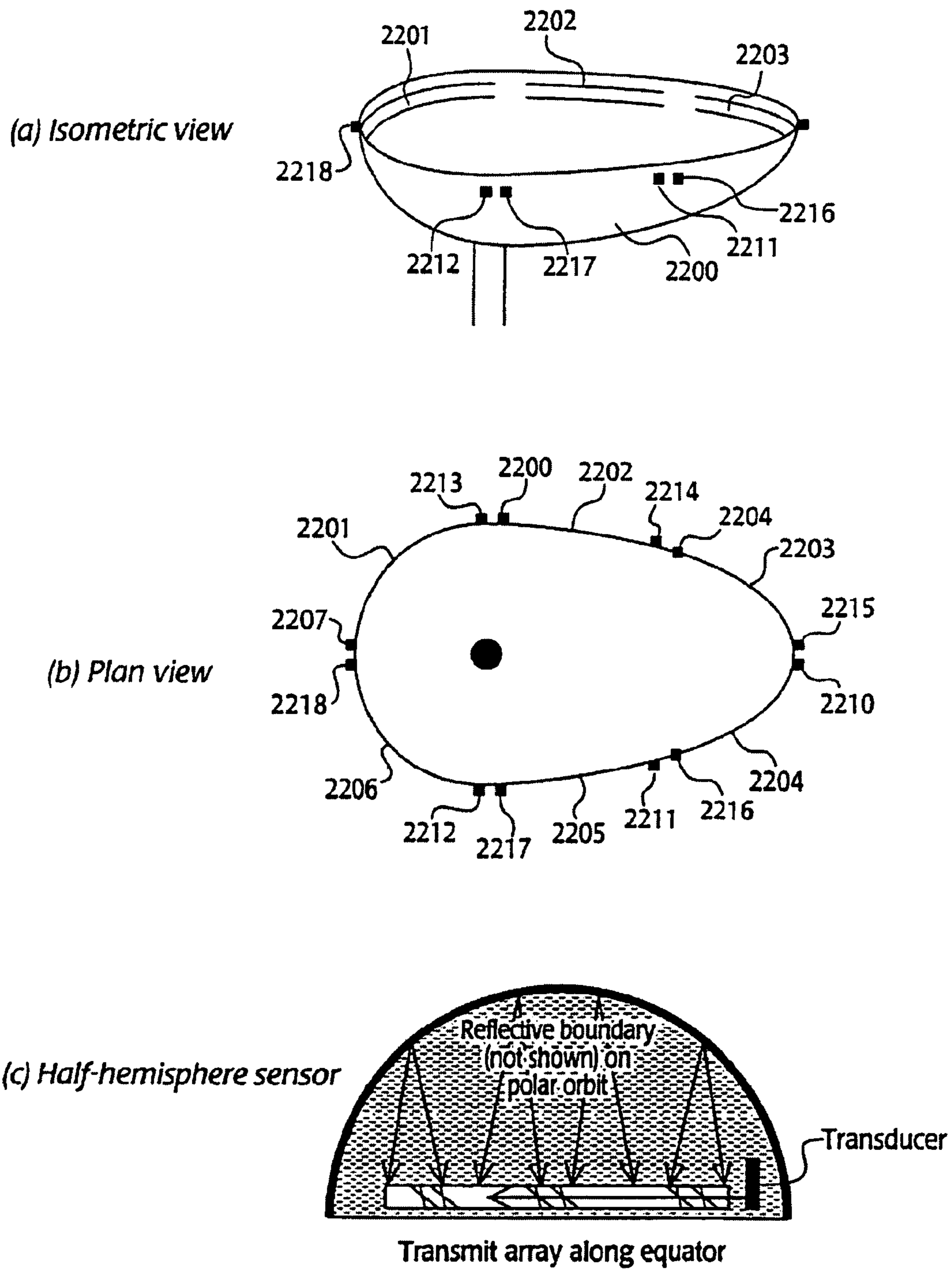
Fig. 22 - Basin sensor
