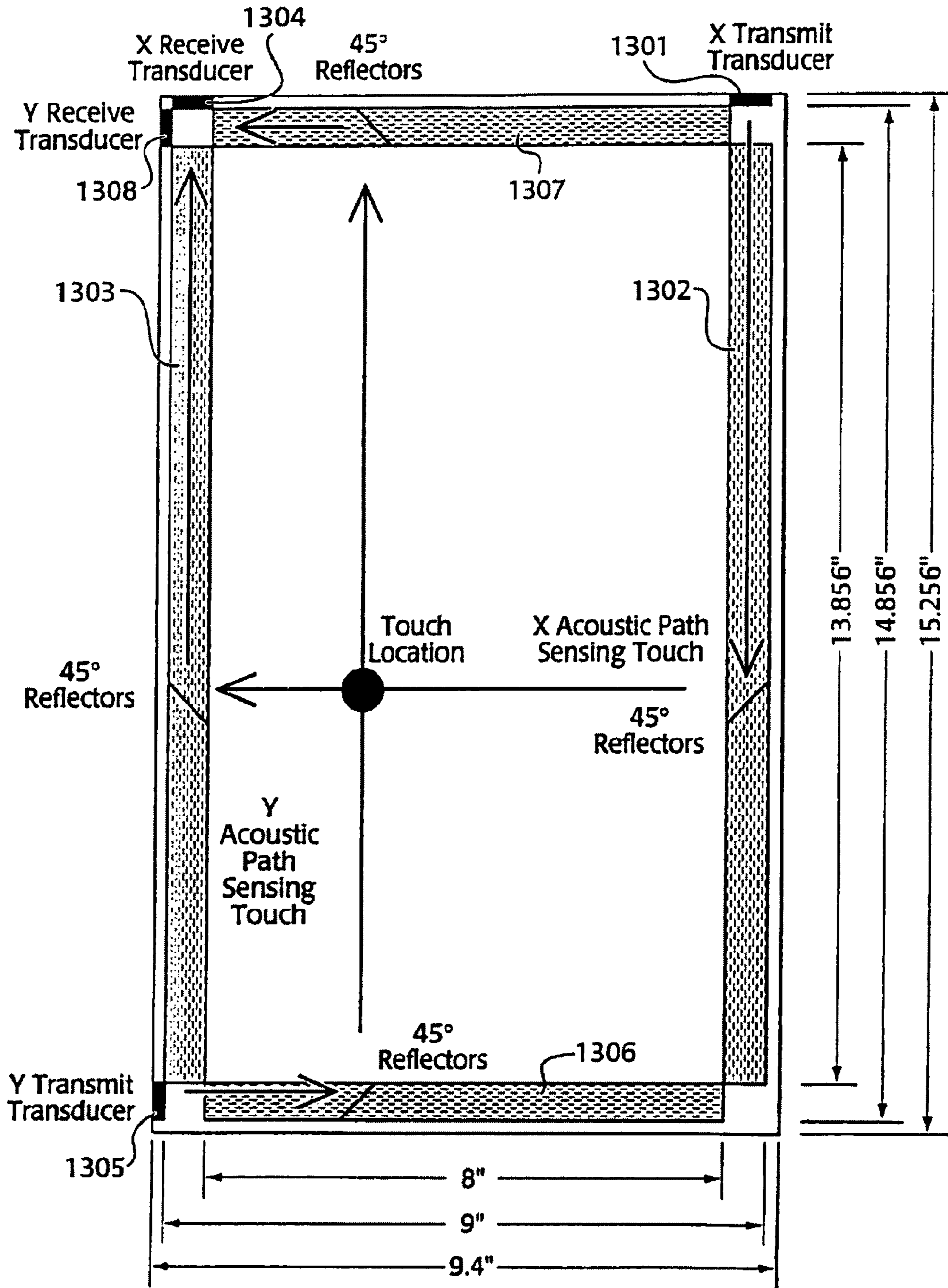
Figure 13 - X, Y, 30° Sensor: (a) X & Y Subsystems
