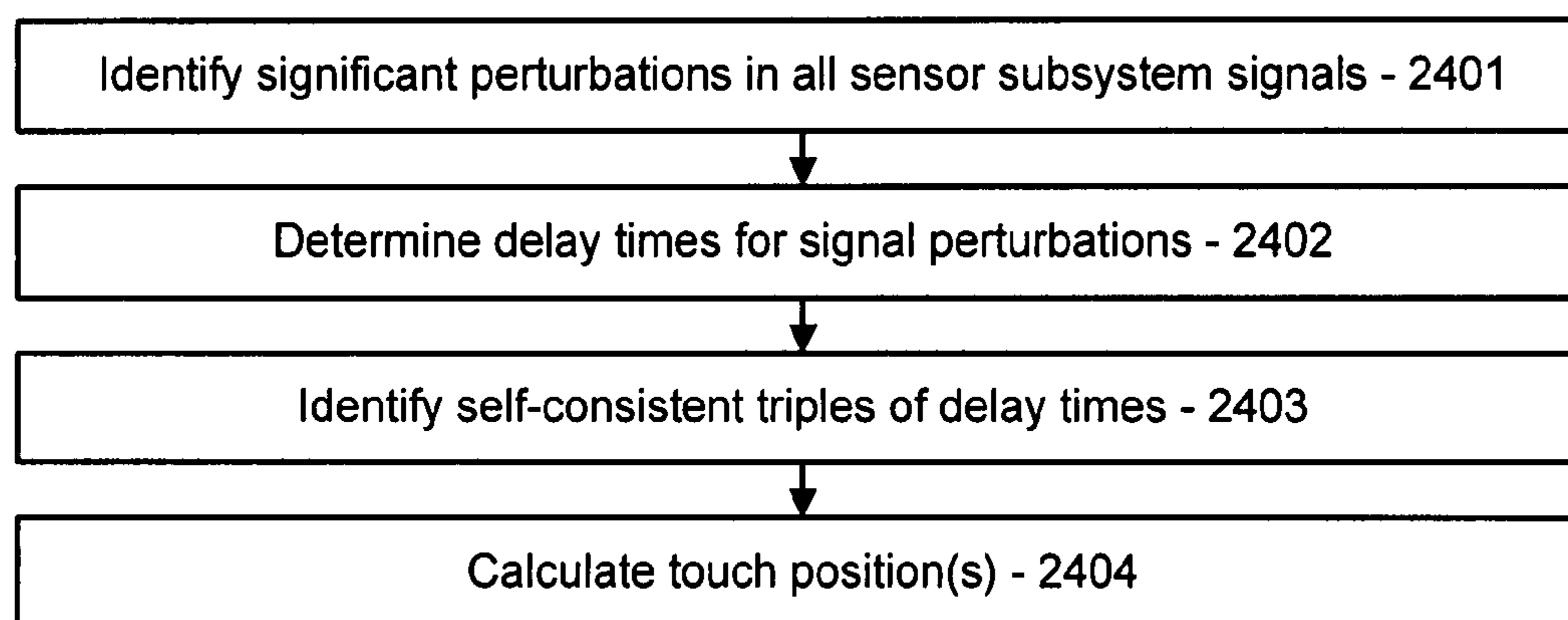
Fig. 24(a) – Redundancy-check algorithm
