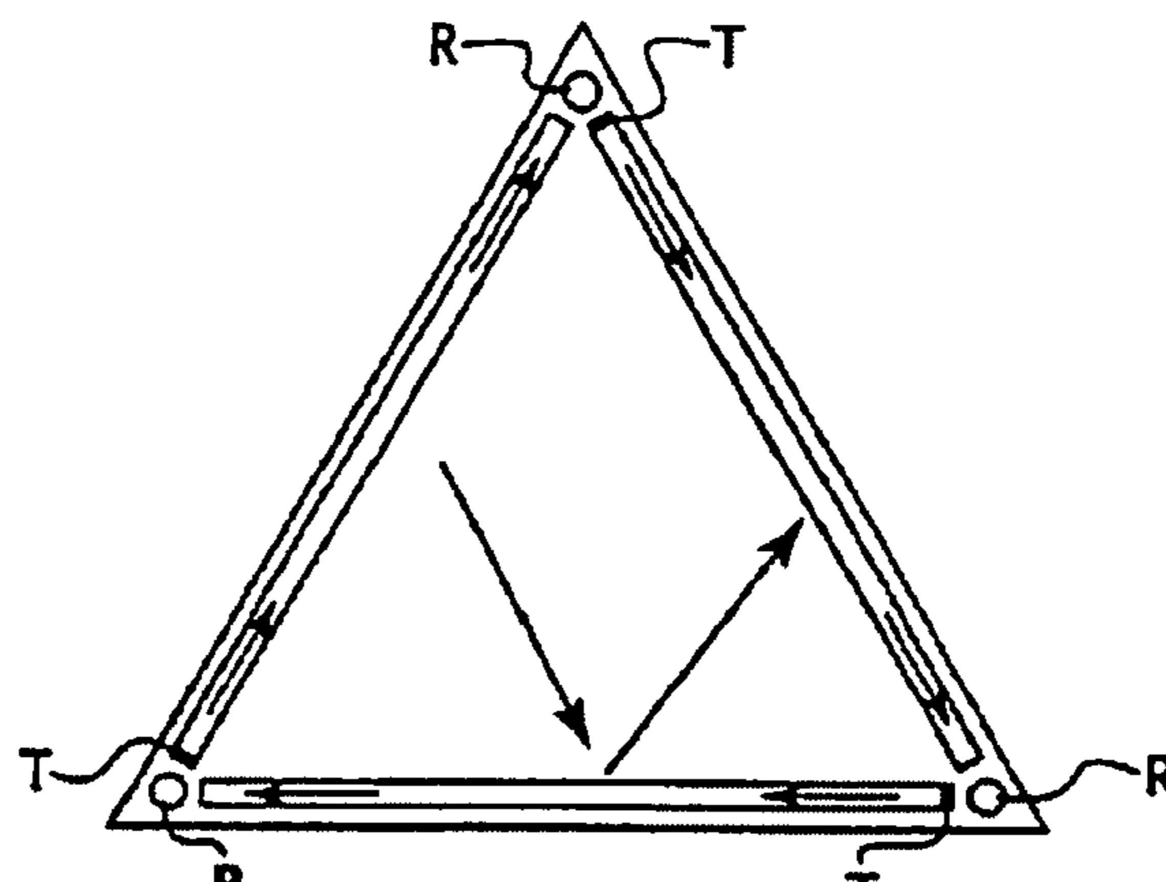
(c) Triangular sensor geometry
