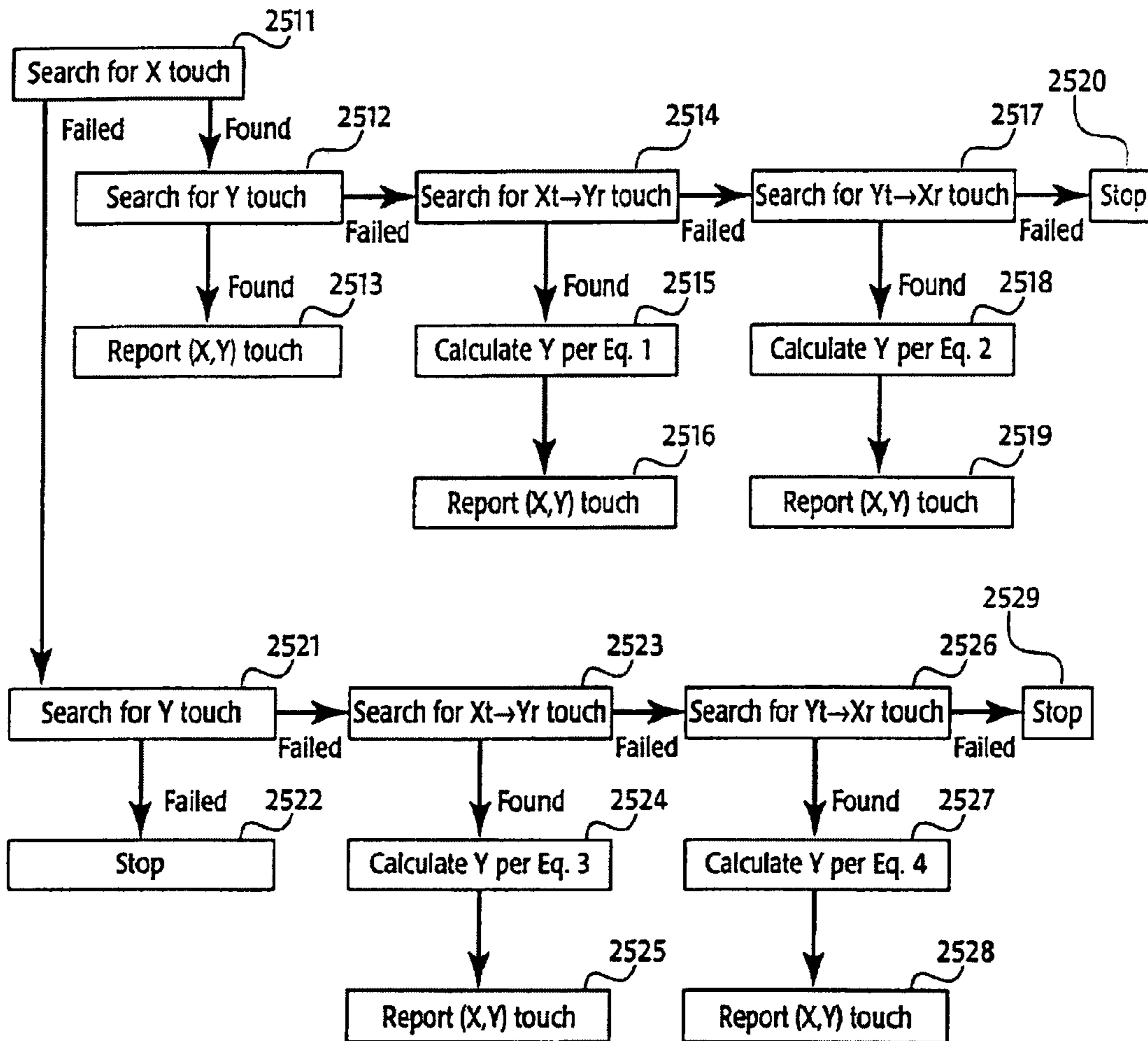
Fig. 25(b) Anti-Shadowing Algorithm Flow Chart
