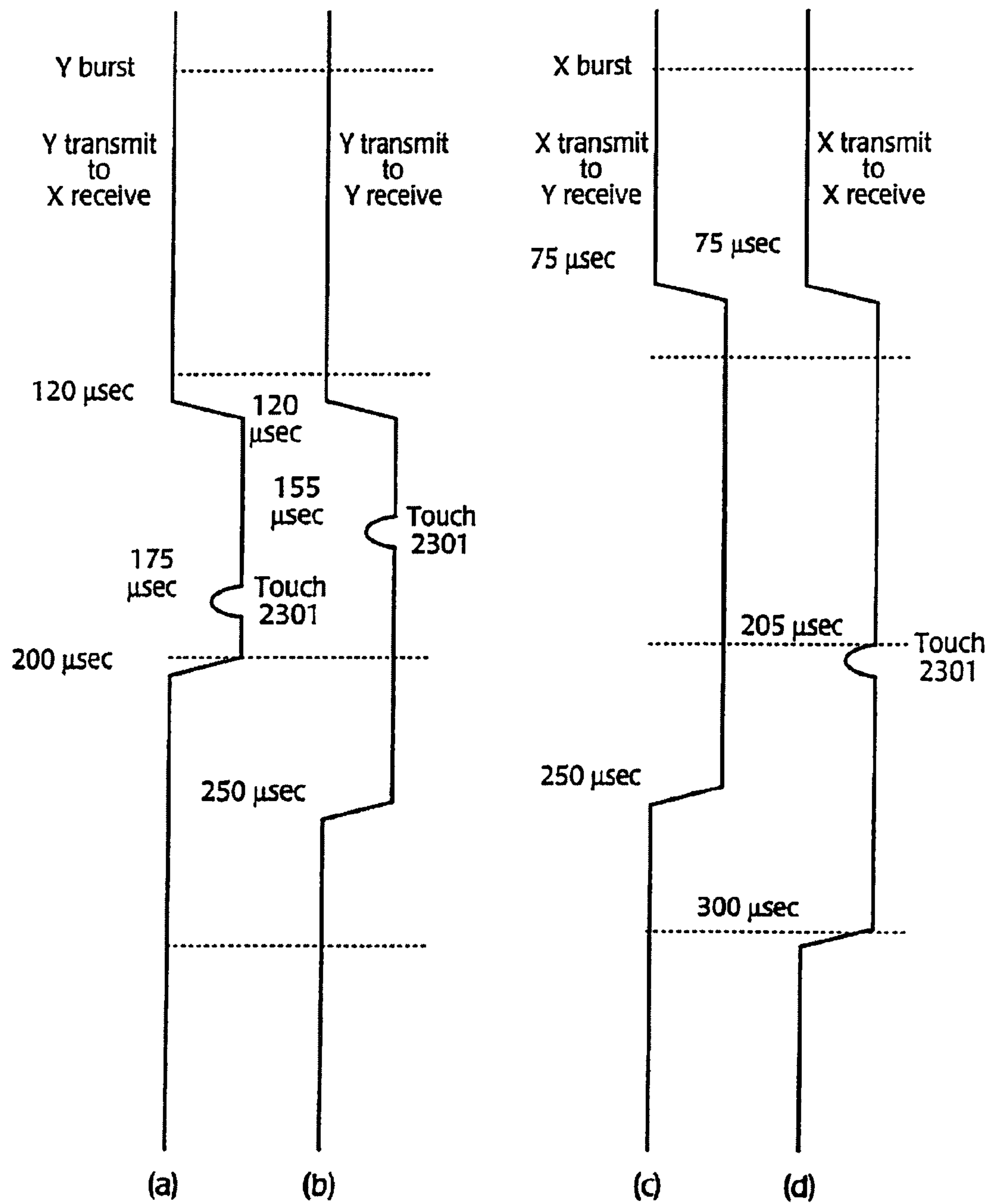
Fig. 23 - Example signals of sensor in Fig. 13
