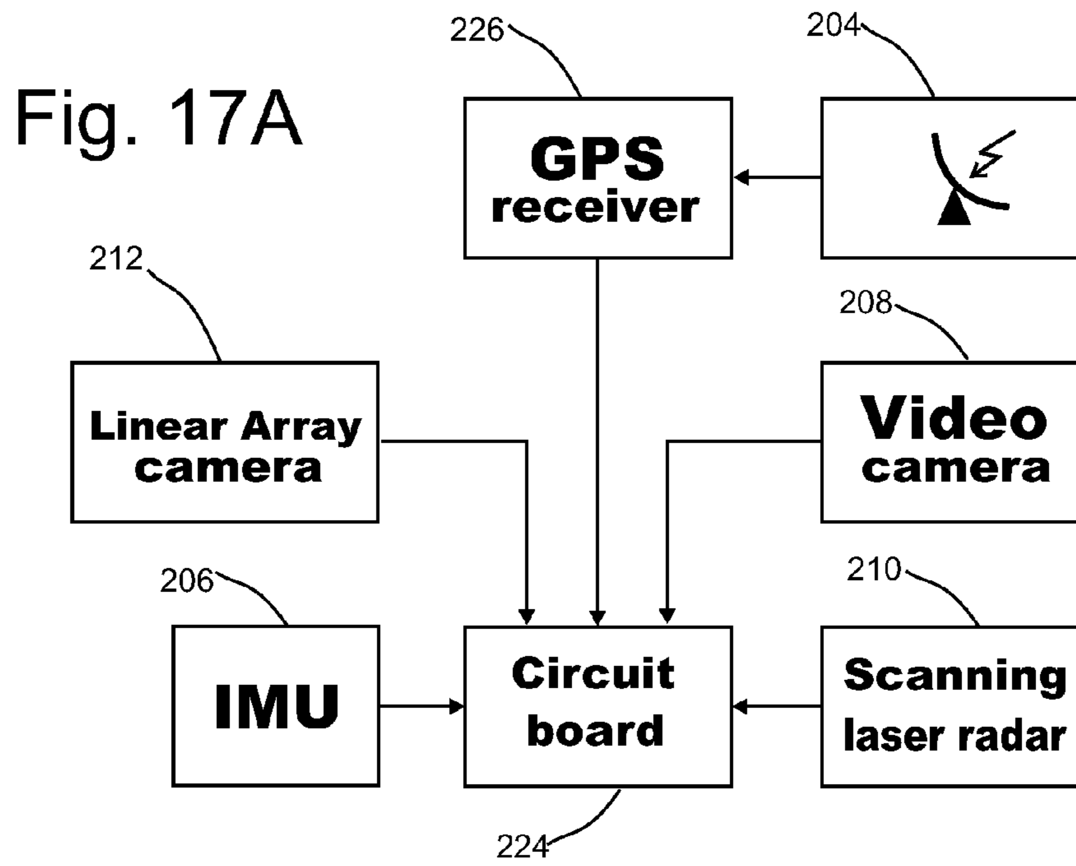
Data acquisition module
