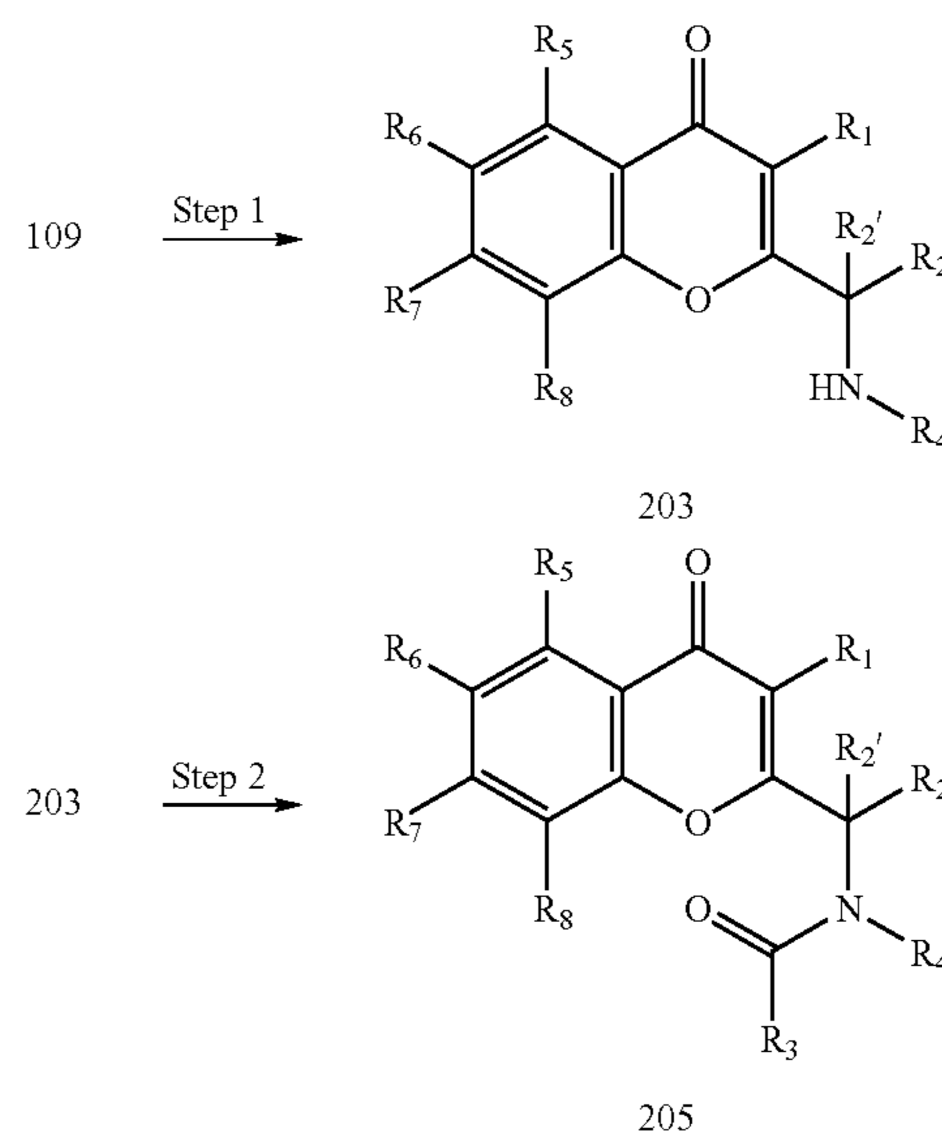
Reaction Scheme 2
