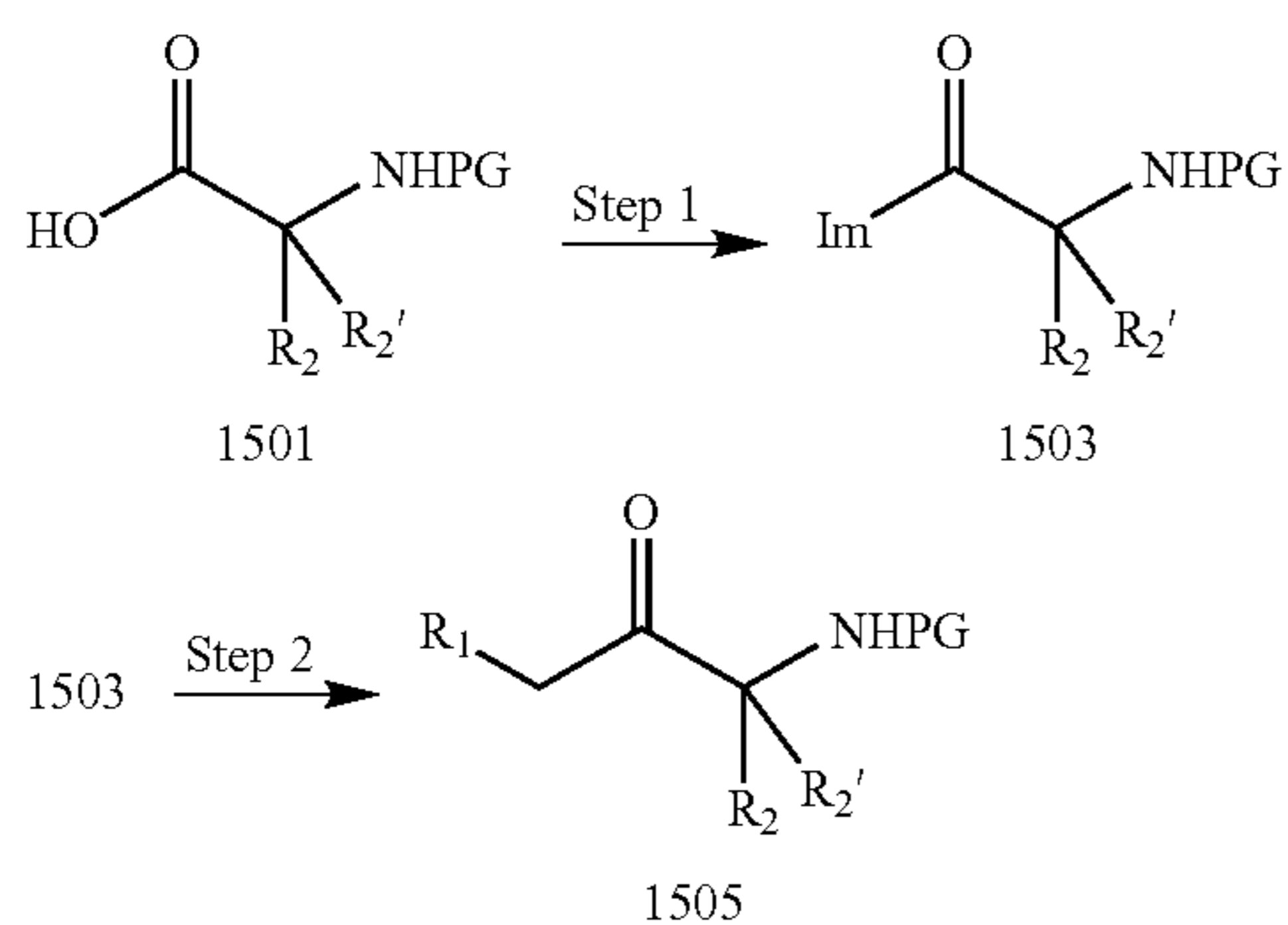
Reaction Scheme 15
