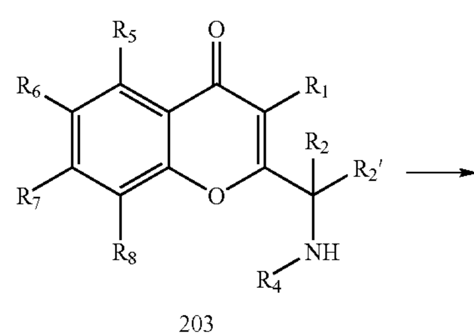
Reaction Scheme 13
