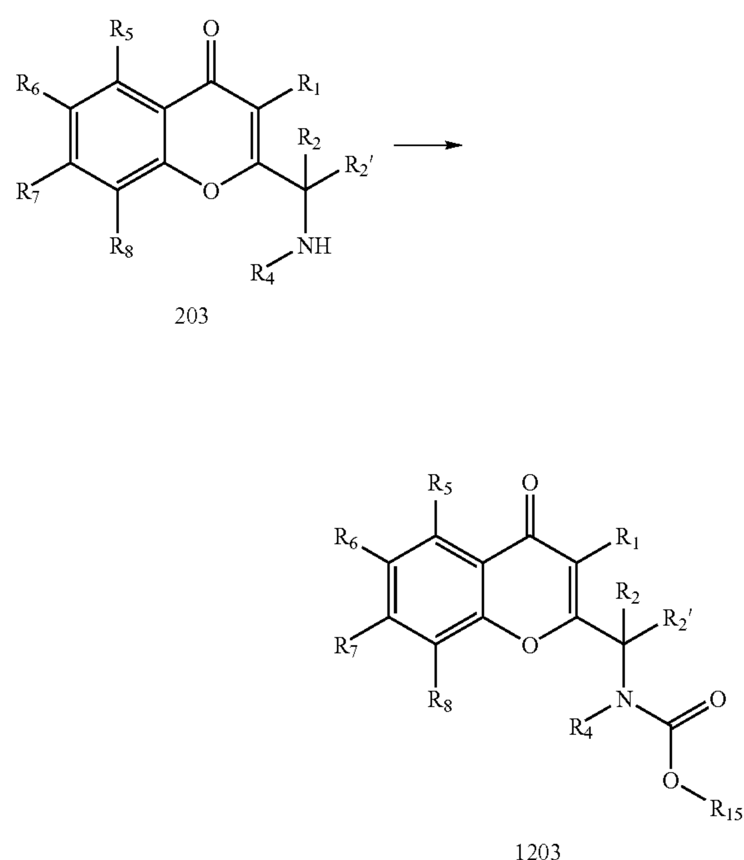
Reaction Scheme 12
