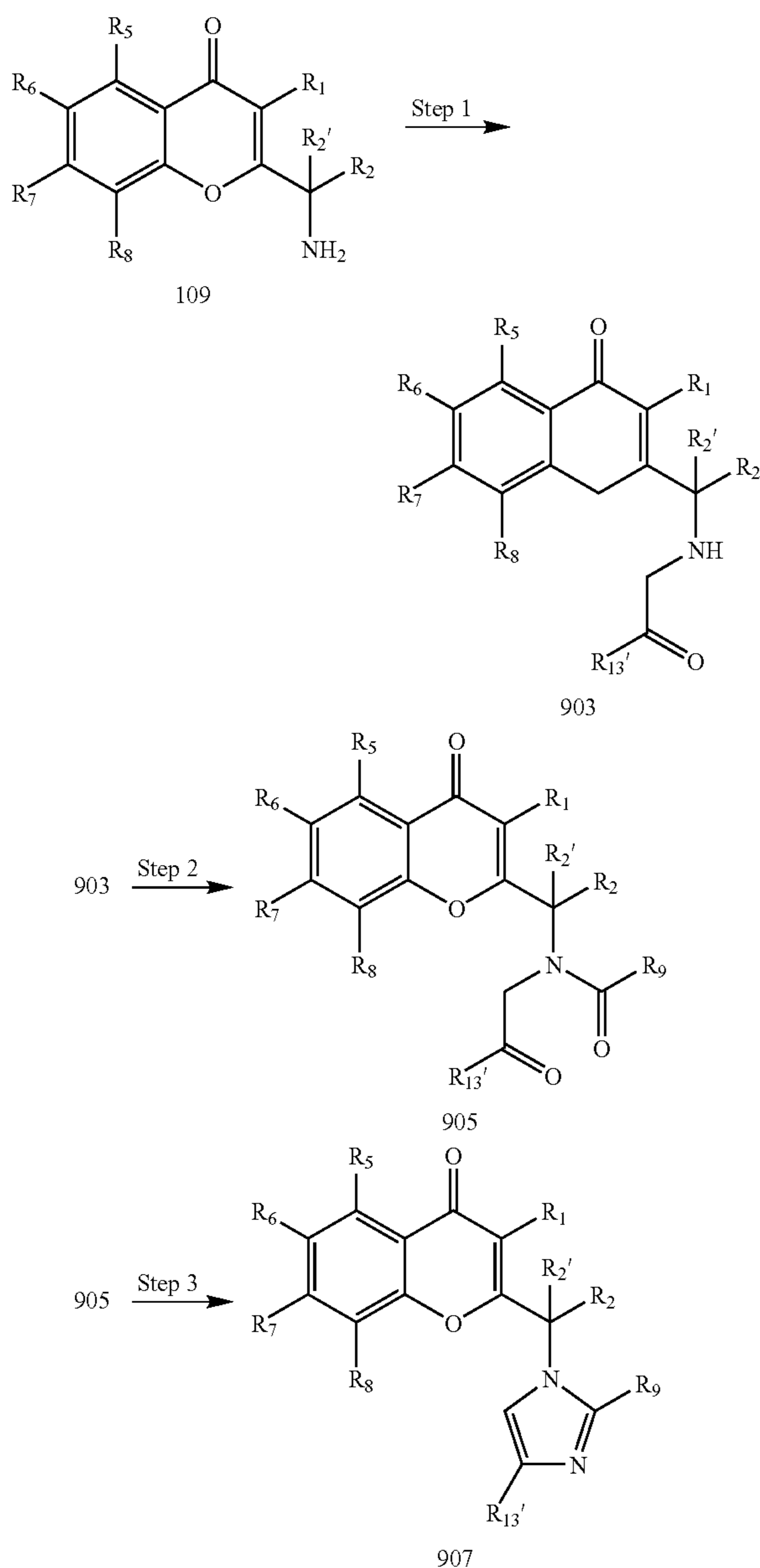
Reaction Scheme 9
