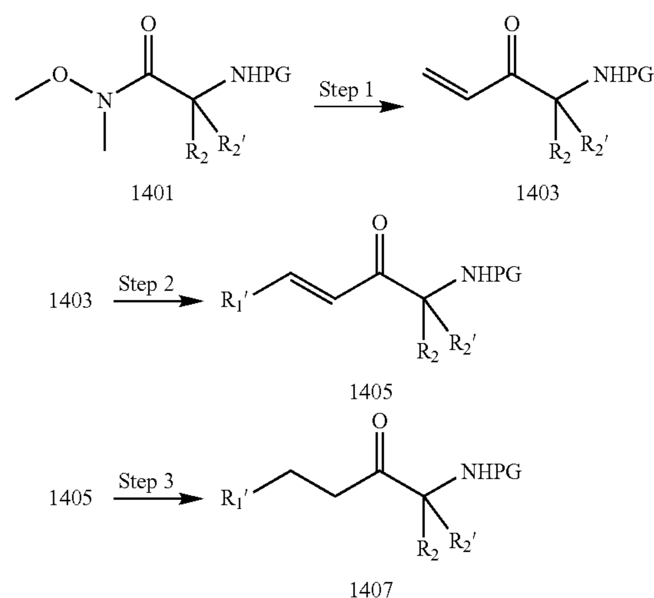
Reaction Scheme 14
