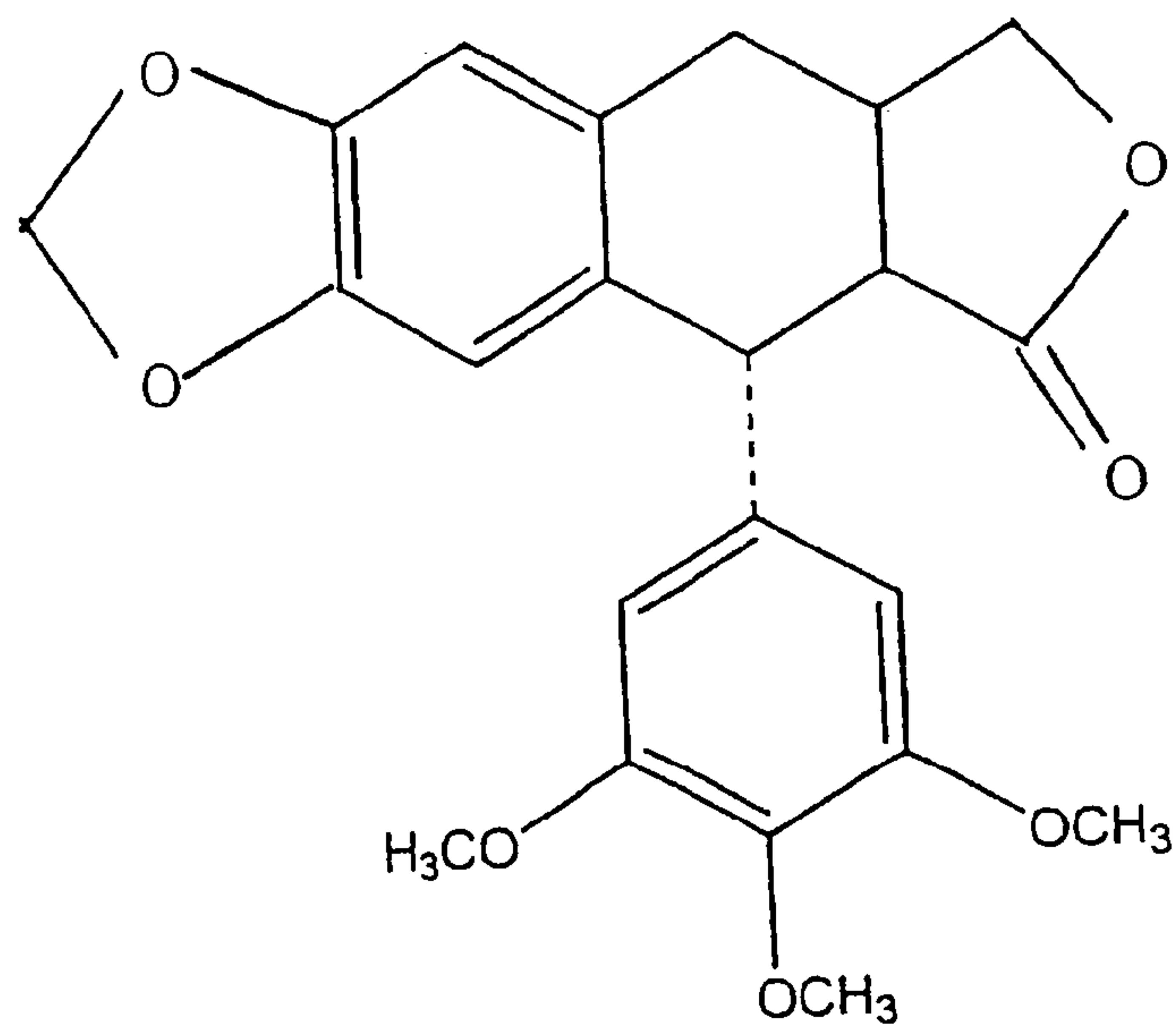
Deoxypicropodophyllin
