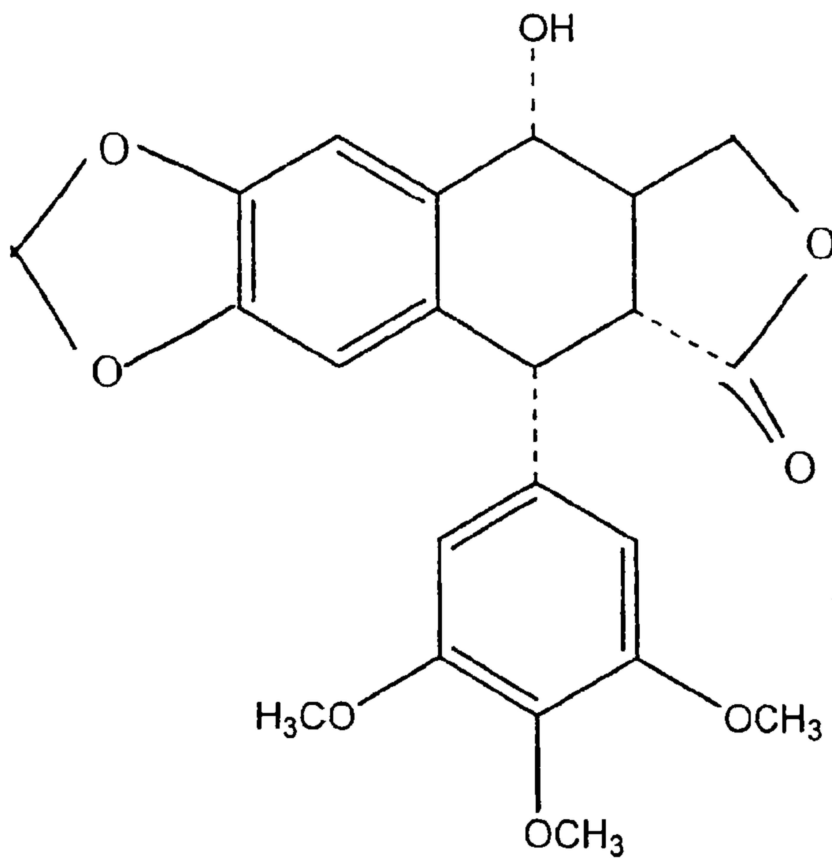
Podophyllotoxin
