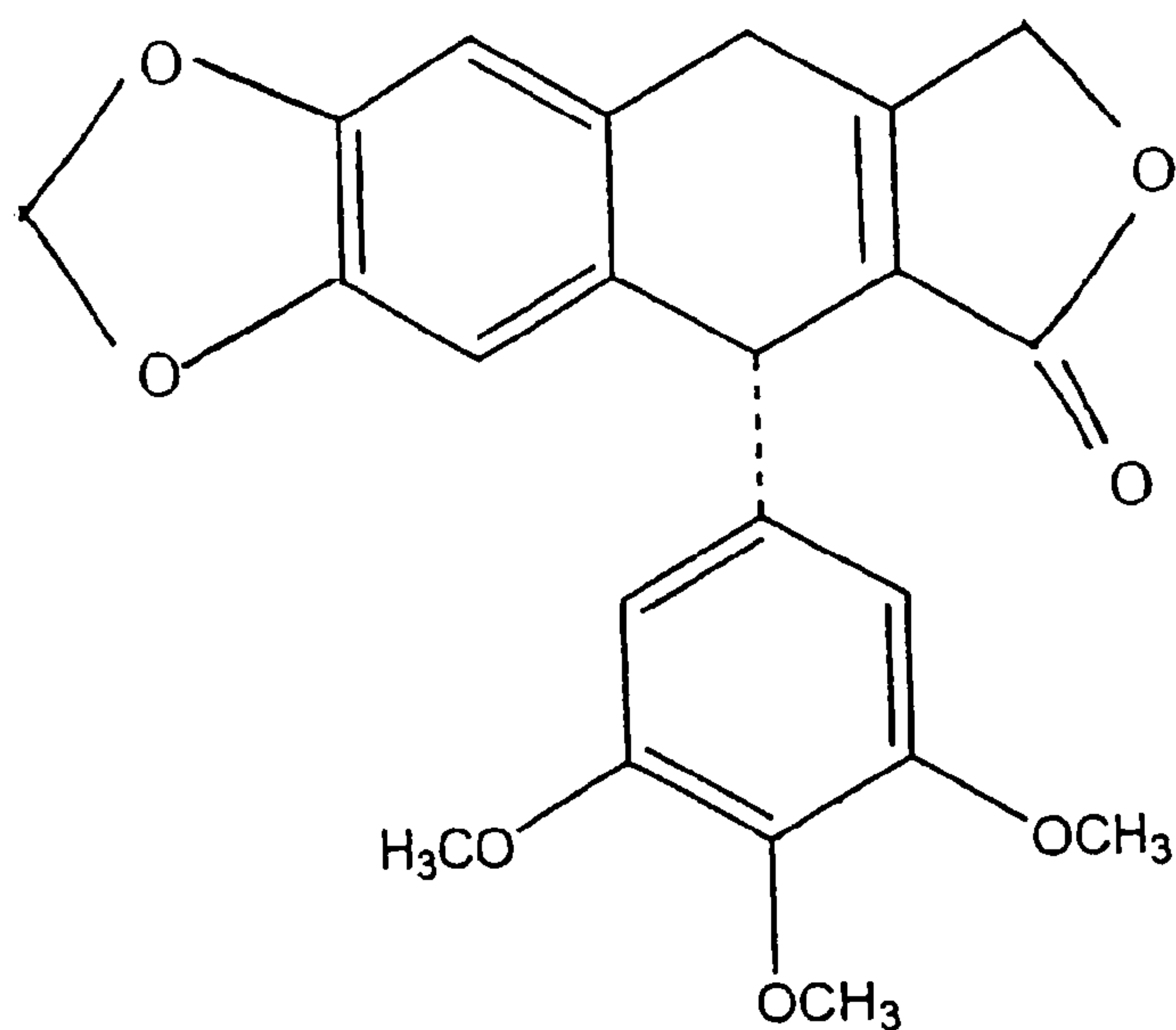
\beta -apopicropodophyllin
