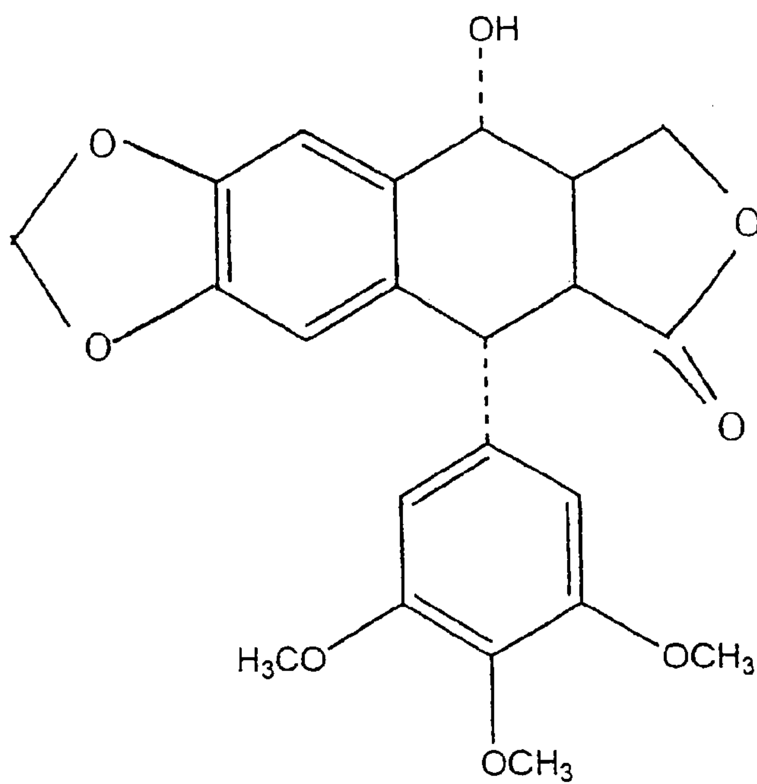
Picropodophyllin
