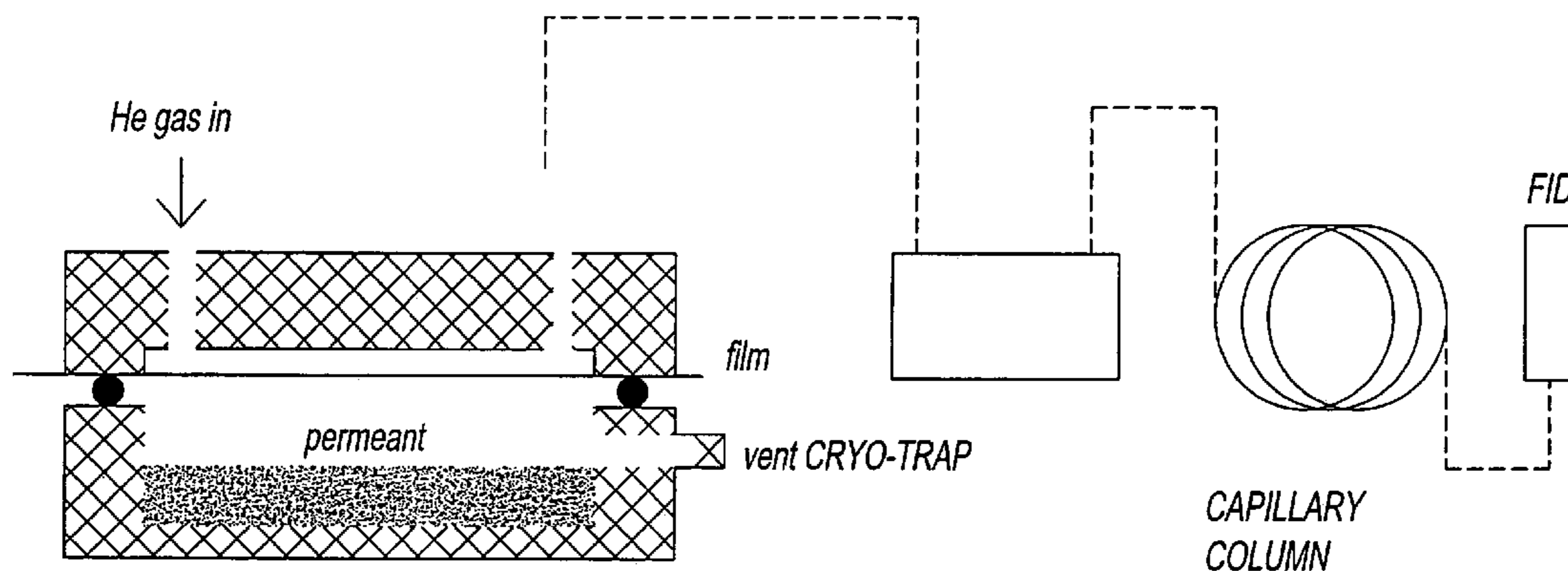
Cell set-up for isostatic permeation test.
