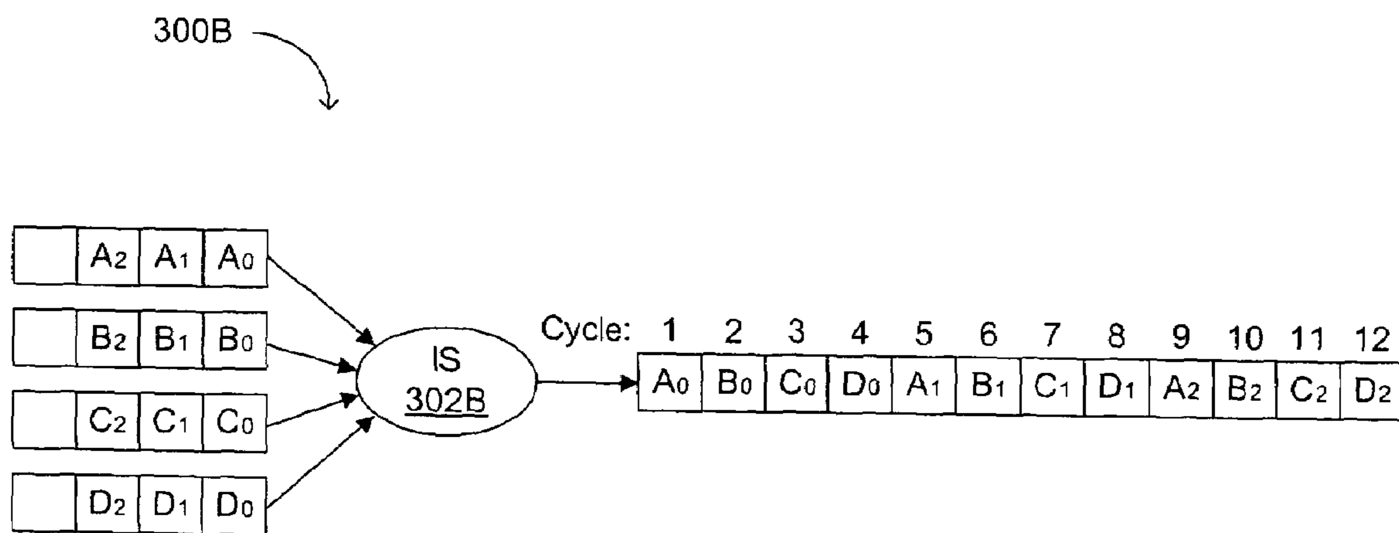
FIG. 3B (conventional)
