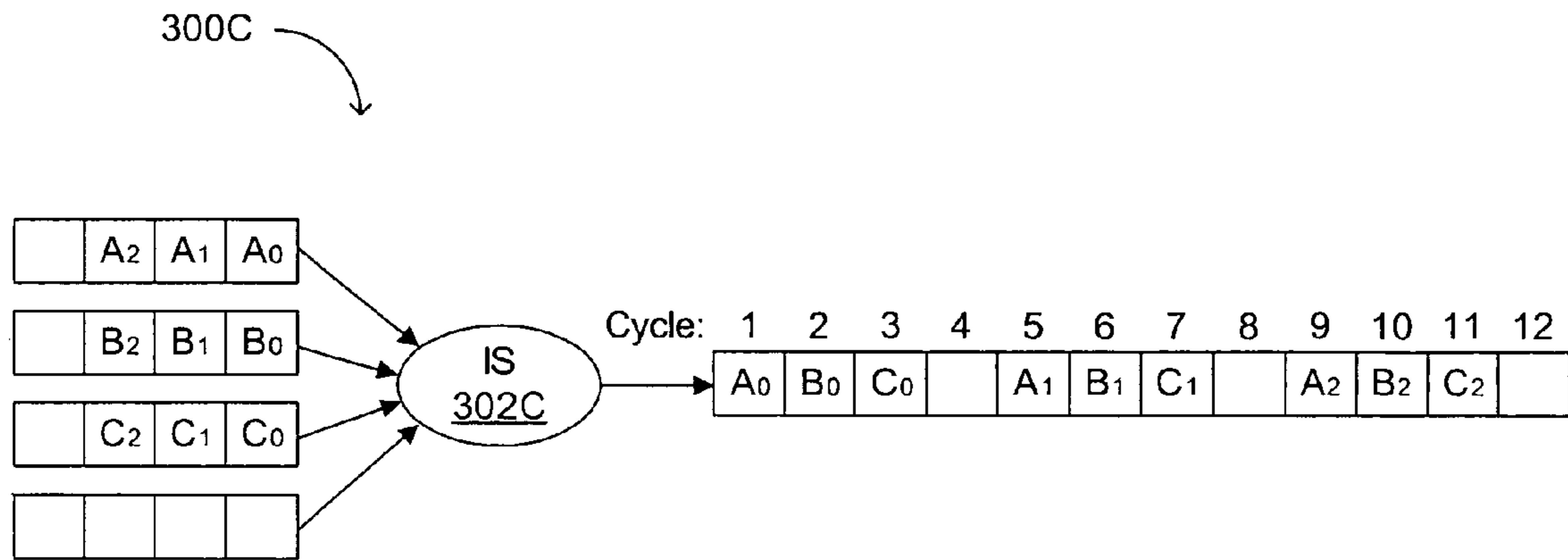
FIG. 3C (conventional)
