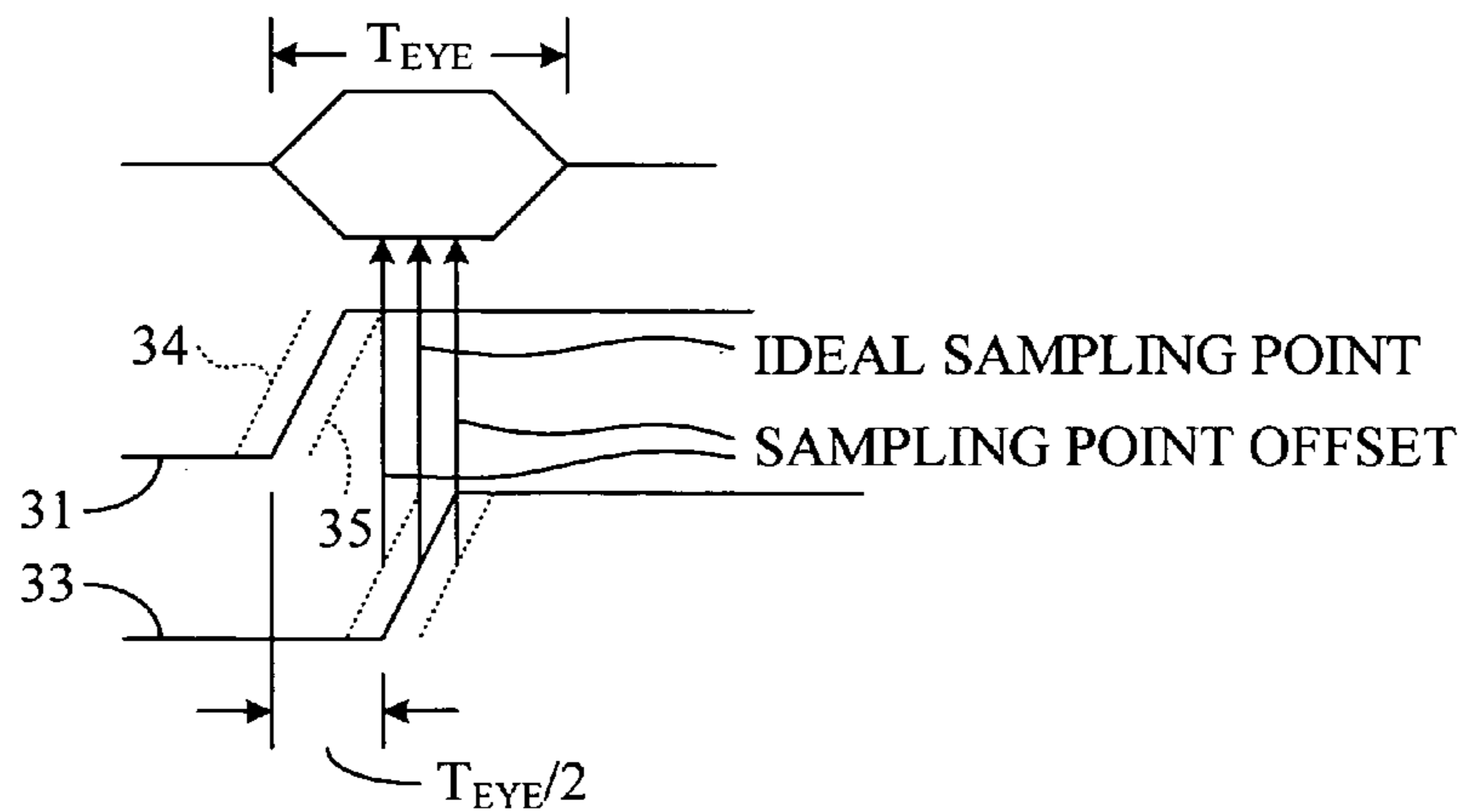
FIG. 2 (Prior Art)
