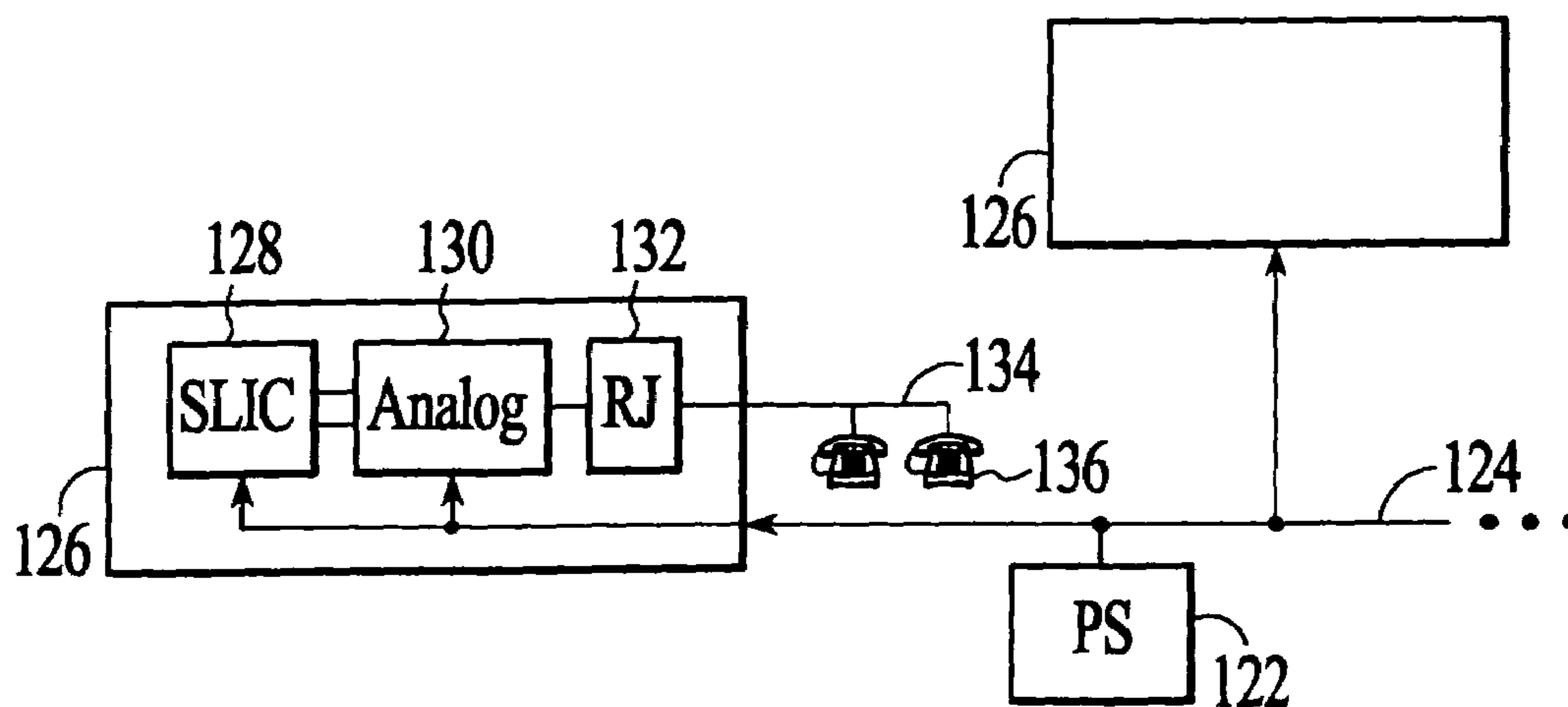
FIG. 7 (PRIOR ART)
