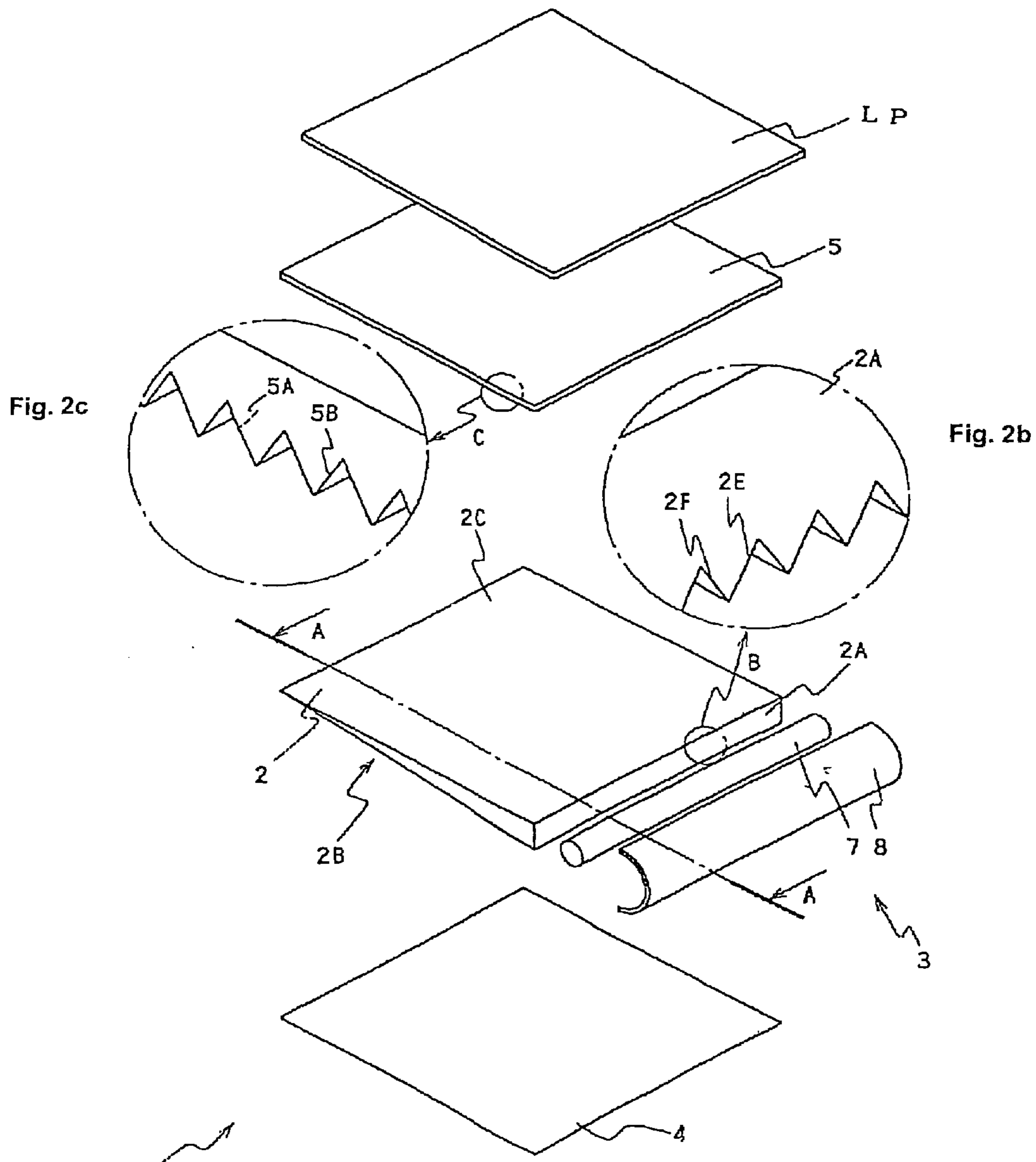
1: SURFACE LIGHT SOURCE DEVICE OF SIDE LIGHT TYPE
