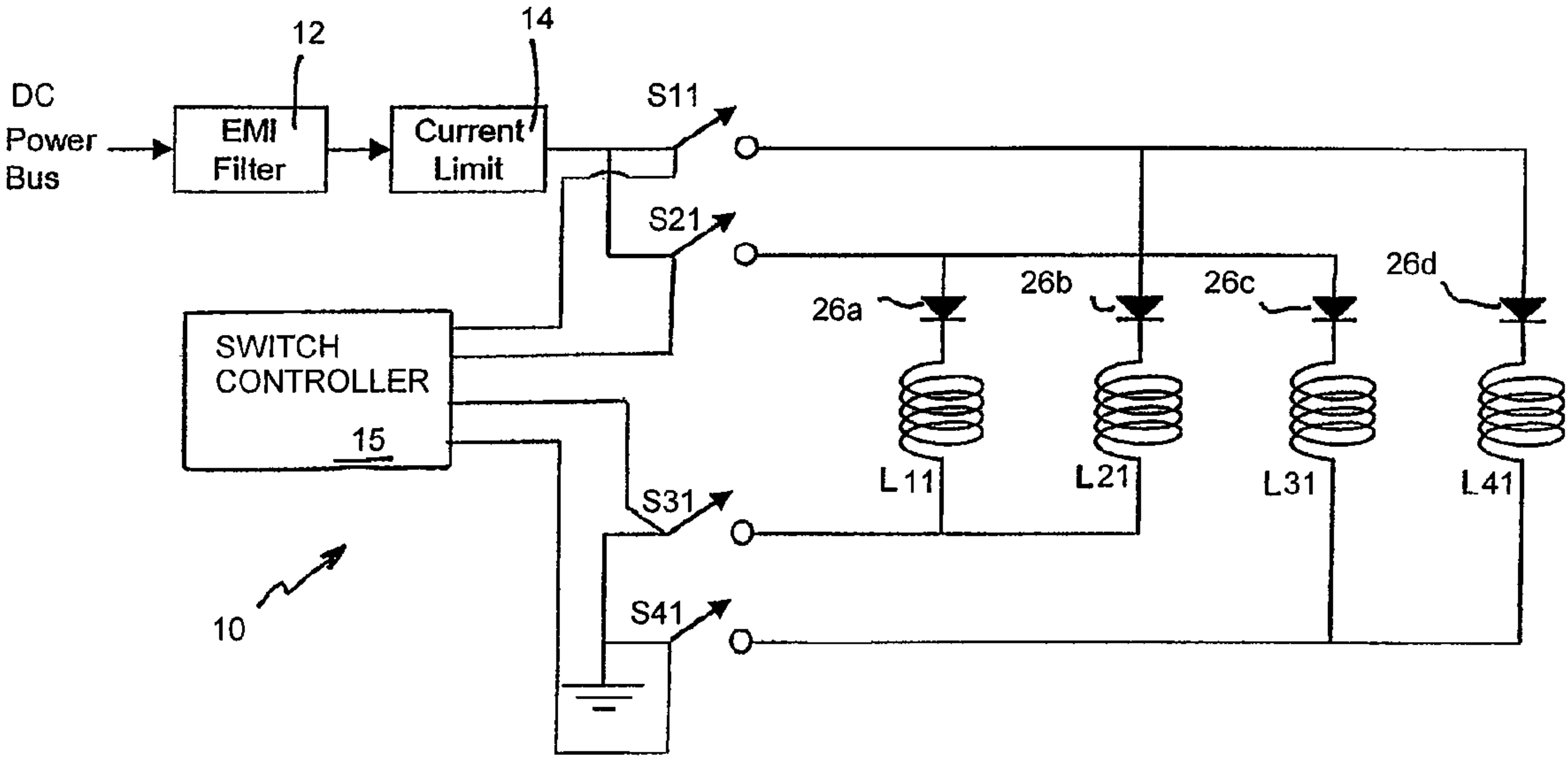
FIG. 1 (Prior Art)
