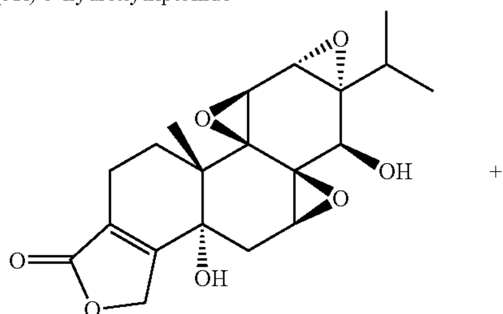
(5R)-5-hydroxytriptolide
