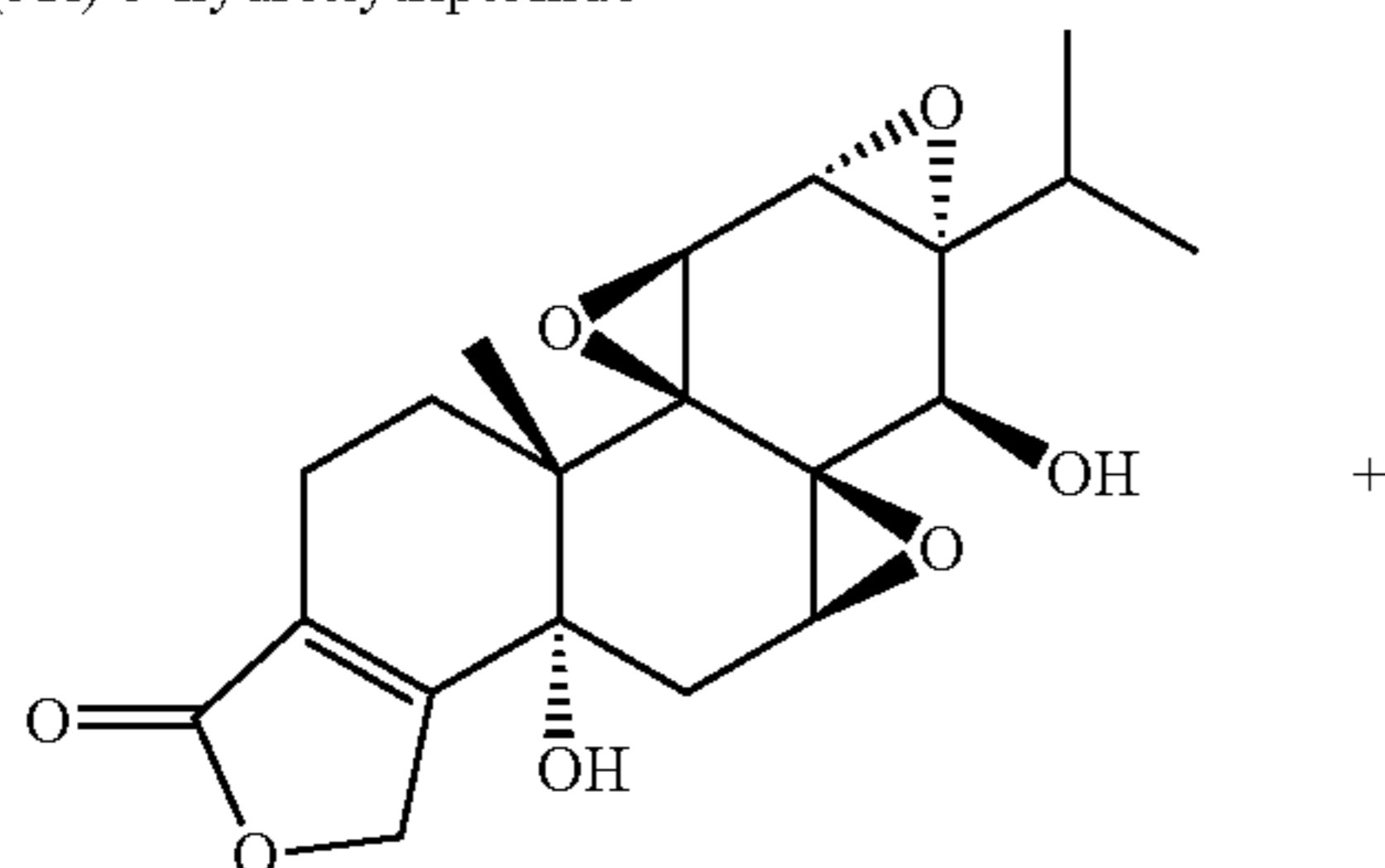
(5R)-5-hydroxytriptolide
