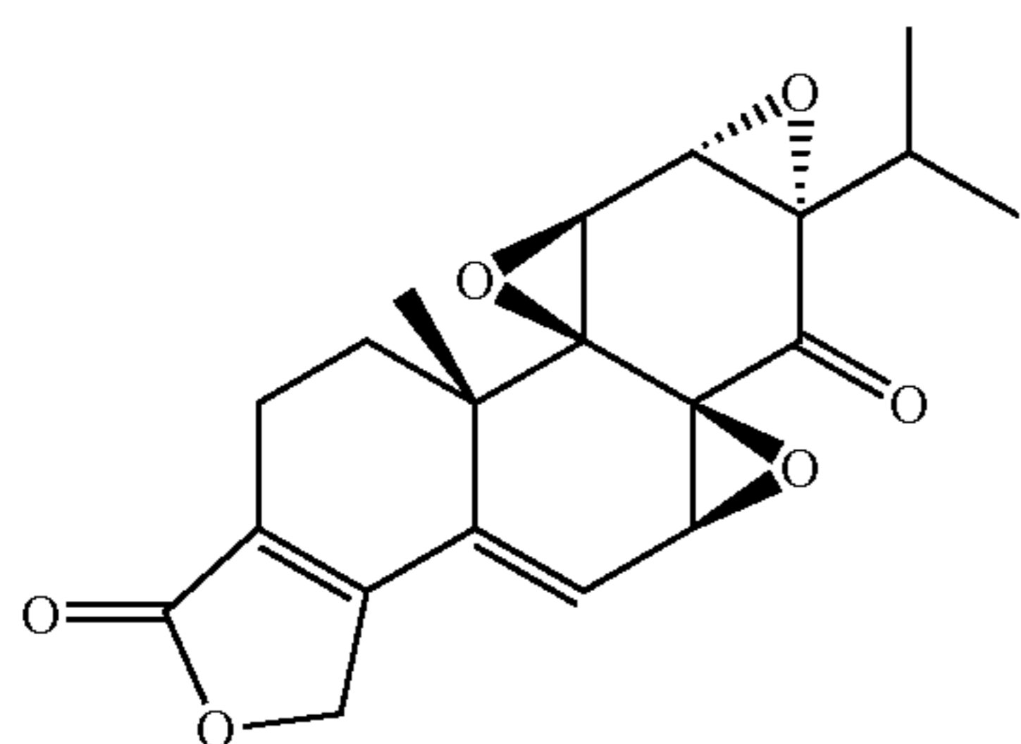
\Delta^{5,6} -dehydrotriptonide
