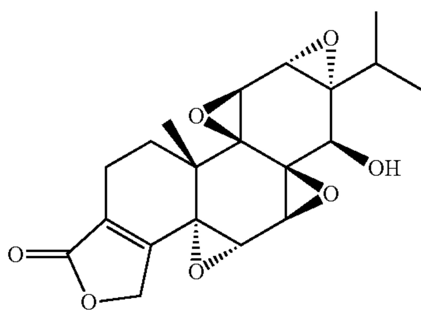
(5R,6S)-5,6-epoxytriptolide
