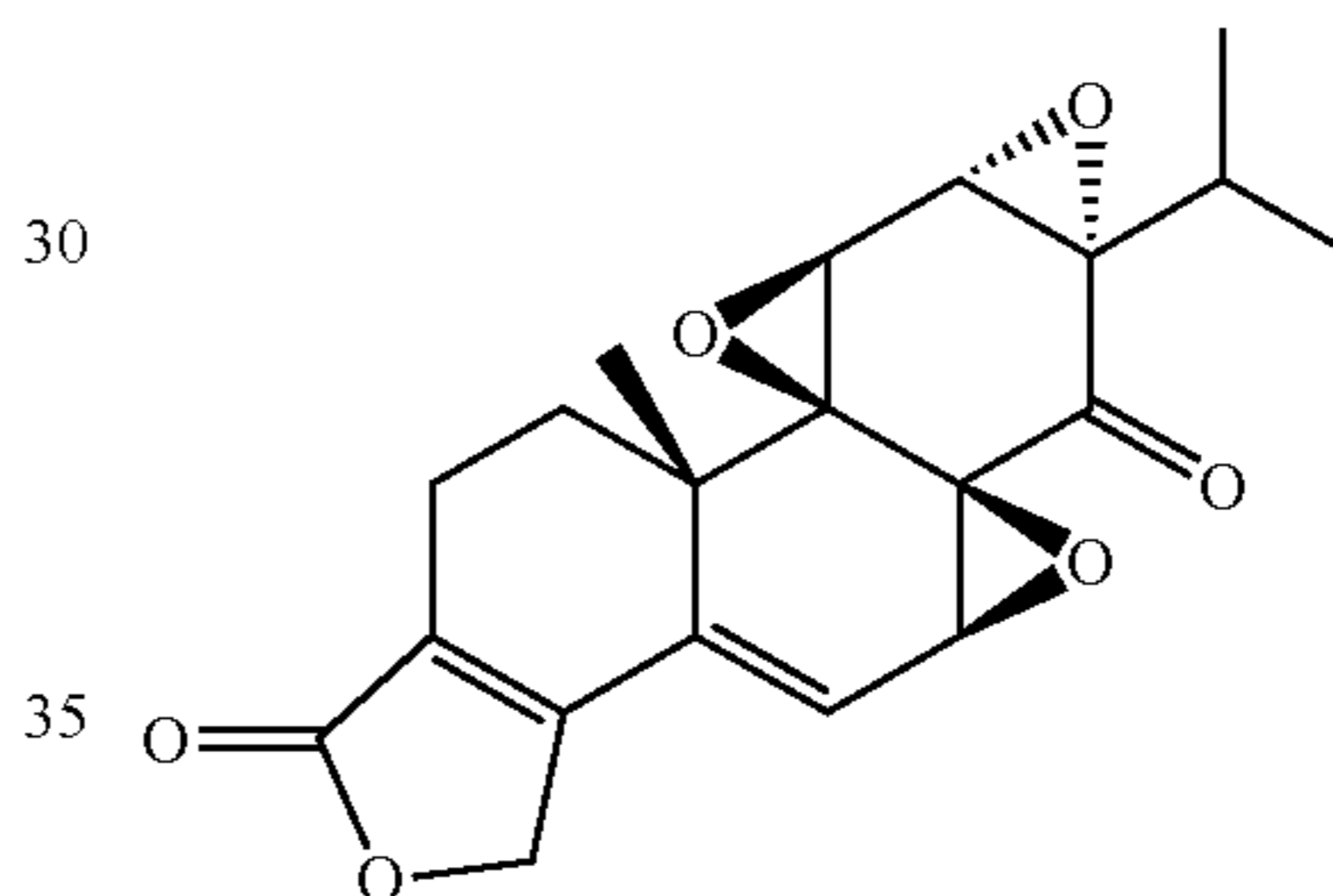
\Delta^{5,6} -dehydrotriptonide
