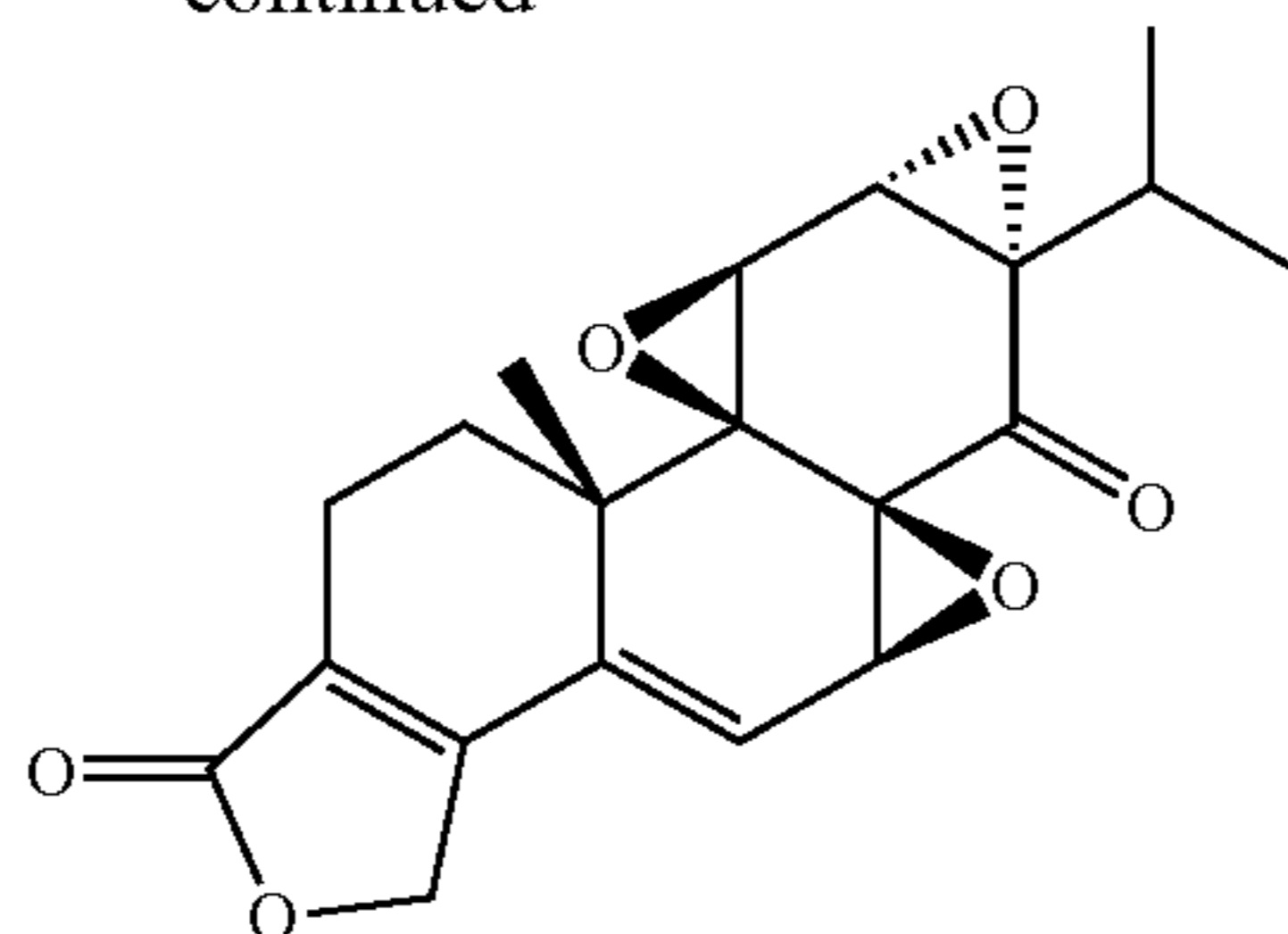
\Delta^{5,6} -dehydrotriptonide
