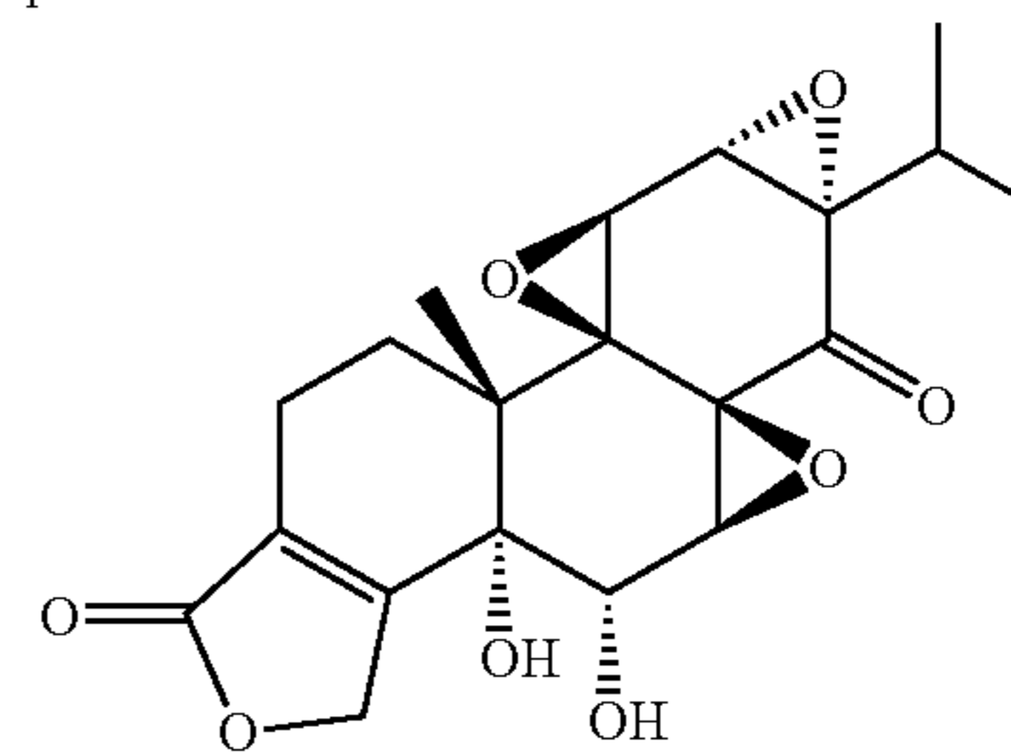
cis-(5R,6S)-5,6-dihydroxytriptonide
