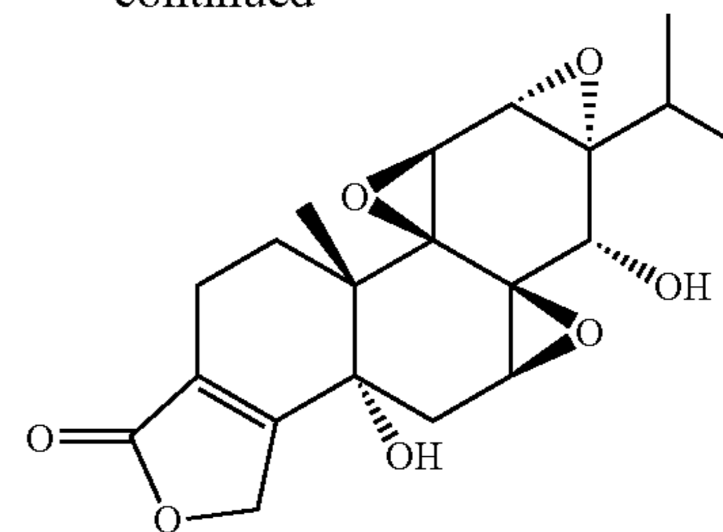
(5R)-5-hydroxy-14-epitriptolide
