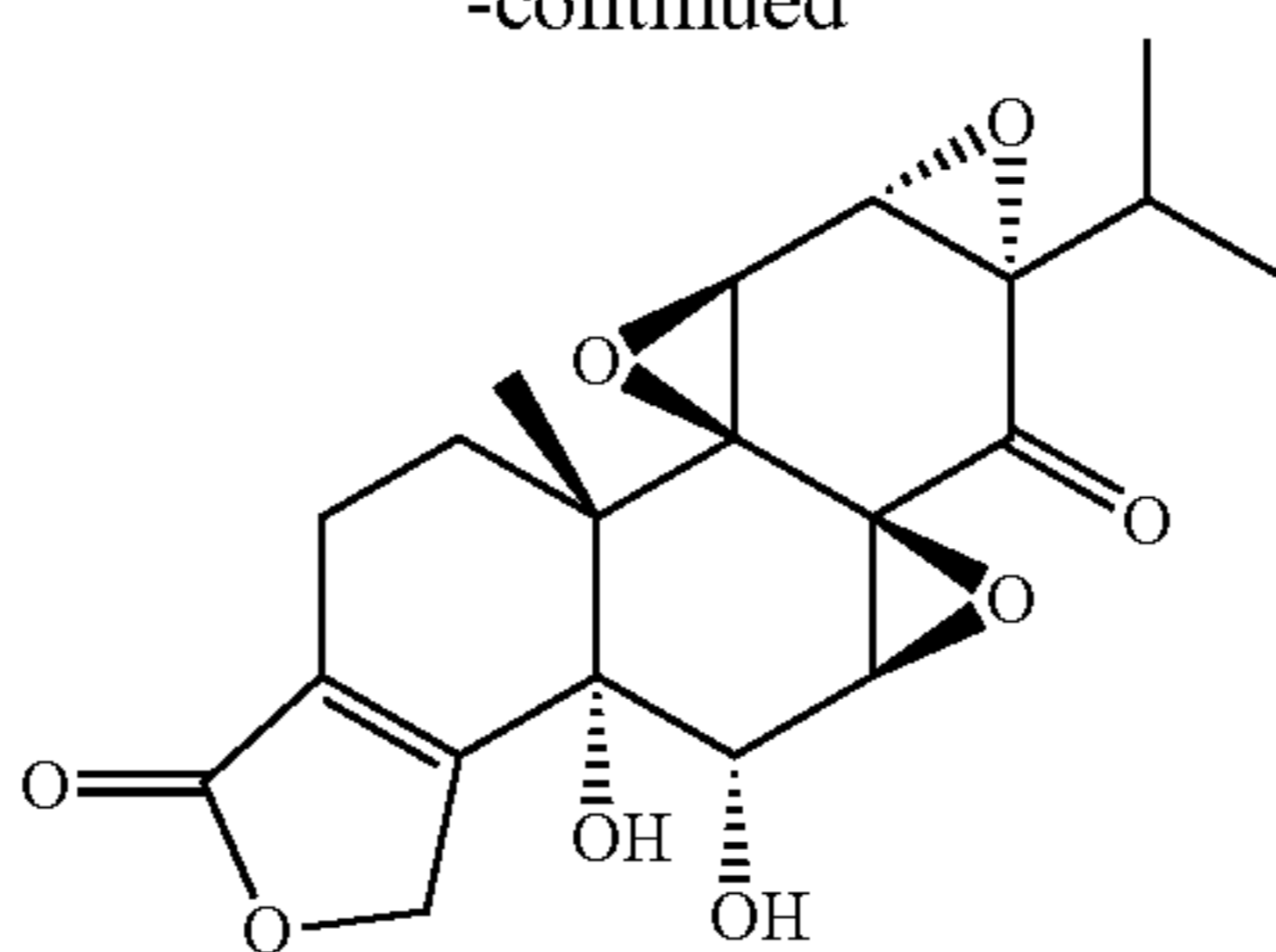
cis-(5R,6S)-dihydroxytriptonide
