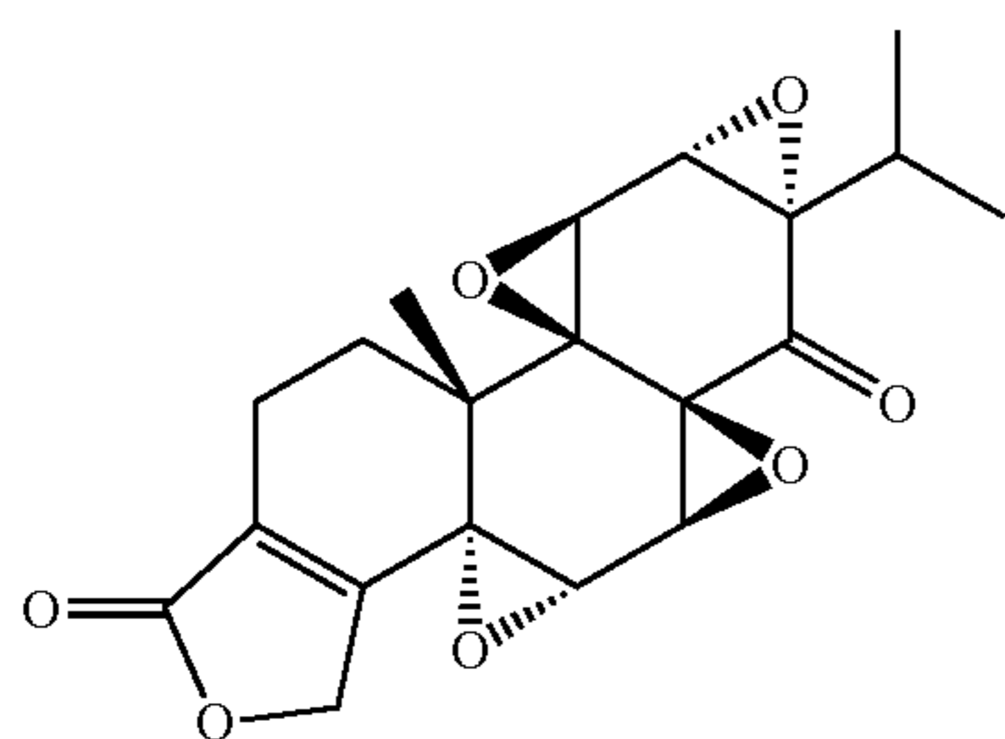
(5R,6S)-5,6-epoxytriptonide
