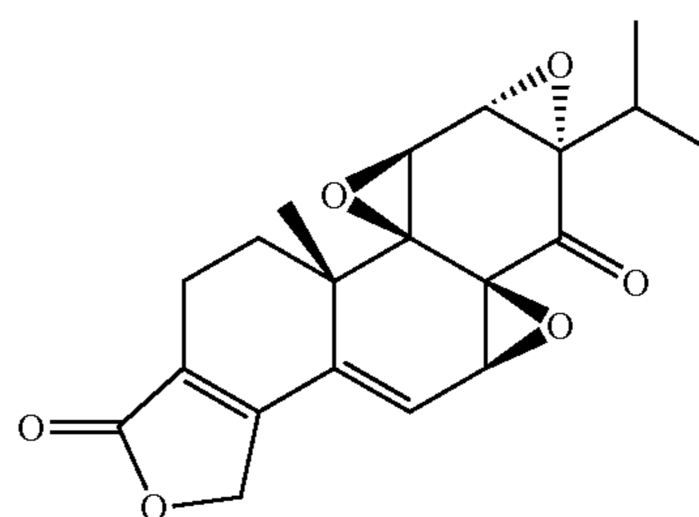
\Delta^{5,6} -dehydrotriptonide
