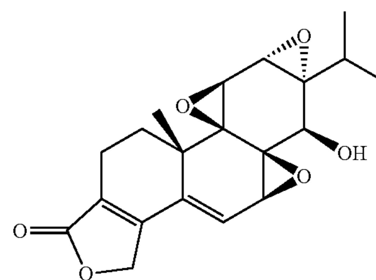
\Delta^{5,6} -dehydrotriptonide
