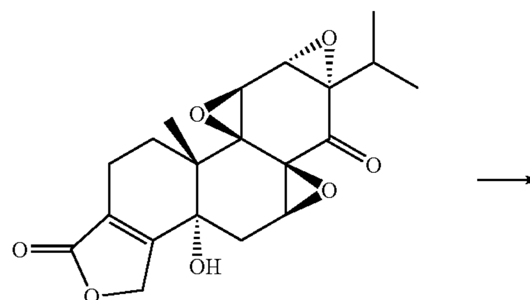
(5R)-5-hydroxytriptonide
