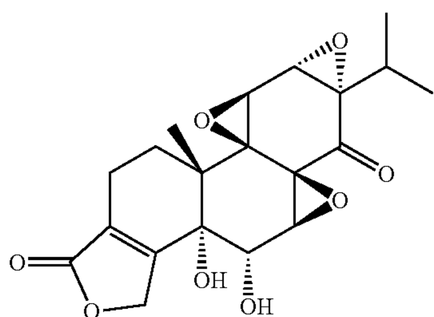
cis-(5R,6S)-5,6-dihydroxytriptonide
