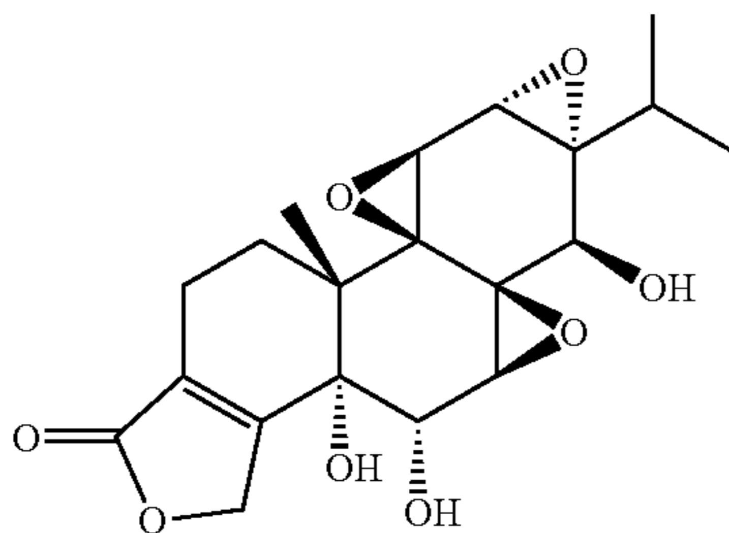
cis-(5R,6S)-5,6-dihydroxytriptolide
