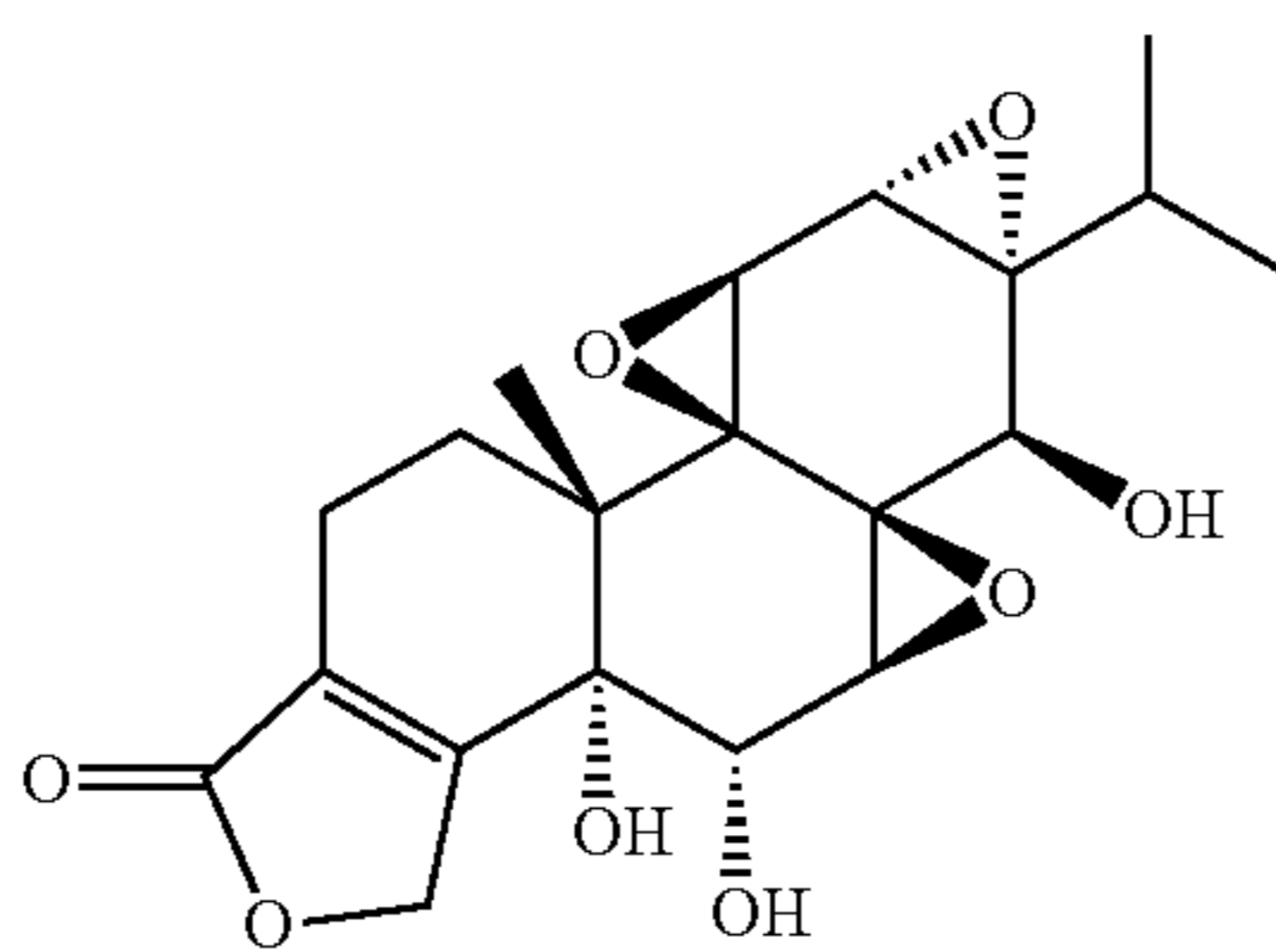
cis-(5R,6S)-5,6-dihydroxytriptolide
