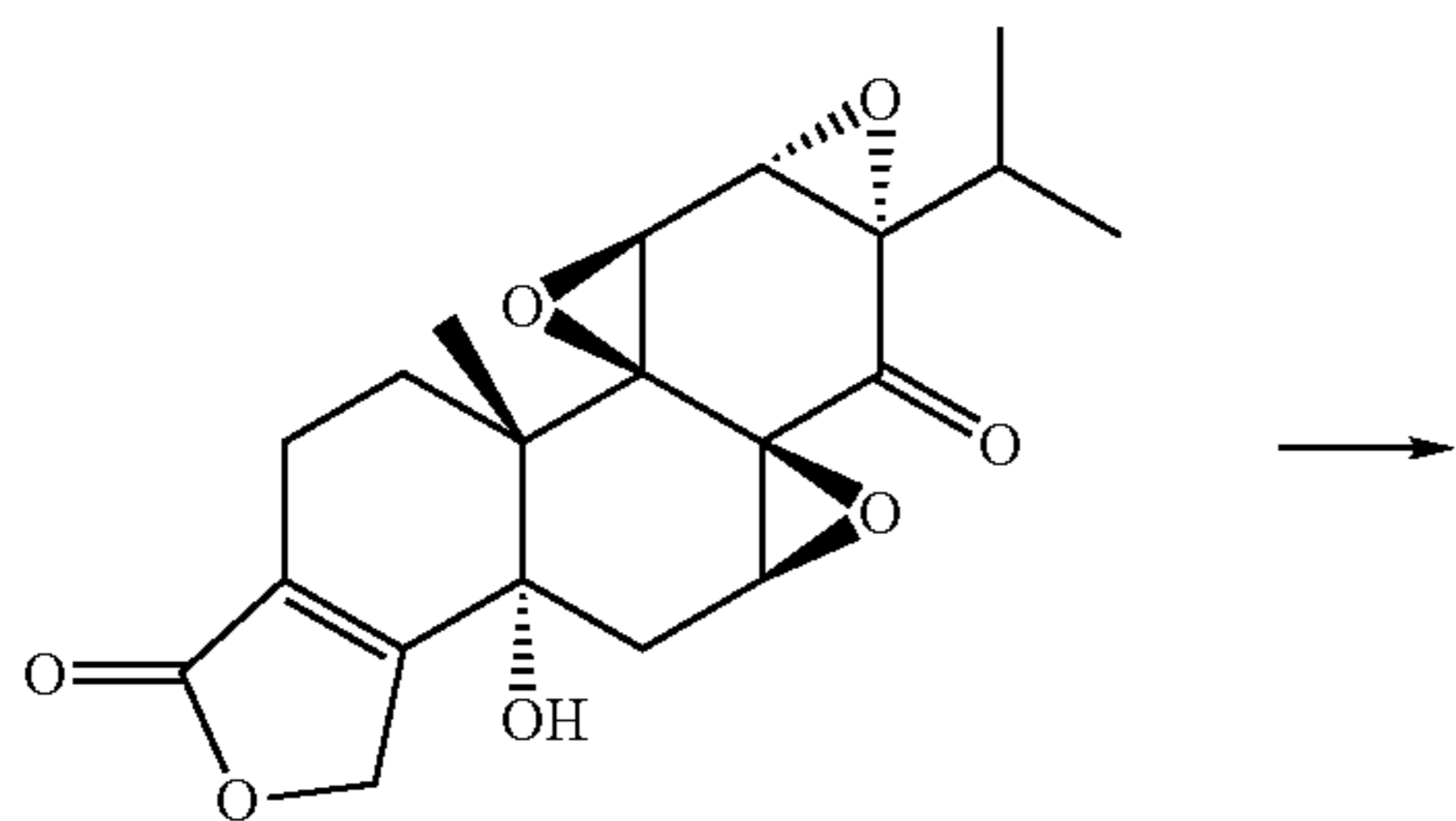
(5R)-5-hydroxytriptolide
