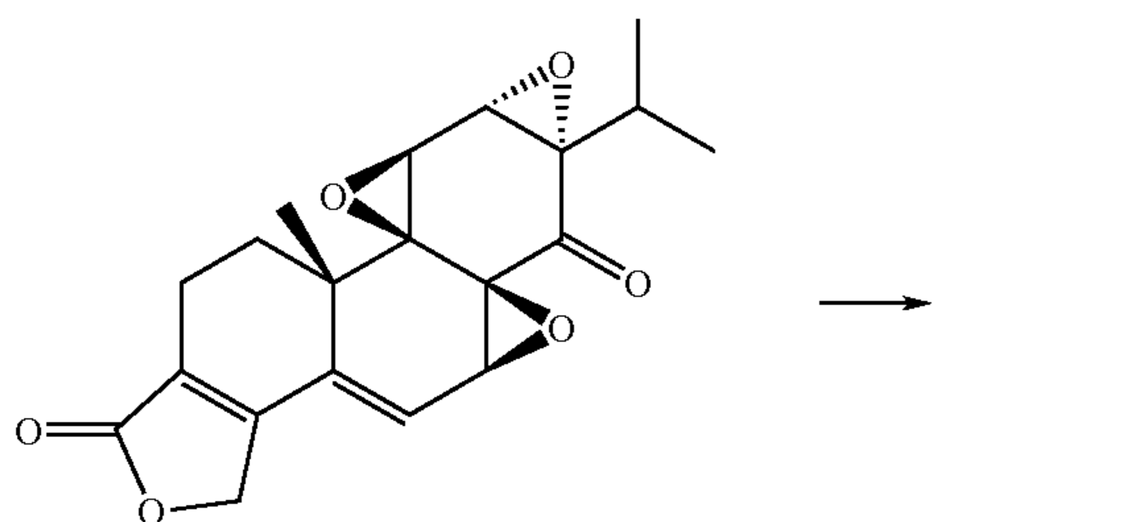
\Delta^{5,6} -dehydrotriptonide
