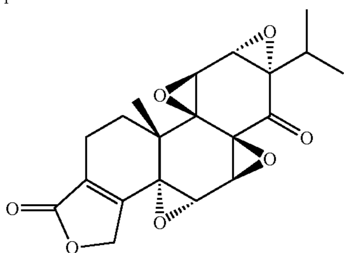
(5R,6S)-5,6-epoxytriptonide
