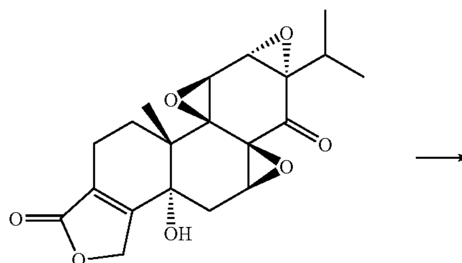
(5R)-5-hydroxytriptonide
