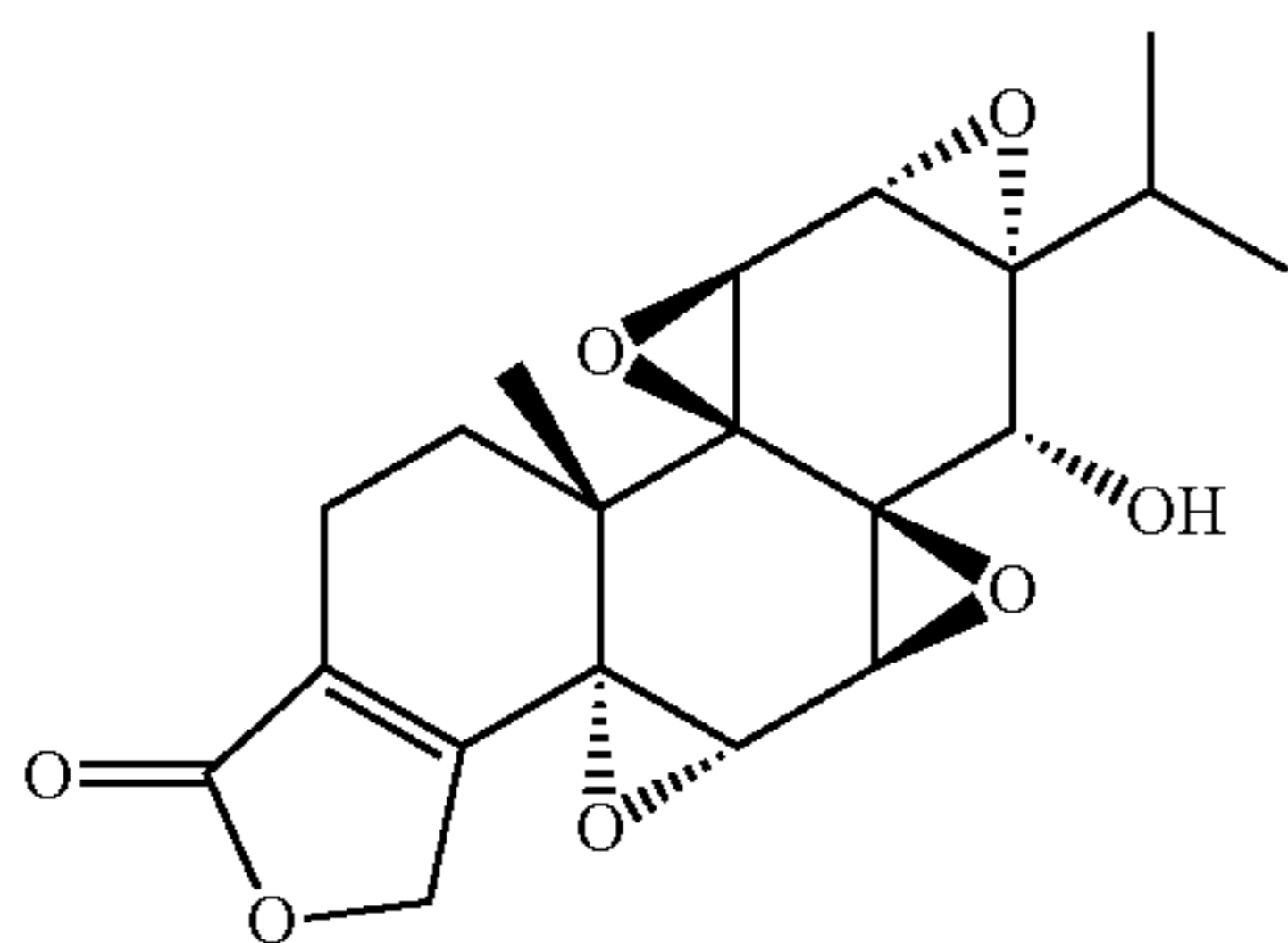
(5R,6S)-5,6-epoxy-14-epitriptolide
