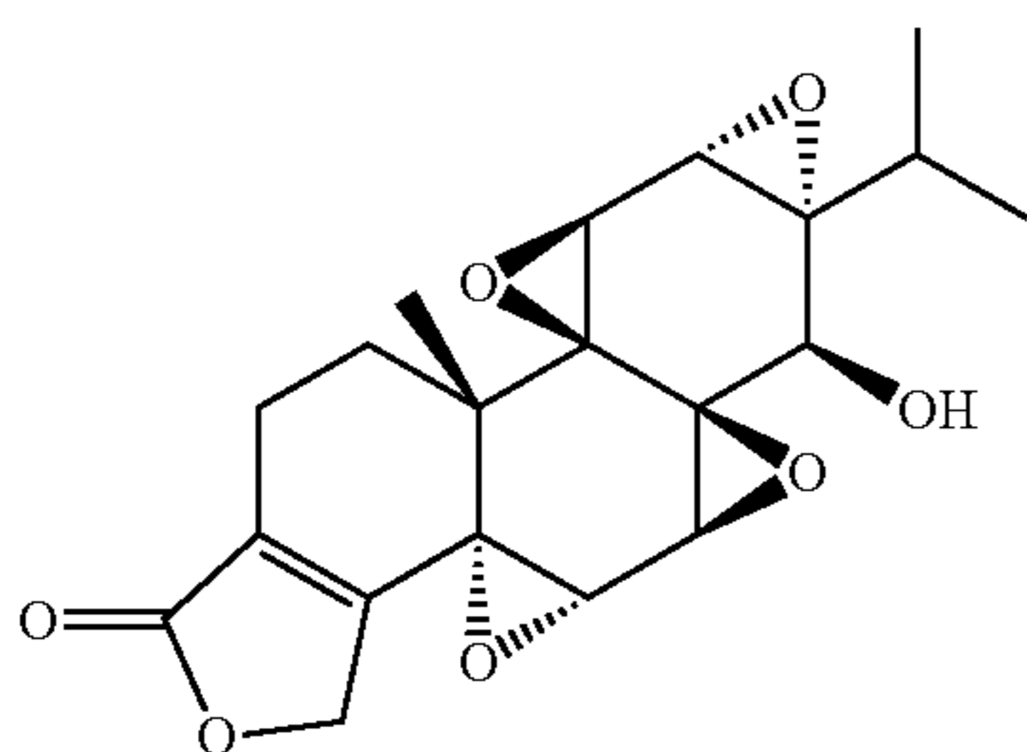
(5R,6S)-5,6-epoxytriptolide
