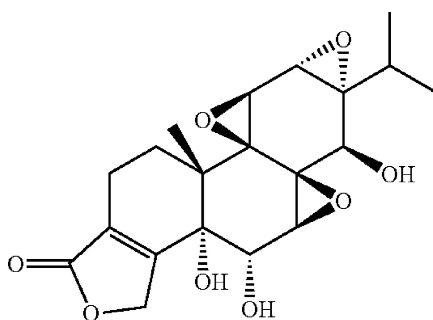
cis-(5R,6S)-5,6-dihydroxytriptolide
