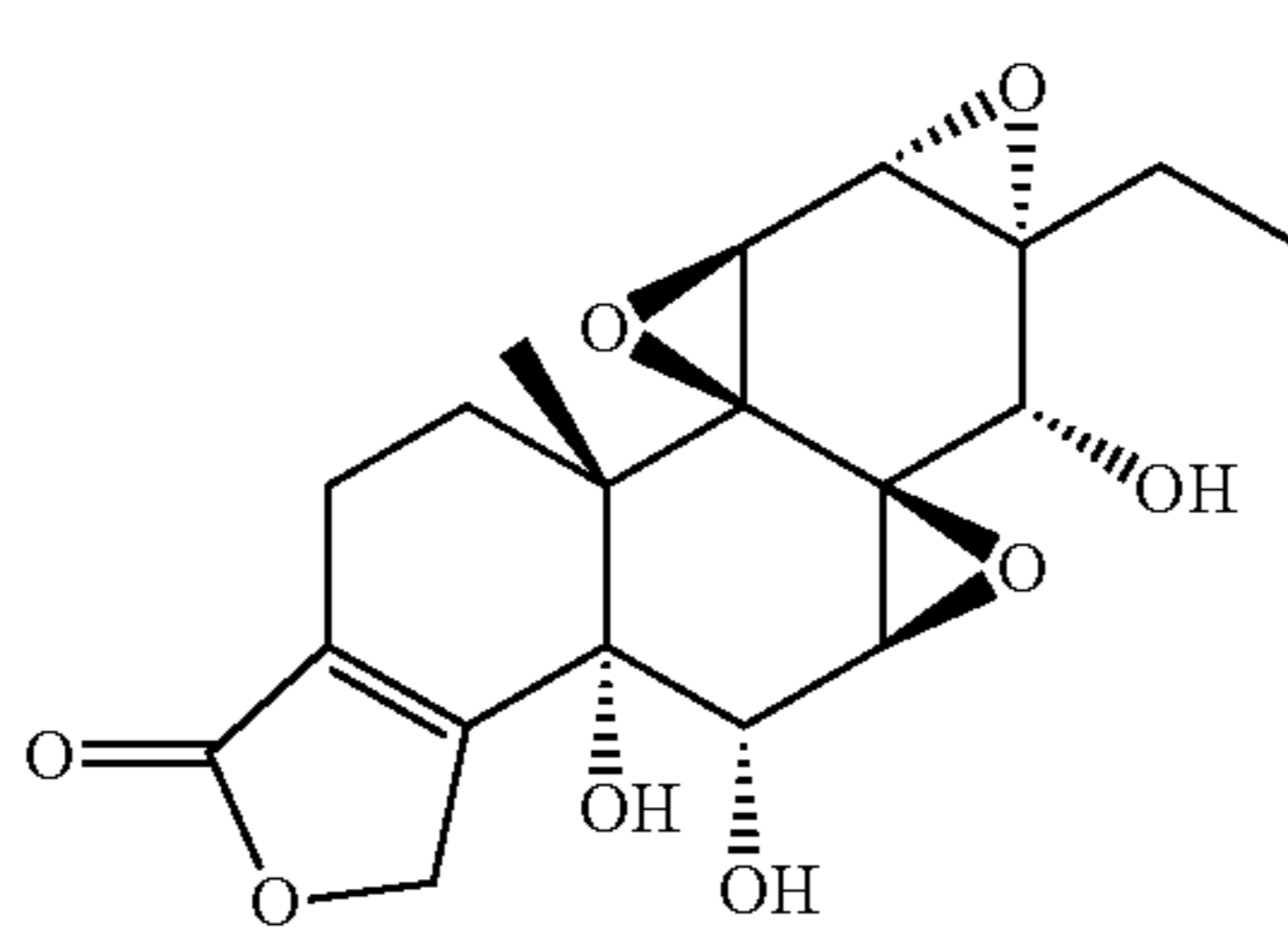
cis-(5R,6S)-5,6-dihydroxy-14-epitriptolide
