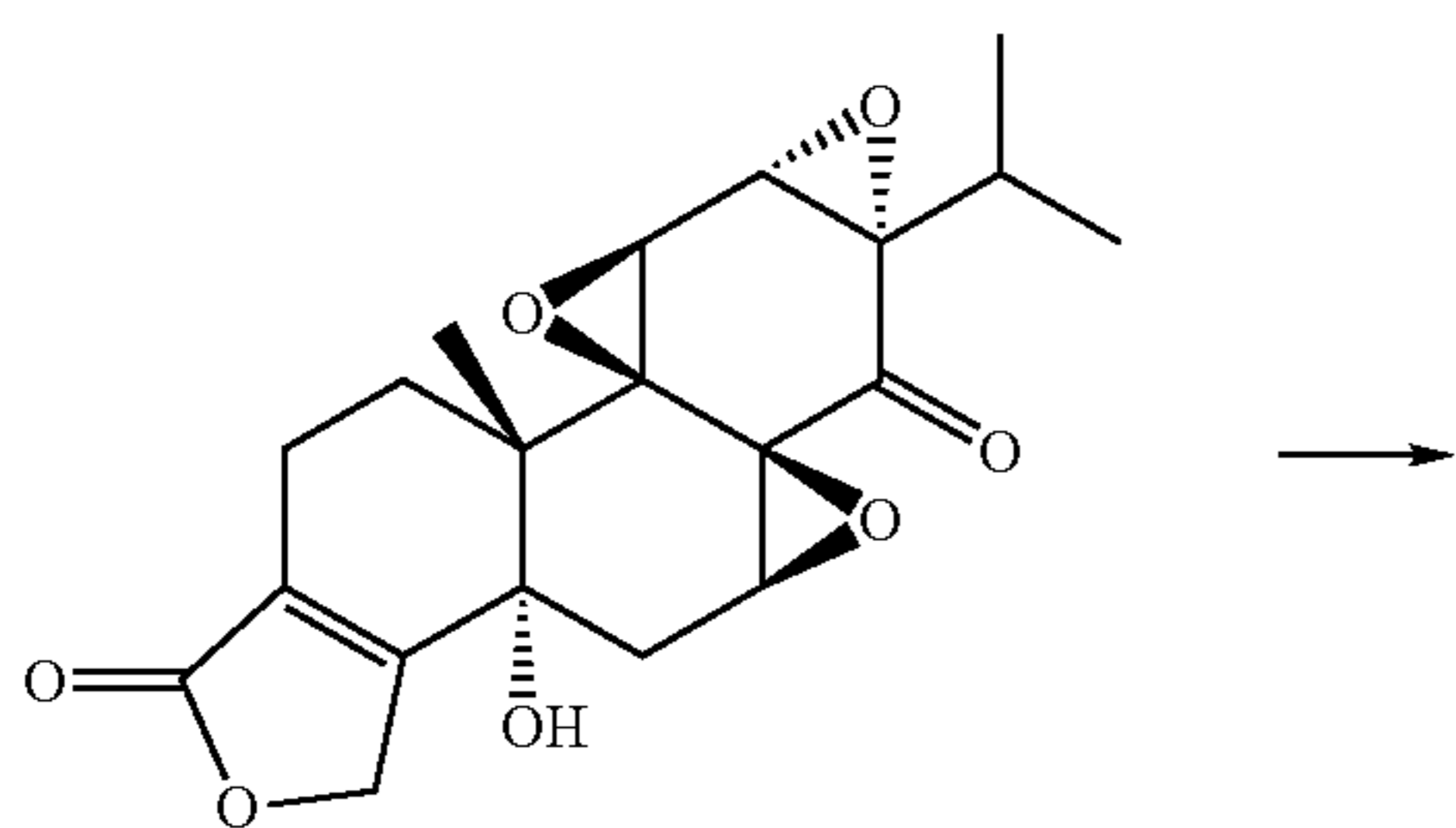
(5R)-5-hydroxytriptolide
