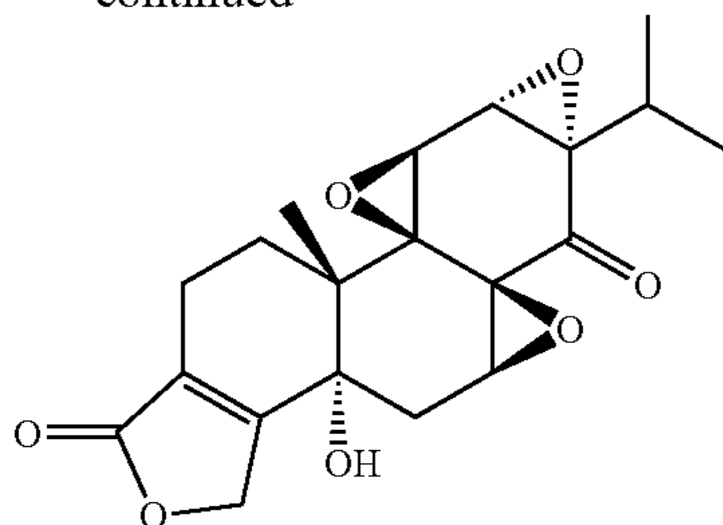
(5R)-5-hydroxytriptonide
