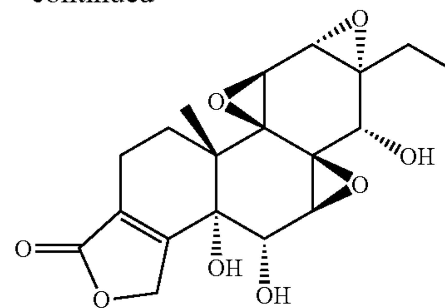
cis-(5R,6S)-5,6-dihydroxy-14-epitriptolide
