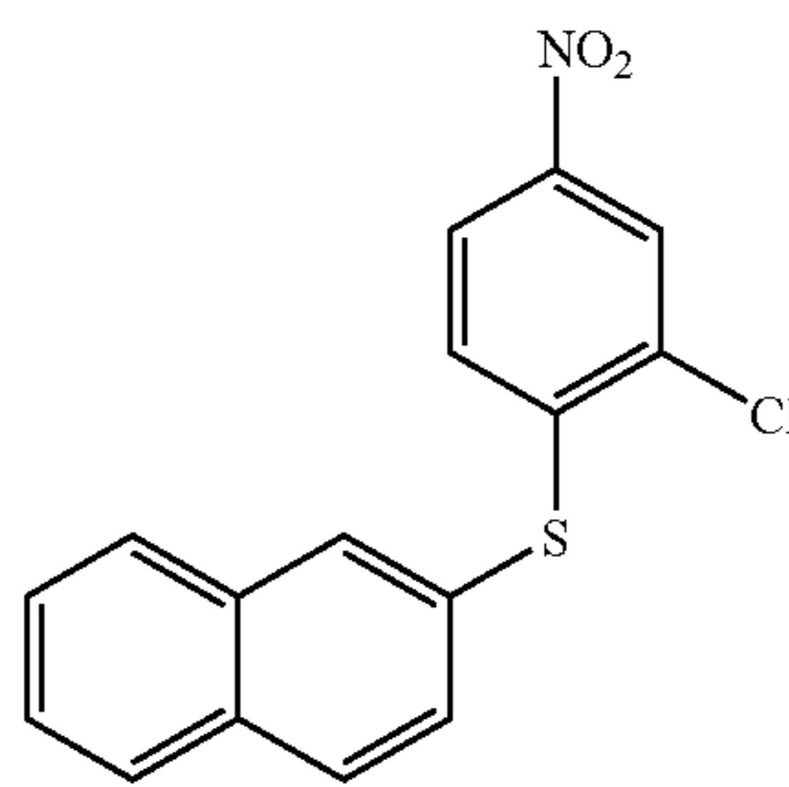
2-(2-Chloro-4-nitro-phenylsulfanyl)-naphthalene (91)
