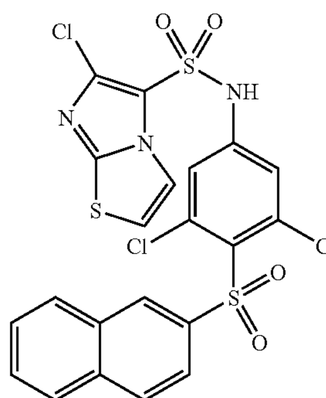
Chloro-imidazo[2,1-b]thiazole-5-sulfonic acid [3,5-dichloro-4-(naphthalen-2-ylsulfanyl)-phenyl]-amide (102)
