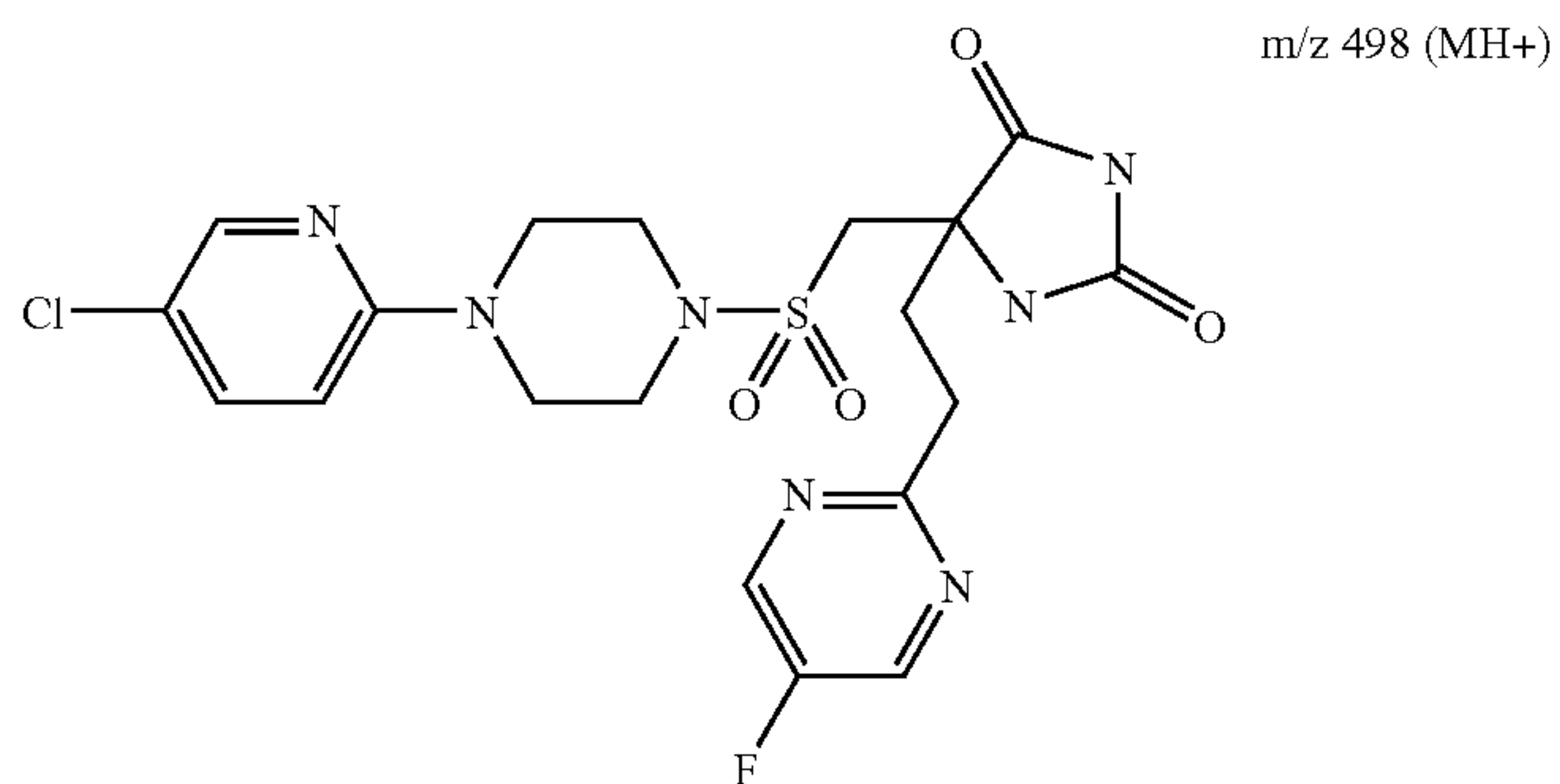
5-[4-(5-Chloro-pyridin-2-yl)-piperazine-1-sulfonylmethyl]-5-[2-(5-fluoro-pyrimidin-2-yl)-ethyl]-imidazolidine-2,4-dione
