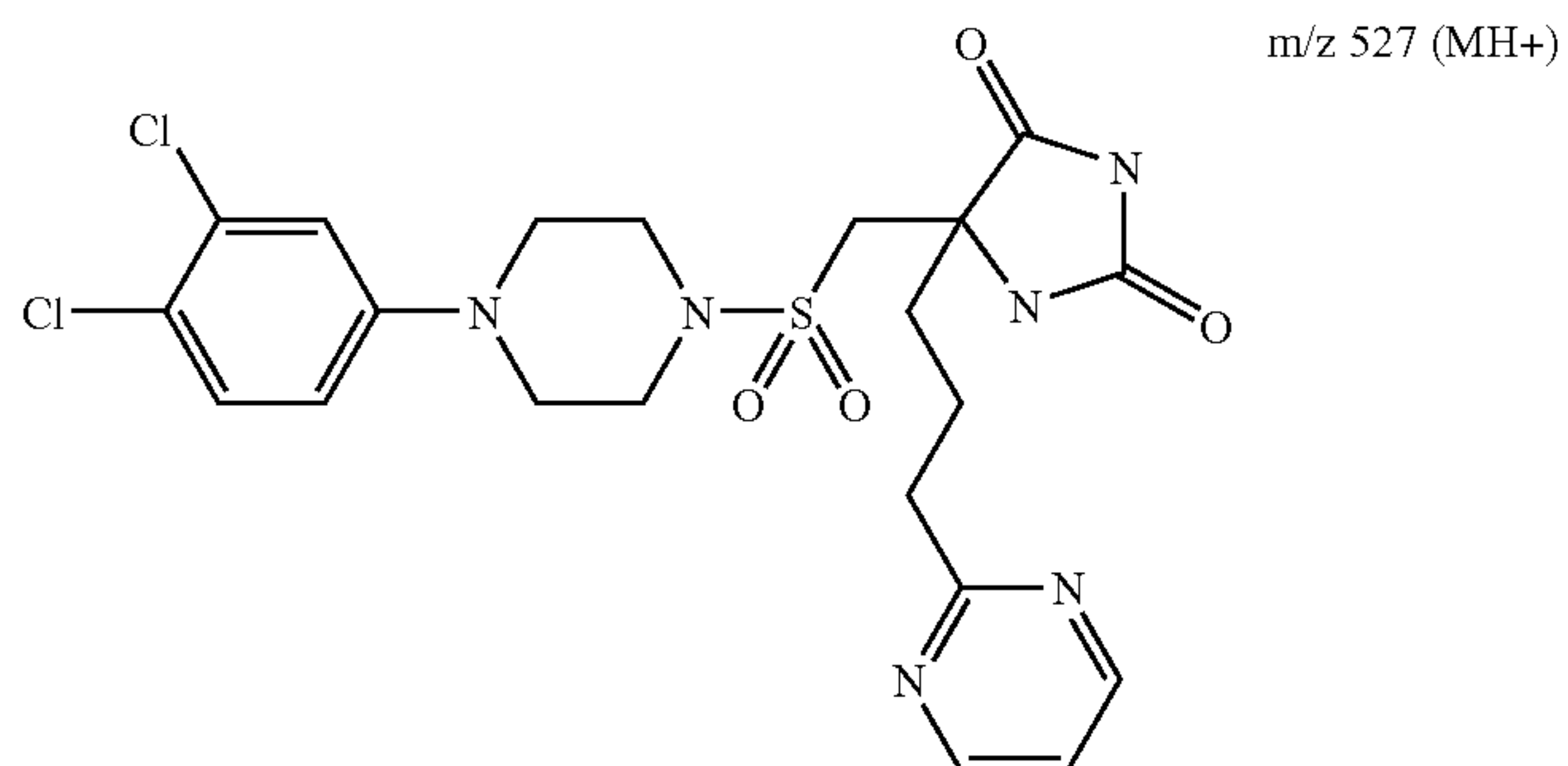
5-[4-(3,4-Dichloro-phenyl)-piperazine-1-sulfonylmethyl]-5-(3-pyrimidin-2-yl-propyl)-imidazolidine-2,4-dione
