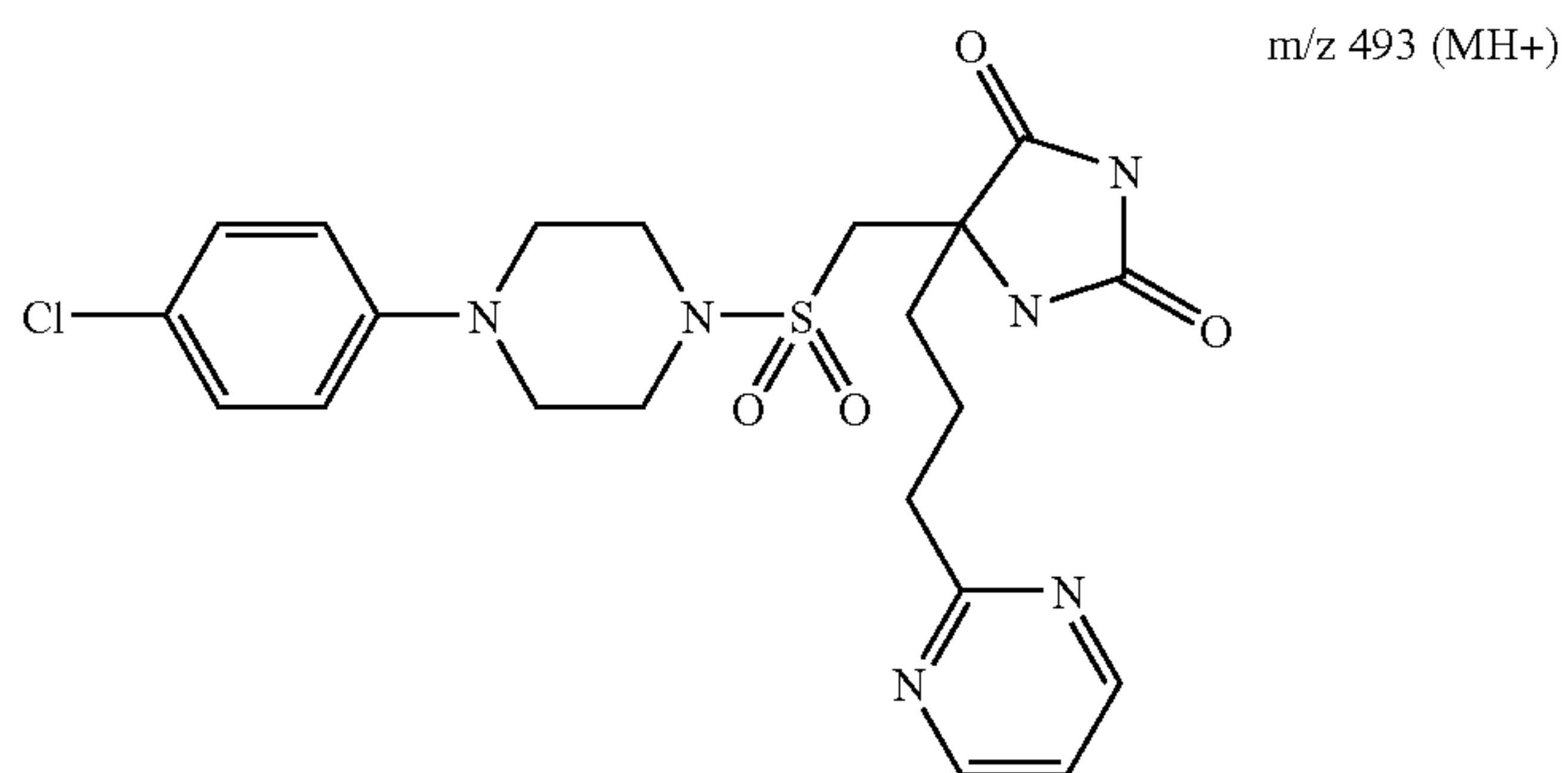
5-[4-(4-Chloro-phenyl)-piperazine-1-sulfonylmethyl]-5-(3-pyrimidin-2-yl-propyl)-imidazolidine-2,4-dione
