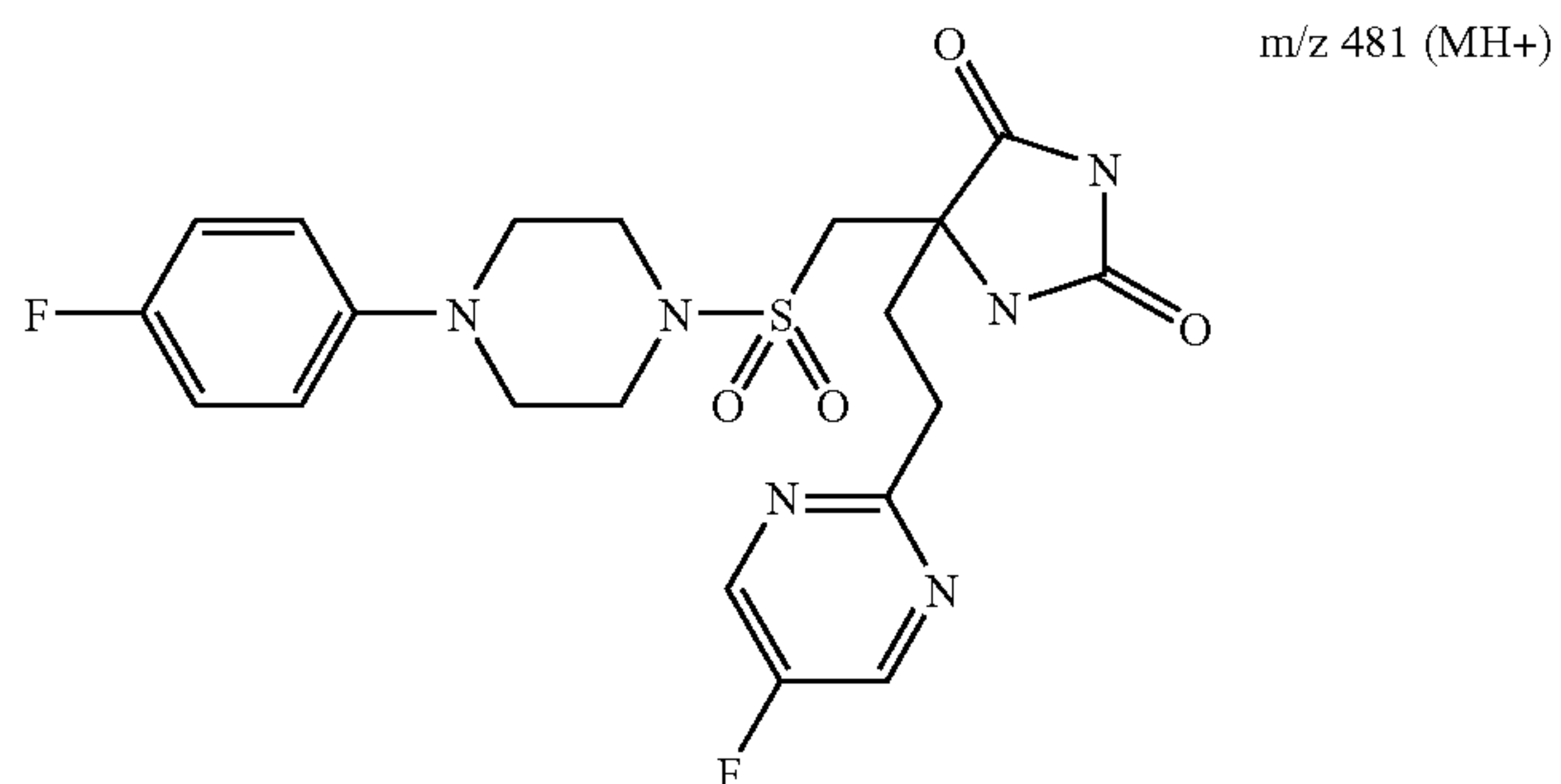
5-[4-(4-Fluoro-phenyl)-piperazine-1-sulfonylmethyl]-5-[2-(5-fluoro-pyrimidin-2-yl)-ethyl]-imidazolidine-2,4-dione
