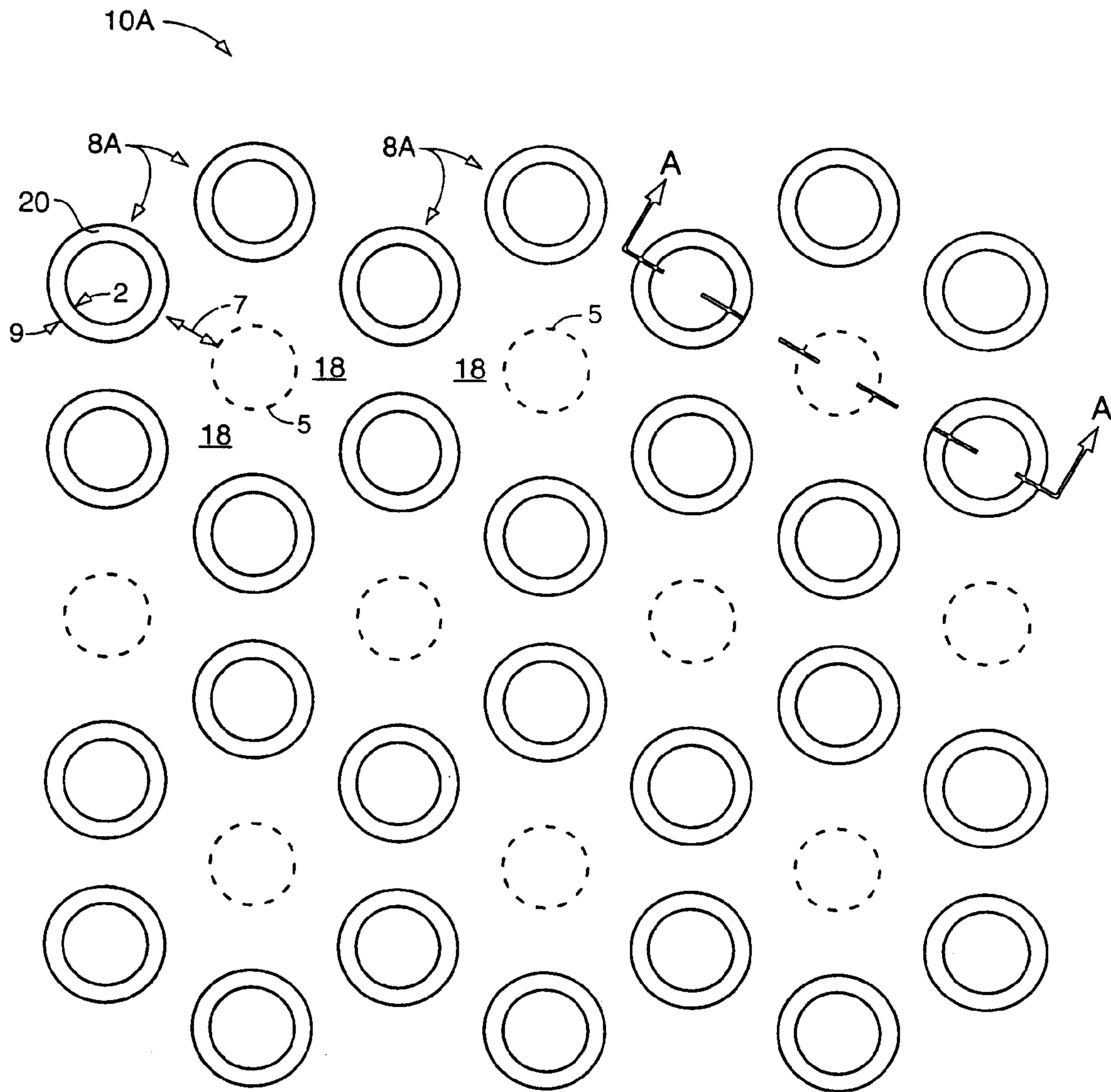
FIG. 1 (PRIOR ART)
