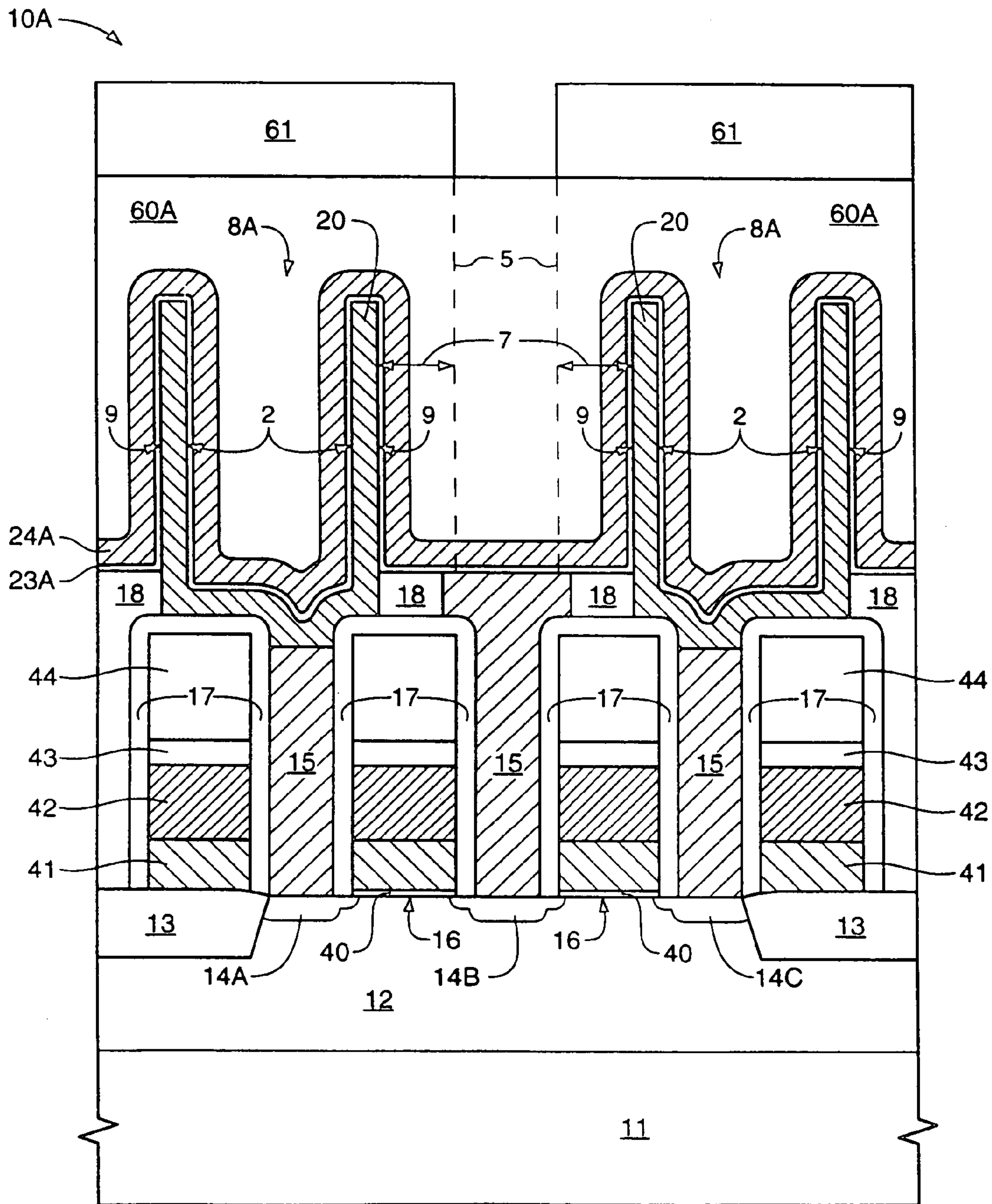
FIG. 2 (PRIOR ART)
