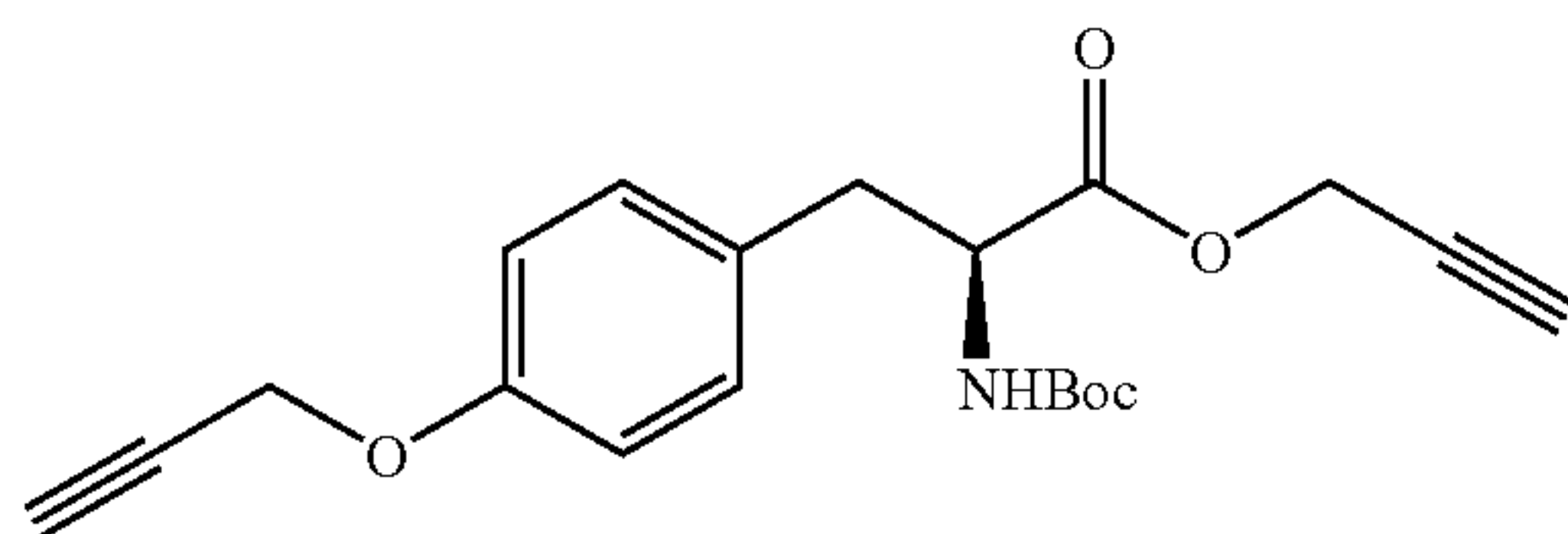
2-tert-Butoxycarbonylamino-3-[4-(prop-2-ynyloxy)phenyl]-propionic acid propargyl ester
