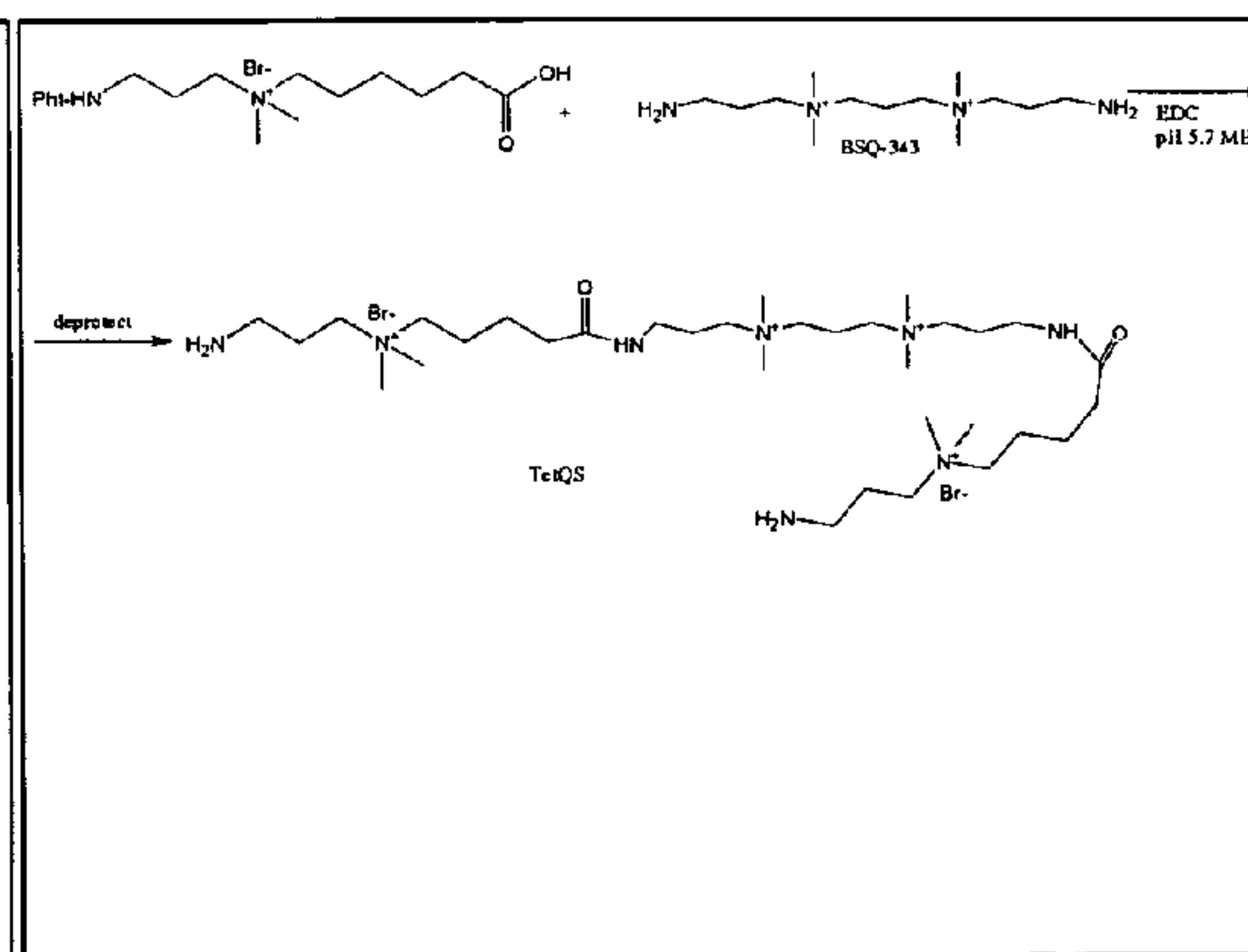
Scheme 4 - TetQS linker
