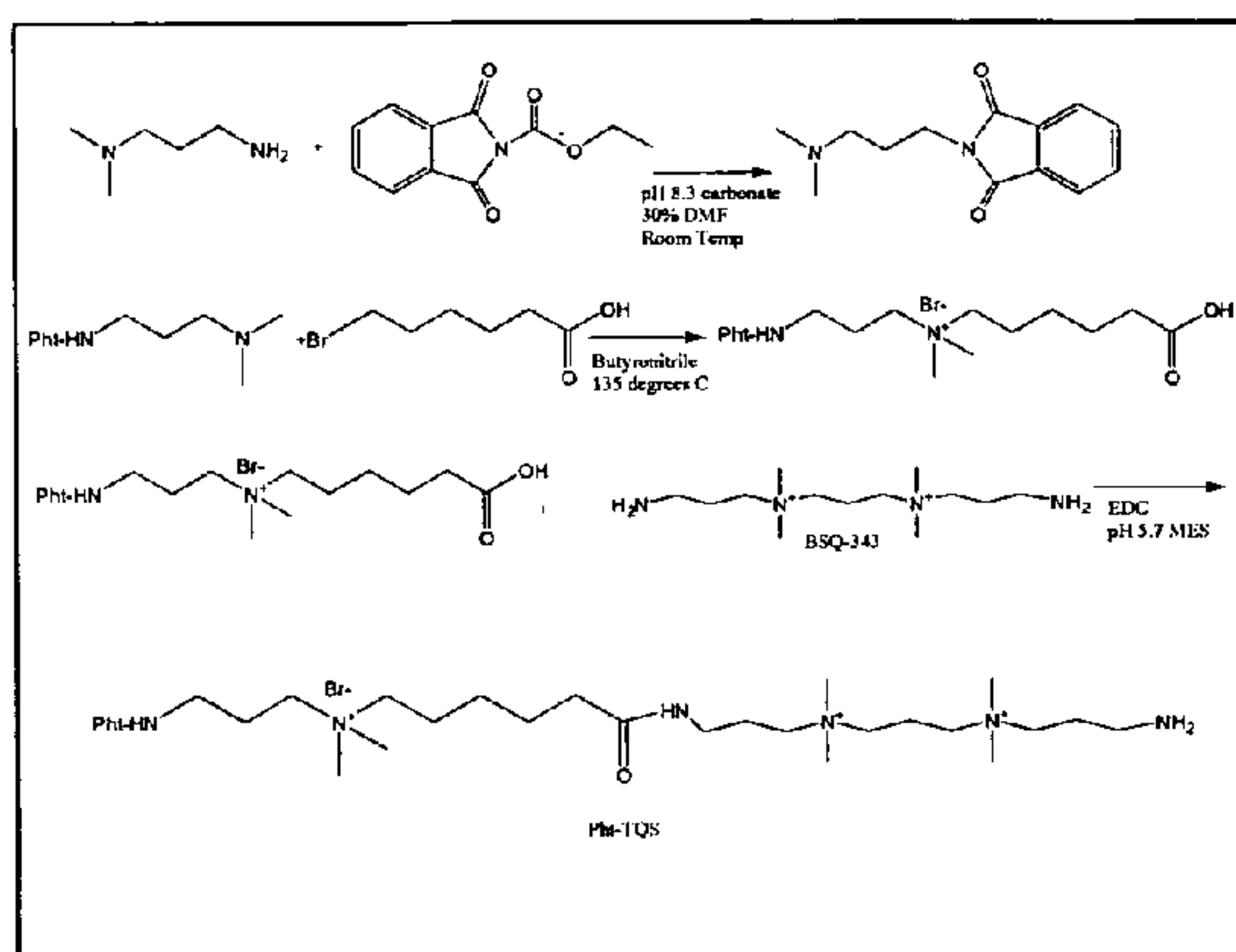
Scheme 3 - TQS linker
