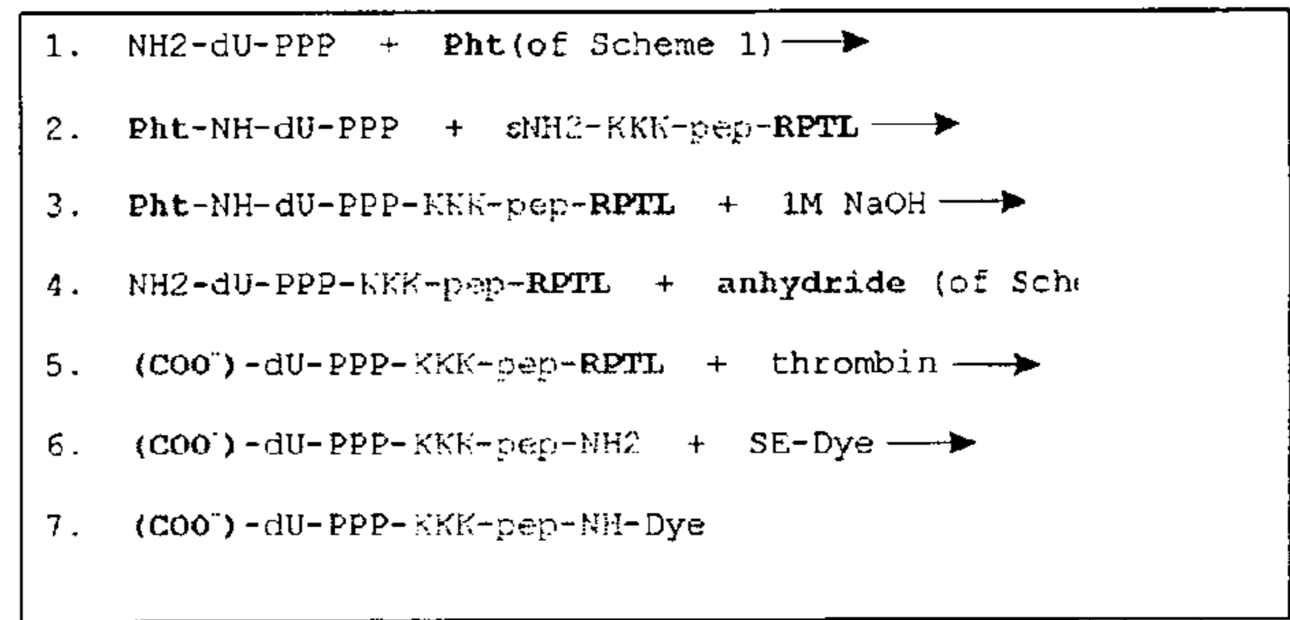
Scheme 10 - \gamma -dNTP With Carboxylated Base
