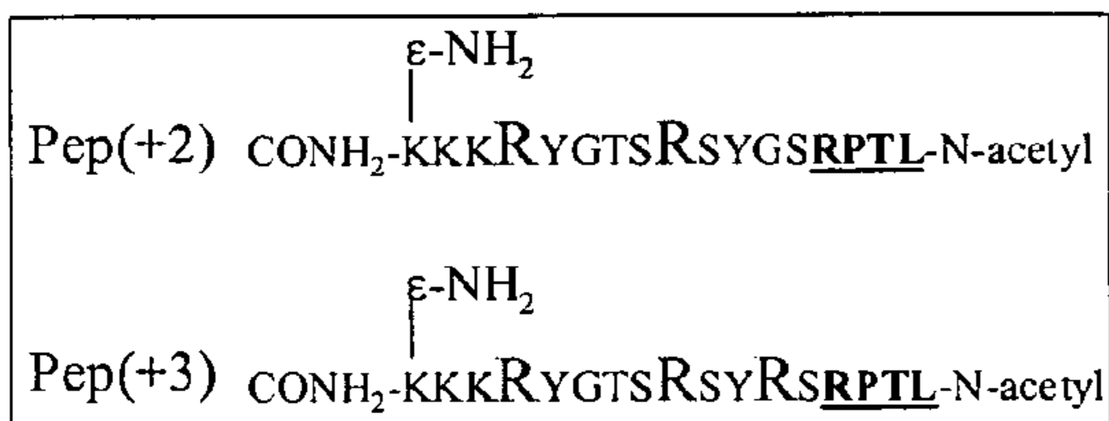
Scheme 7 - Peptide linkers (shown in C-to-N direction)
