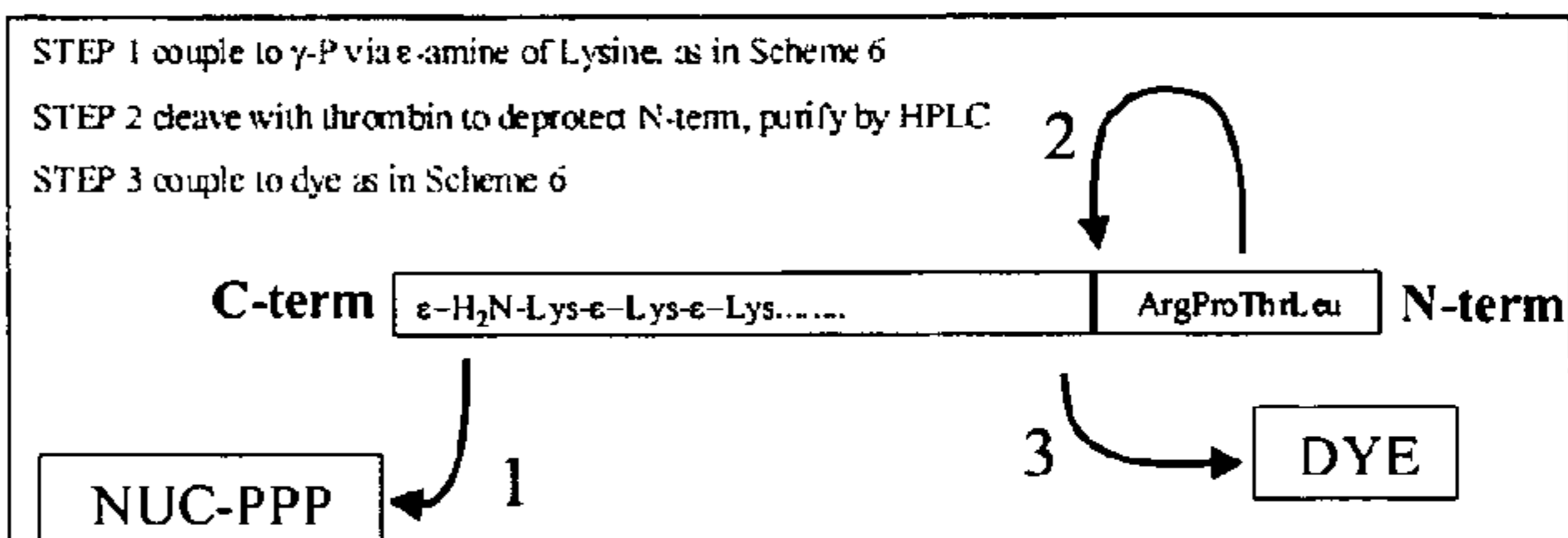
Scheme 8 - Peptide Deprotection By Thrombin Cleavage
