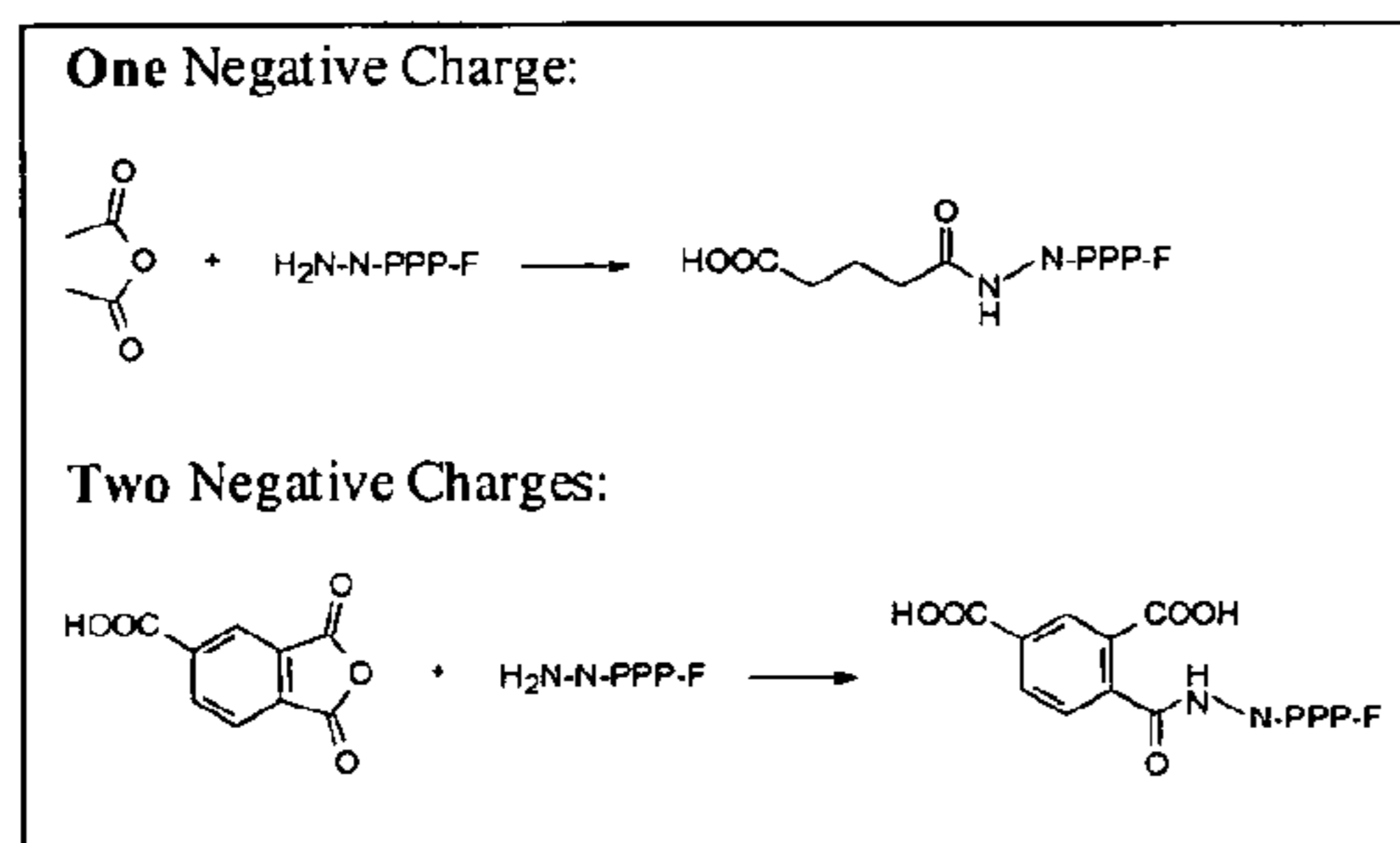
Scheme 9 - Add carboxylate to aminoallyl-dUTP
