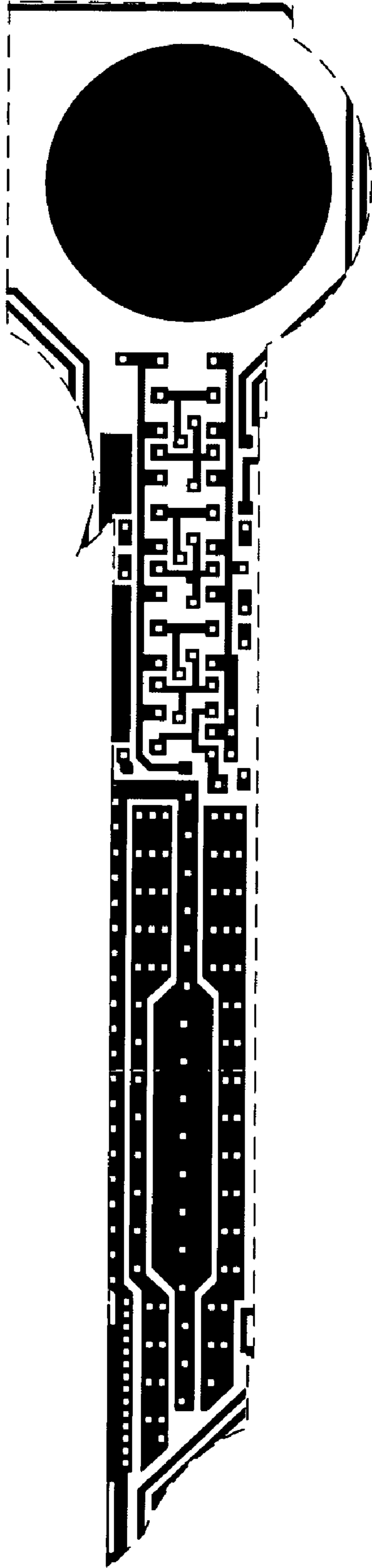
Metal 1 mask
