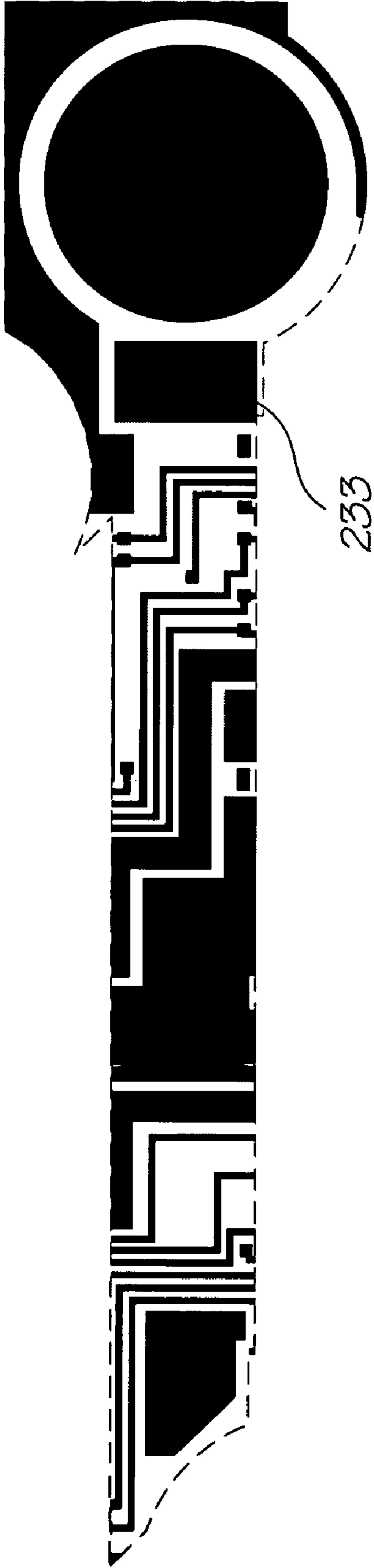
Metal 2 mask
