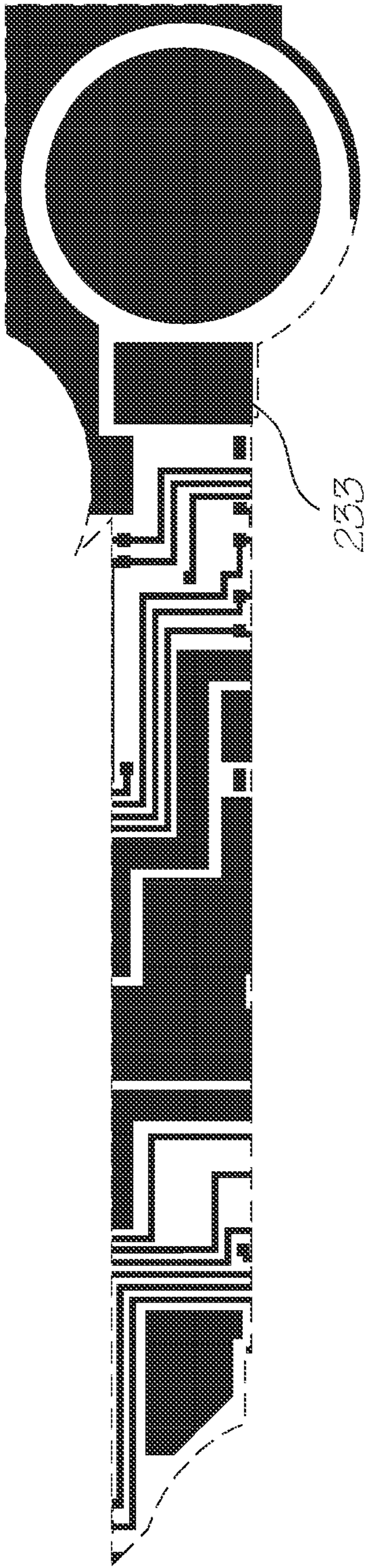
Metal 2 mask
