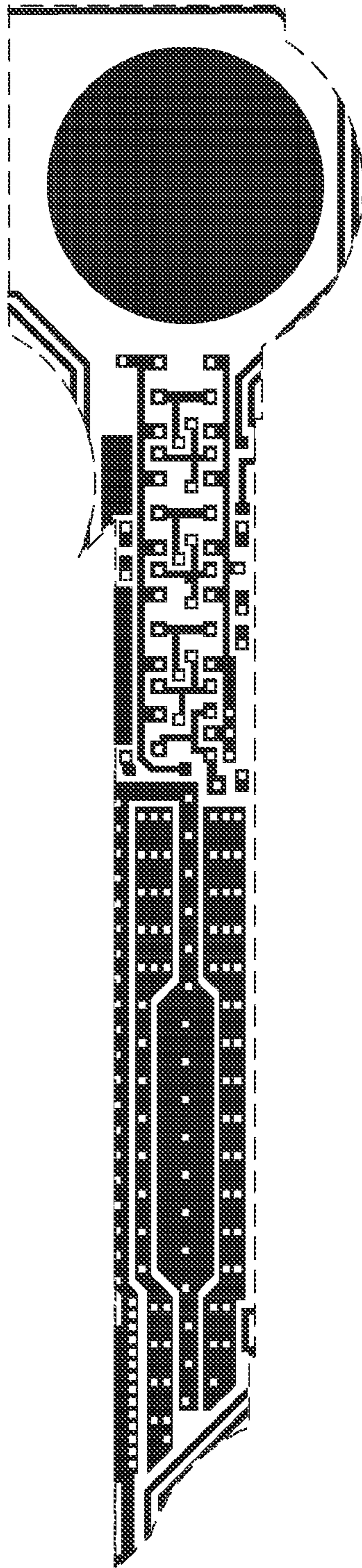
Metal 1 mask
