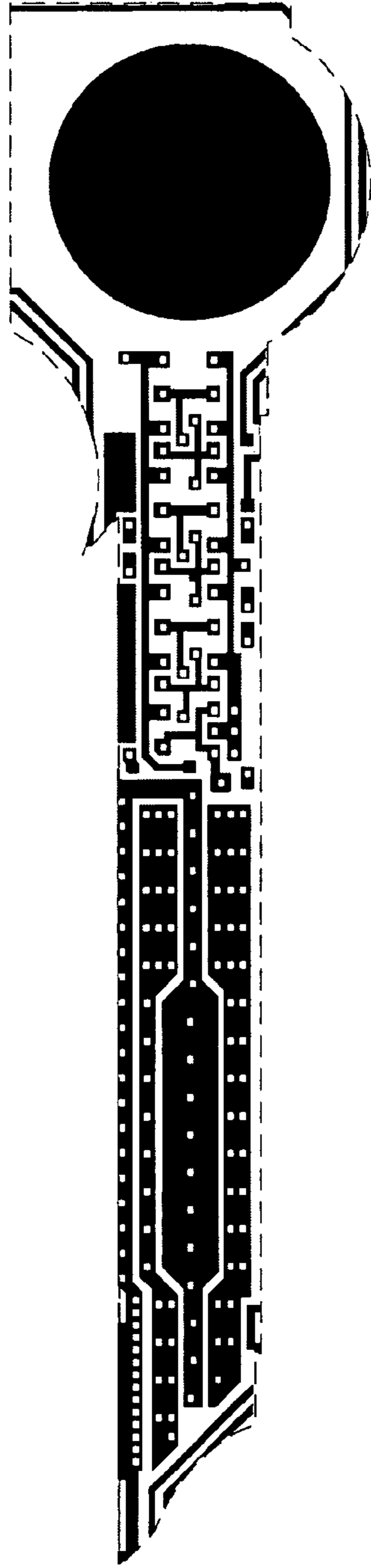
Metal 1 mask
