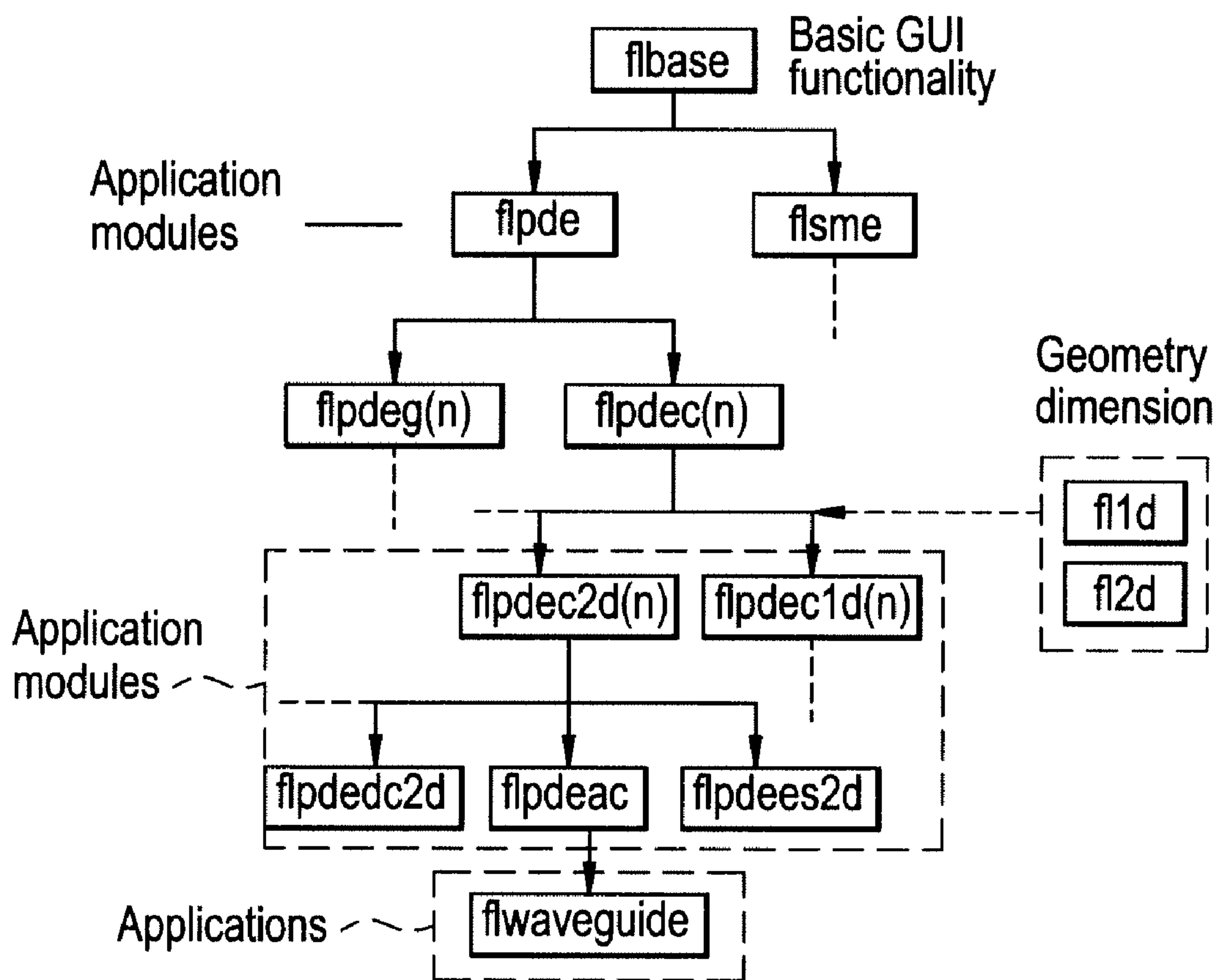
The Class Hierarchy of FEMLAB
