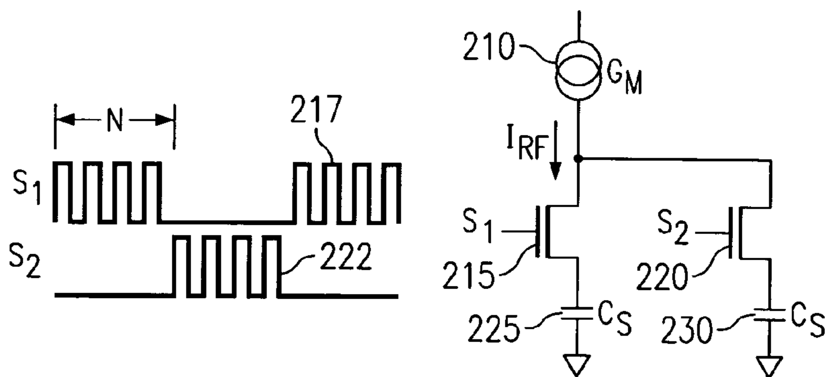
FIG. 2 (PRIOR ART)
