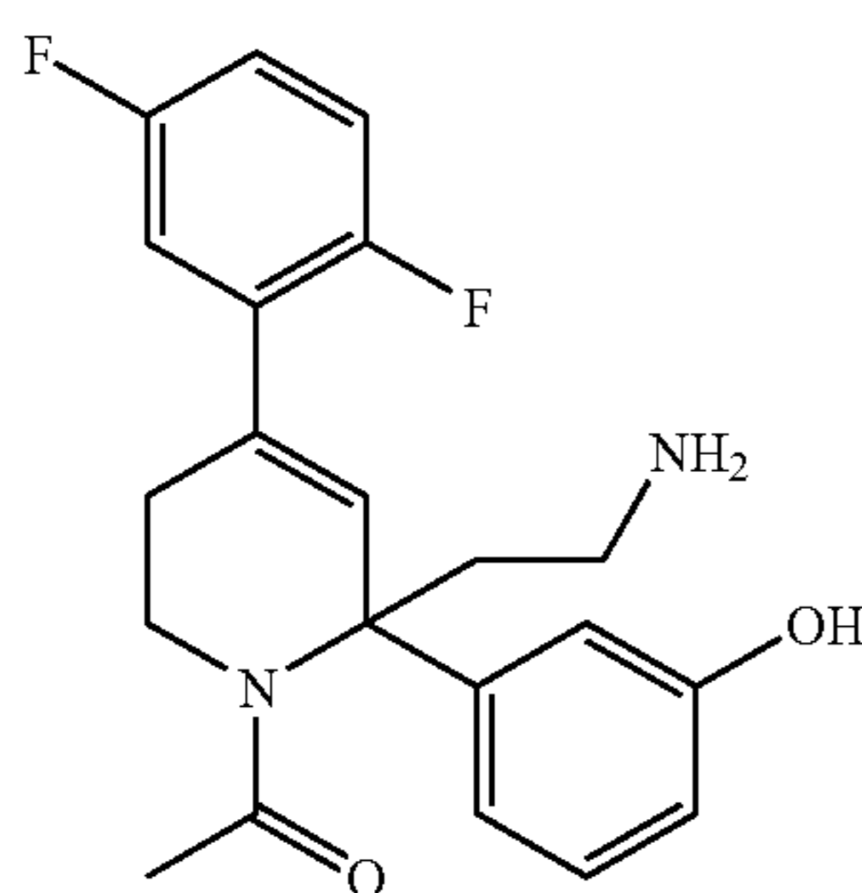
3-[1-acetyl-2-(2-aminoethyl)-4-(2,5- difluorophenyl)-1,2,5,6- tetrahydropyridin-2-yl]phenol
