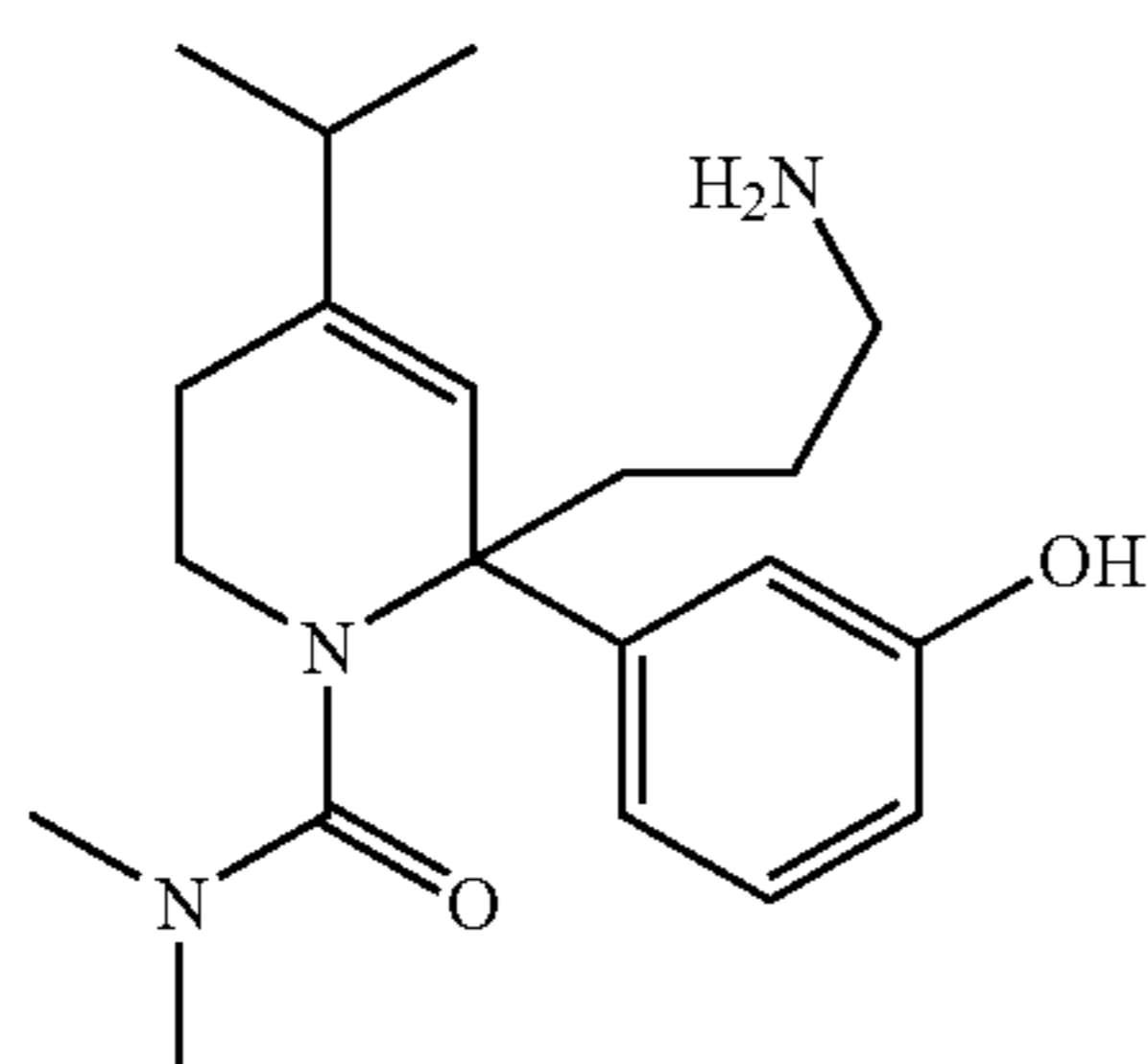
6-(3-aminopropyl)-6-(3-hydroxyphenyl)- 4-isopropyl-N,N-dimethyl-3,6- dihydropyridine-1(2H)-carboxamide
