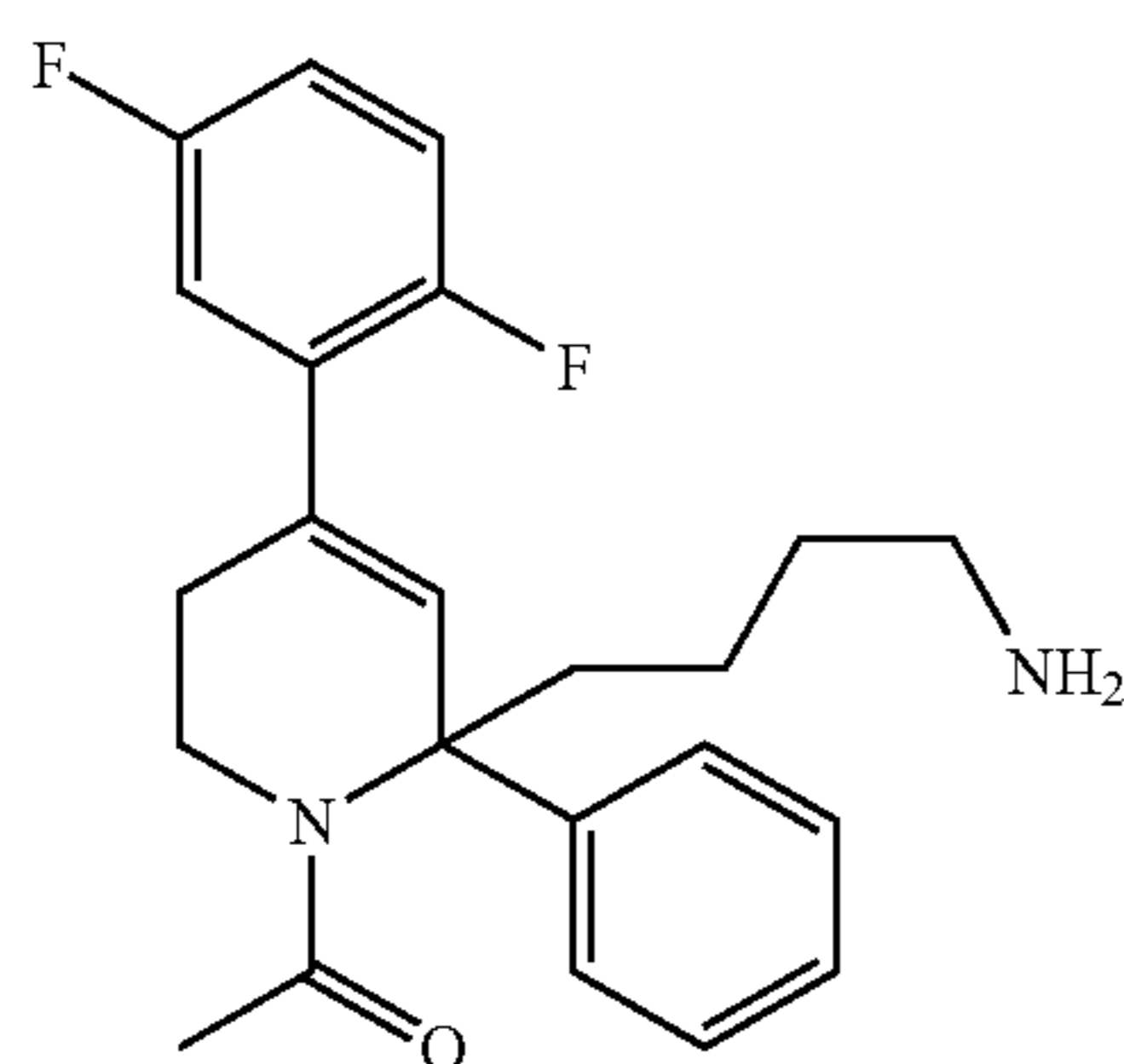
4-[1-acetyl-4-(2,5-difluorophenyl)-2- phenyl-1,2,5,6-tetrahydropyridin-2- yl]butan-1-amine
