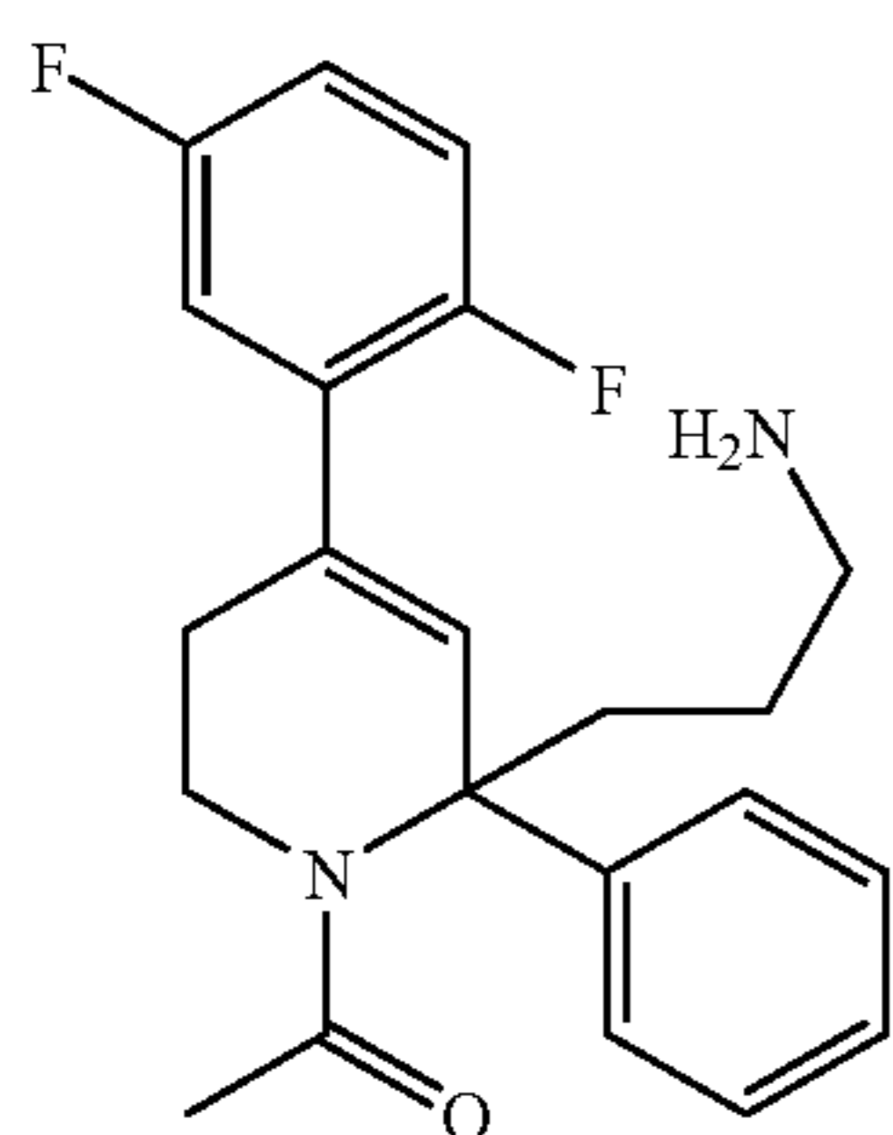
3-[1-acetyl-4-(2,5-difluorophenyl)-2- phenyl-1,2,5,6-tetrahydropyridin-2- yl]propan-1-amine
