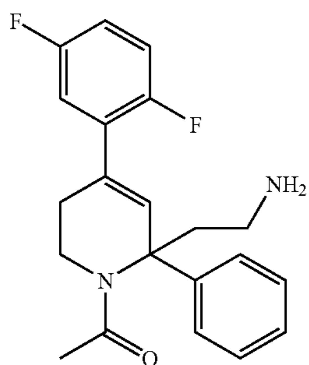
2-[1-acetyl-4-(2,5-difluorophenyl)-2- phenyl-1,2,5,6-tetrahydropyridin-2- yl]ethanamine
