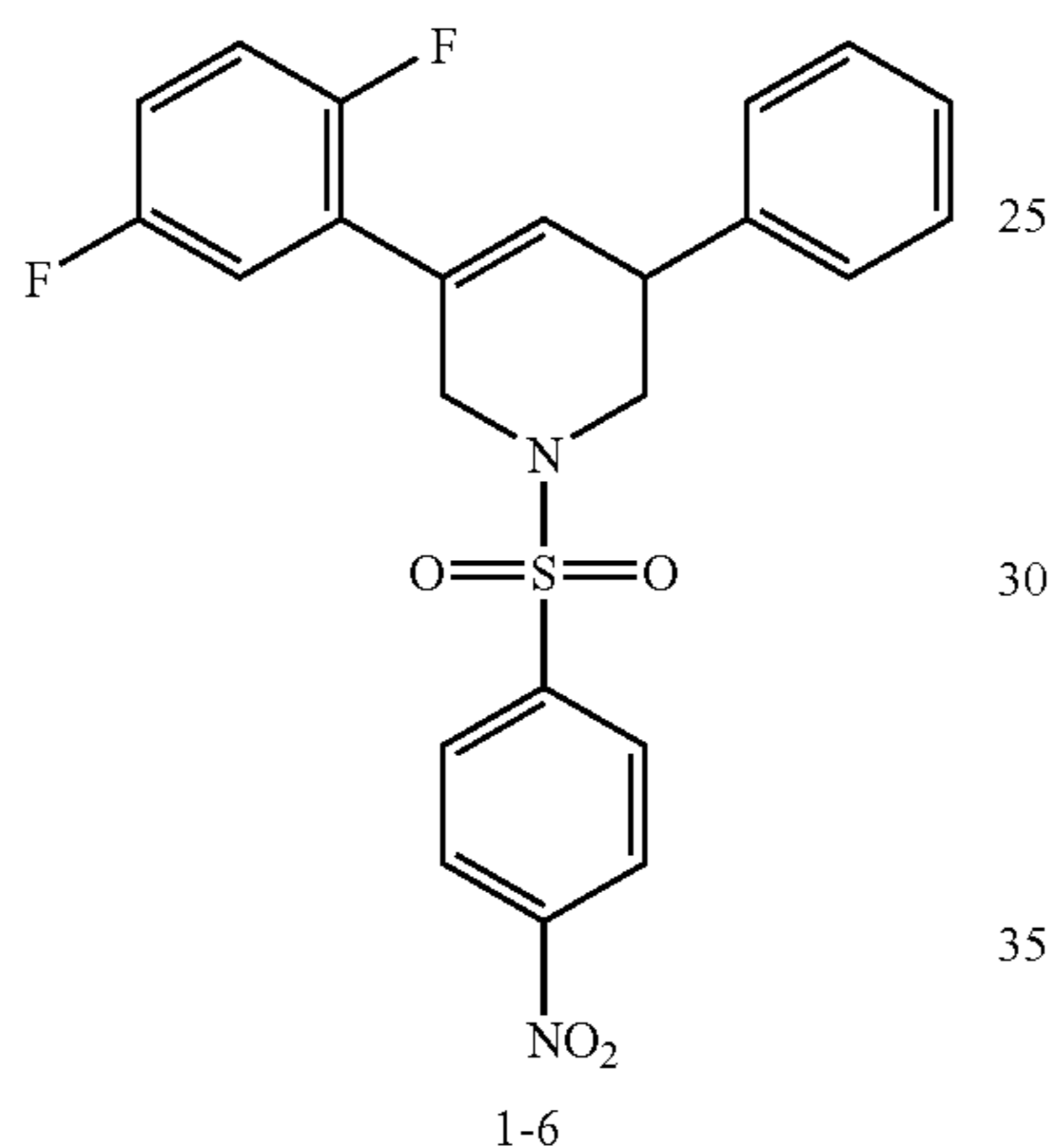
5-(2,5-difluorophenyl)-3-phenyl-1,2,3,6-tetrahydro- pyridine (1-7)
