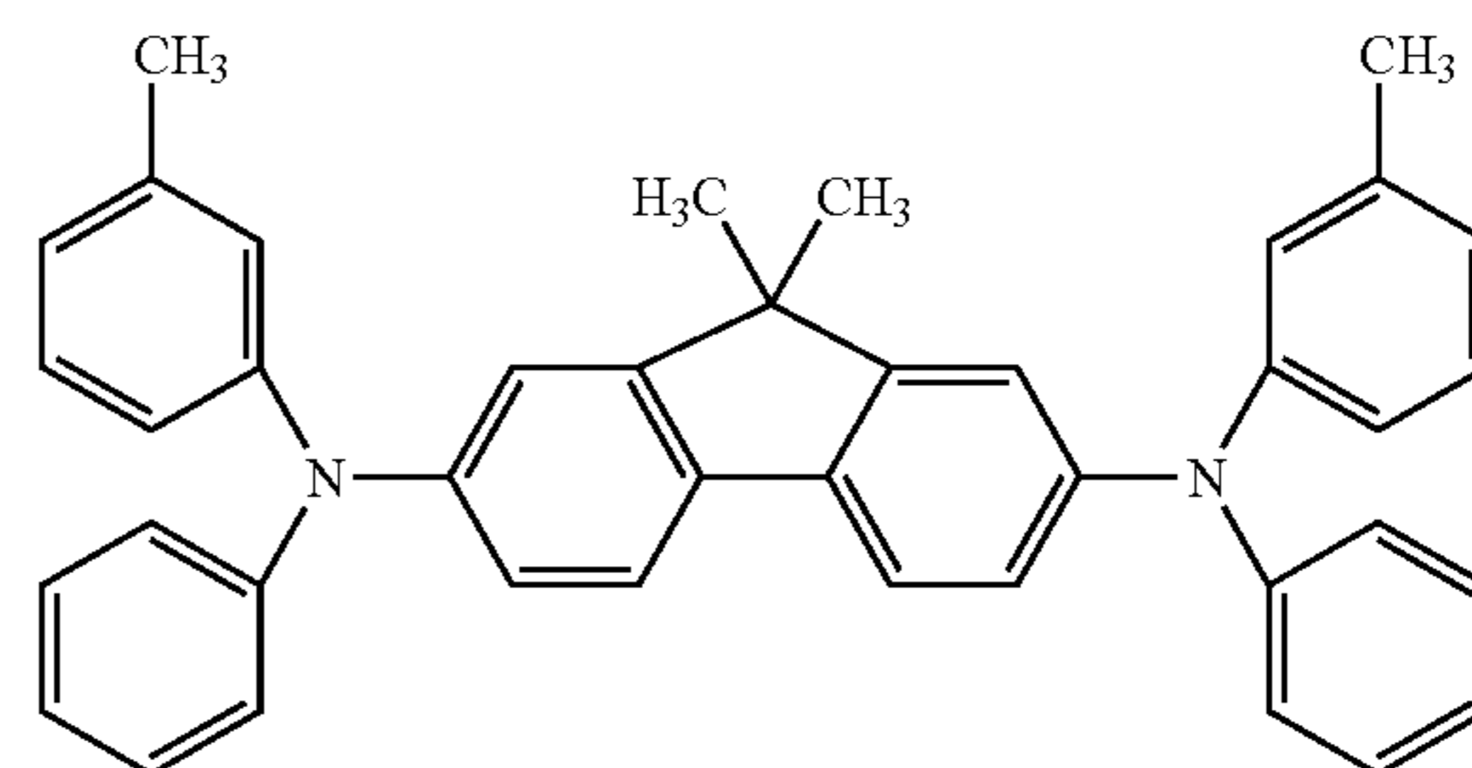
DTDPFL
