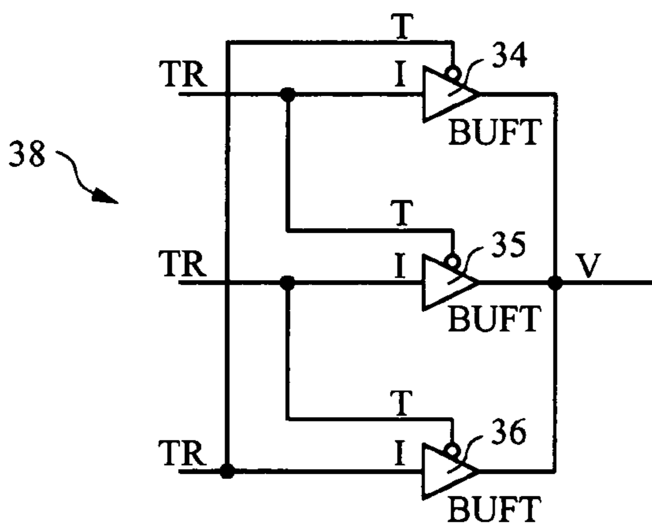
Voting circuit with BUFTs
